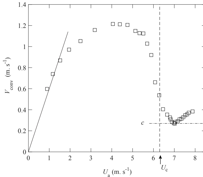
Figure 3.10: Convection velocity V_{\text{conv}} = \Lambda_x/\mathbb{T} , averaged over x \in [700, 1090] mm, as a function of the wind velocity U_a . The continuous line shows V_{\text{conv}} = 0.6U_a . The vertical dashed line indicates the onset of wave growth at U_c = 6.3 \text{ m.s}^{-1} , where the growth rate \beta transitions from zero to positive values. The horizontal dashed line shows the local phase velocity c = 0.27 \text{ m.s}^{-1} corresponding to the local wavelength \lambda = 44 \text{ mm} .
