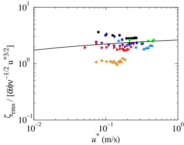
Figure 5.16: Evolution of \zeta_{rms}/\overline{\alpha}\phi\nu^{-1/2}u^{*3/2} relative to the friction velocity. The continuous line corresponds to 0.57f(Re_\tau) . \phi is computed using the values in table 5.1 with \Lambda = \lambda_c . For the symbols, refer to figure 5.12.
