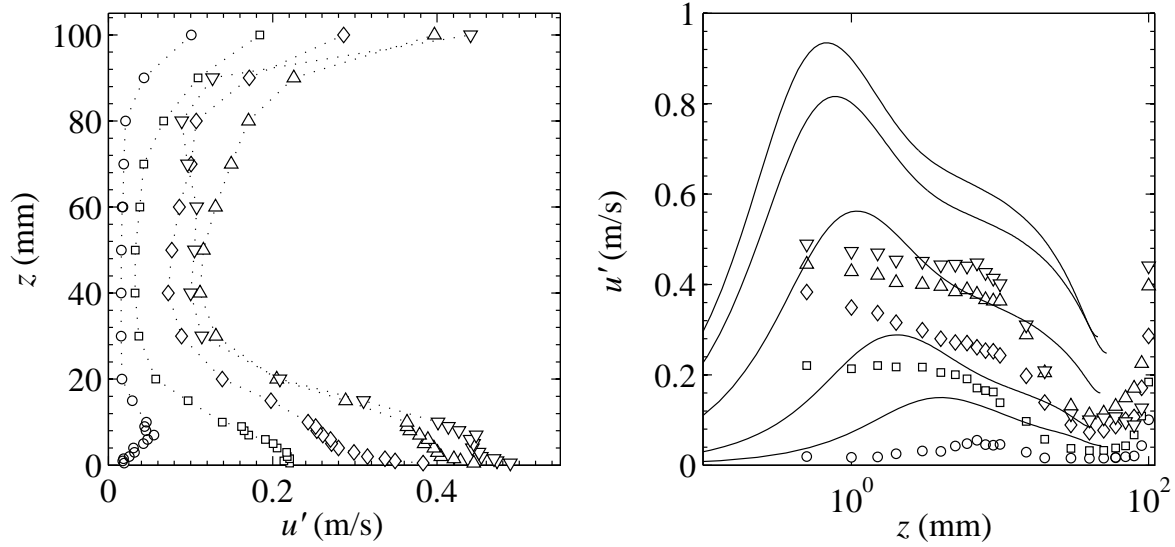
Figure 2.11: Root mean square of the velocity fluctuations at x = 500 mm at the center of the wind channel at wind speeds 1.0 \text{ m.s}^{-1} ( \circ ), 1.9 \text{ m.s}^{-1} ( \square ), 3.9 \text{ m.s}^{-1} ( \diamond ), 5.8 \text{ m.s}^{-1} ( \triangle ) and 6.6 \text{ m.s}^{-1} ( \nabla ). (Left) In linear coordinates. (Right) Compared in semilogarithmic coordinates with numerical simulations (continuous lines). Note that the axes are inverted between the two plots. The simulated profiles correspond from bottom to top to the increasing Re_{sim} in table 2.1 on page 40.
