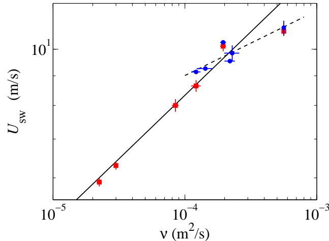
Figure 5.20: Evolution of the minimal wind velocity at which solitary waves are observed as a function of the kinematic viscosity of the liquid. This minimal velocity U_{sw} ( \bullet ) is compared to the threshold velocity U_c ( \blacksquare ) found previously. The dashed line corresponds to the power fit U_{sw} = K\nu^{0.11} with K = 25.2 SI, while the continuous line is the power fit associated to the threshold velocities U_c = a\nu^{0.22} , with a = 62.6 SI (see figure 5.10 on page 102).
