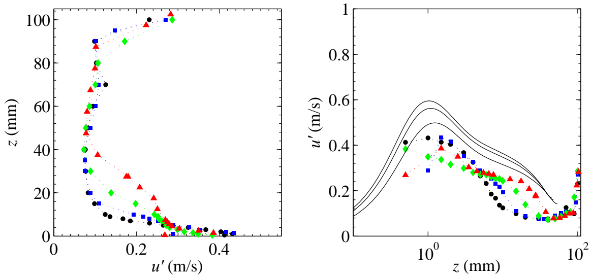
Figure 2.12: Root mean square of the velocity fluctuations at U_a = 3.9 \text{ m.s}^{-1} at the center of the wind channel at fetch -100 mm ( \bullet ), 20 mm ( \blacksquare ), 500 mm ( \blacklozenge ) and 1000 mm ( \blacktriangle ). (Left) In linear coordinates. (Right) Compared in semilogarithmic coordinates with numerical simulations (continuous lines). Note that the axes are inverted between the two plots. The simulated profiles correspond from bottom to top to the increasing fetch x in table 2.2 on page 40.
