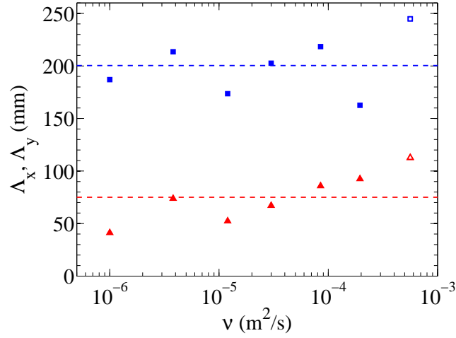
Figure 5.15: Correlation lengths \Lambda_x in the x direction (■) and \Lambda_y in the y direction (▲) as a function of the viscosity, in the wrinkles regime. For all but the highest viscosity, the correlation lengths are taken at a wind velocity U_a = 3.2 \pm 0.2 \text{ m.s}^{-1} . Because of the lower limit \zeta_{rms} = 0.65 \mu\text{m} , the data at the smallest available velocity in the wrinkles regime ( U_a = 4.5 \text{ m.s}^{-1} ) is used instead (open symbols). The two dotted line correspond to the average values \Lambda_x \simeq 200 \text{ mm} and \Lambda_y \simeq 75 \text{ mm} .
