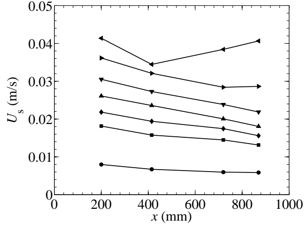
Figure 2.21: Evolution of surface drift U_s with fetch at various wind speeds: 3.0, 5.0, 5.5, 6.0, 6.5, 7.0 and 7.2 m.s -1 (from bottom to top plot).
