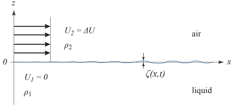
Figure 1.3: Sketch of the simplified velocity profile in the reference frame of the lower fluid used for the Kelvin-Helmholtz analysis.
