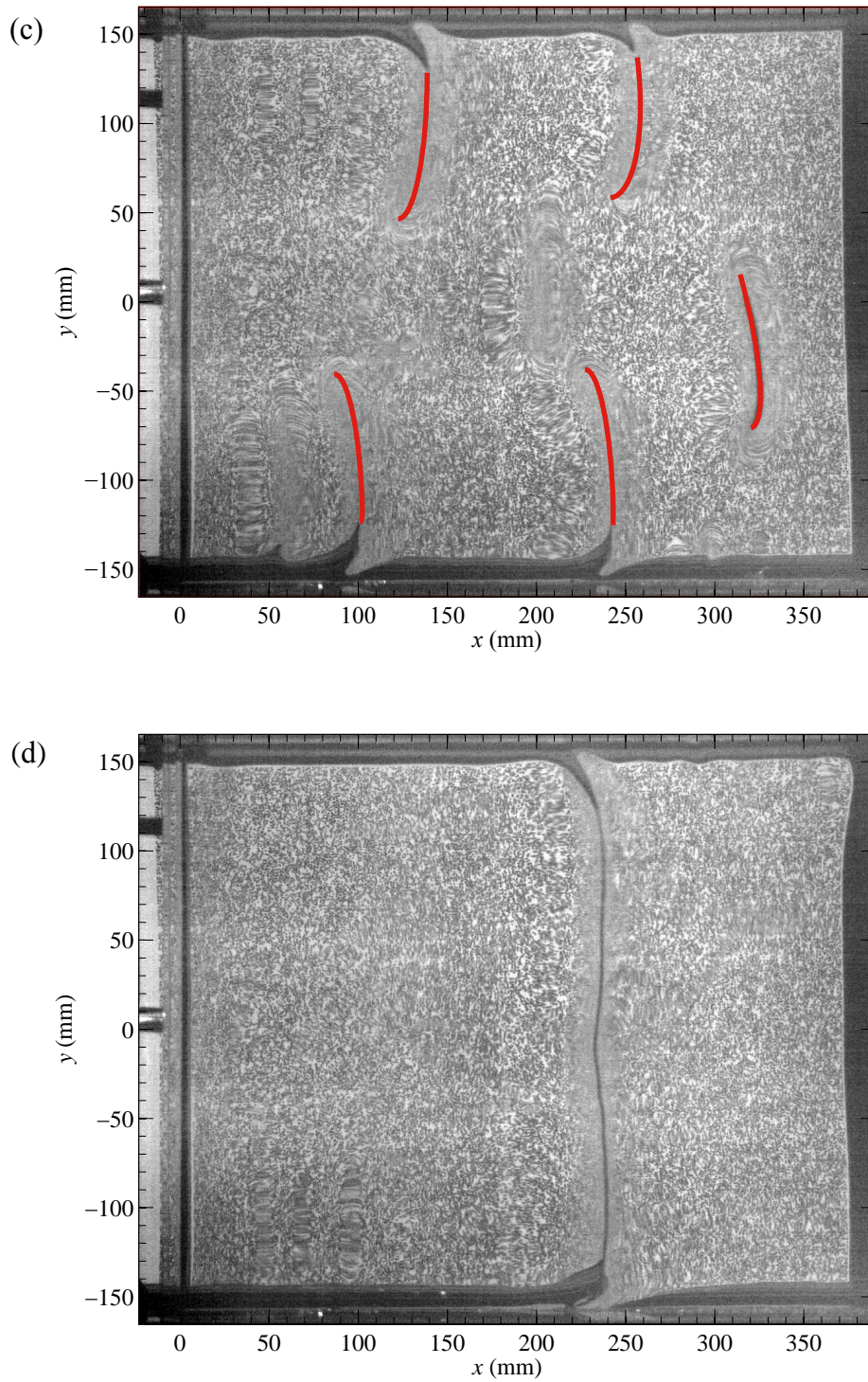
Figure 5.19 (continued). At U_a = 11.8 \text{ m}\cdot\text{s}^{-1} , (c) with multiple solitary waves, (d) with a fully transverse solitary wave.
