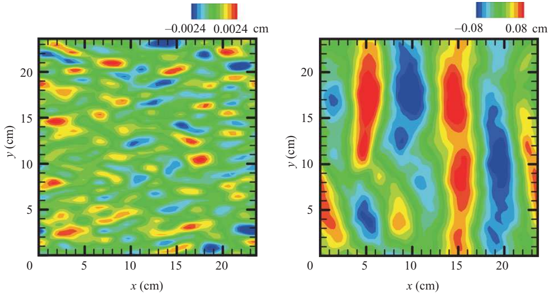
Figure 1.8: Snapshots of the instantaneous water surface elevation under the threshold, at time t = 2.6 s (left) and above the threshold, at t = 66 s (right). The wind is blowing in the direction of positive x . Adapted from [Lin et al., 2008].
