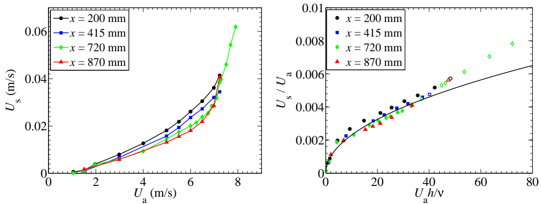
Figure 2.20: At fetches x = 200, 415, 720, 870 \text{ mm} . (Left) Evolution of the surface drift U_s with the wind speed U_a . (Right) Growth of the ratio U_s/U_a with Re = U_a h/\nu . Open symbols correspond to wind velocities above 7 \text{ m.s}^{-1} . The continuous line corresponds to Keulegan's law (Eq. (2.2.8)) with K = 7.3 \times 10^{-4} .
