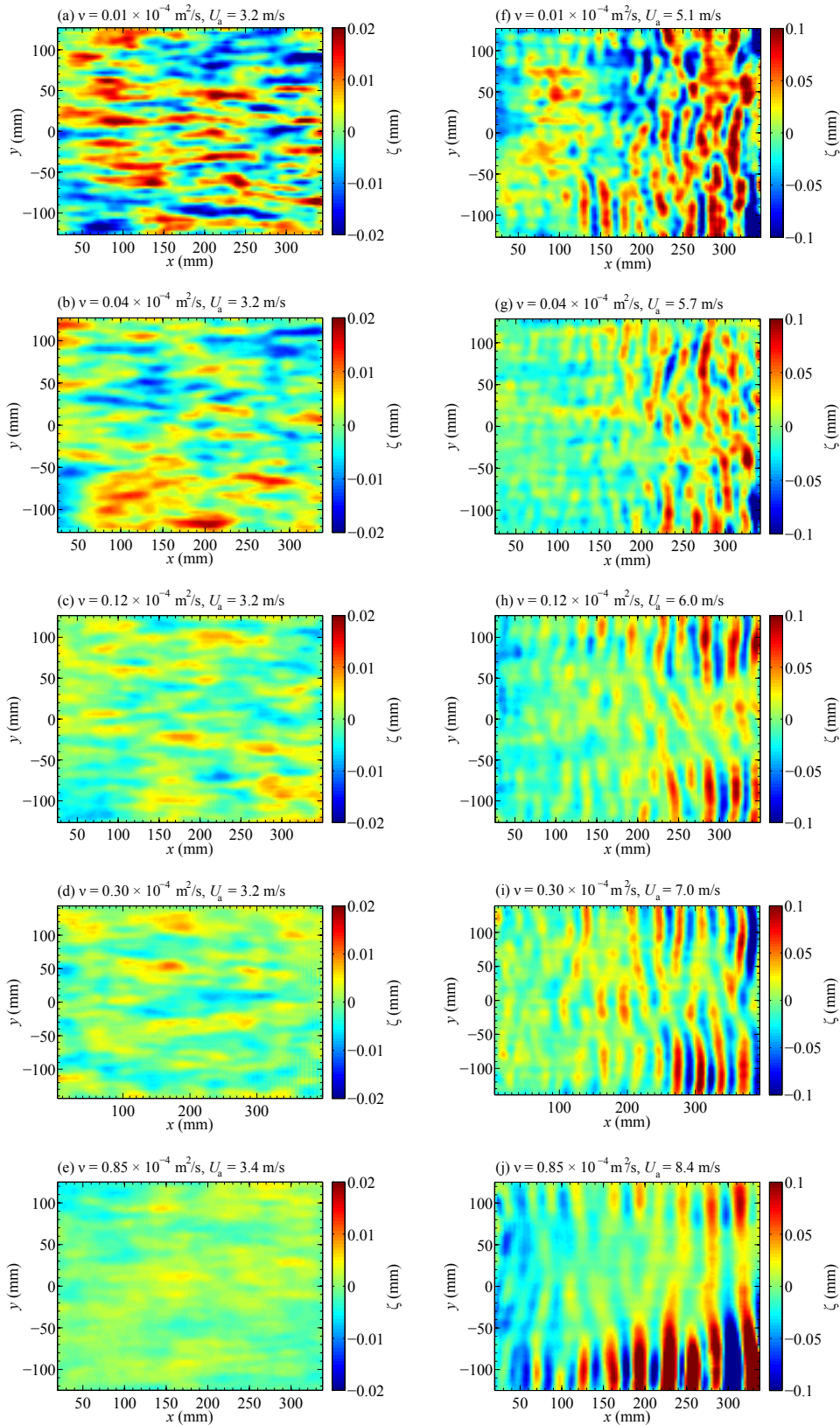
Figure 5.5: Instantaneous surface height \zeta(x, y) measured by FS-SS centered at fetch x = 190 \text{ mm} , for the increasing viscosities \nu = 0.01, 0.04, 0.12, 0.30 and 0.85 \times 10^{-4} \text{ m}^2 \cdot \text{s}^{-1} (for each pair of fields on a line, from top to bottom); (a-e) below the threshold, at a wind velocity chosen to be about 3.2 \text{ m} \cdot \text{s}^{-1} ; (f-j) above the threshold velocity. Note that the color map is the same within each column but varies from one column to the other.
