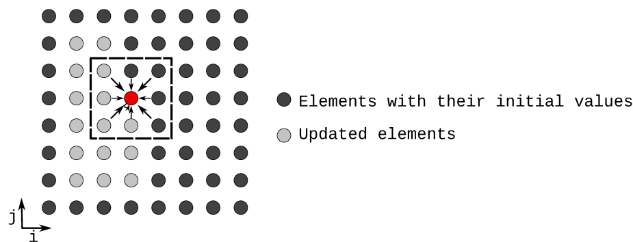
Figure 6.1 – Seidel Domain.
