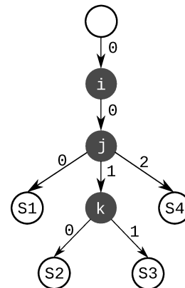
Figure 2.3 – Abstract Syntax Tree.
