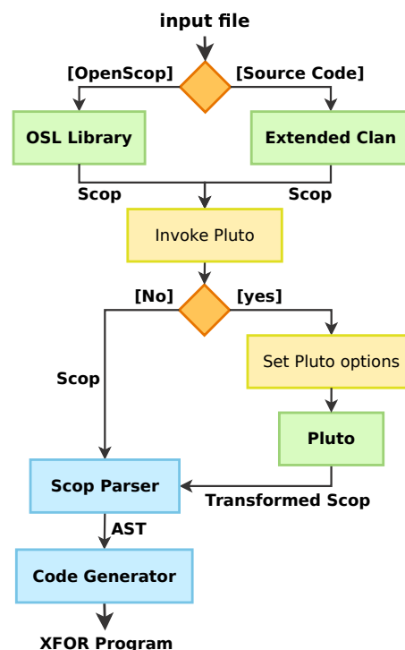
Figure 9.8 – XFORGEN Functioning.
