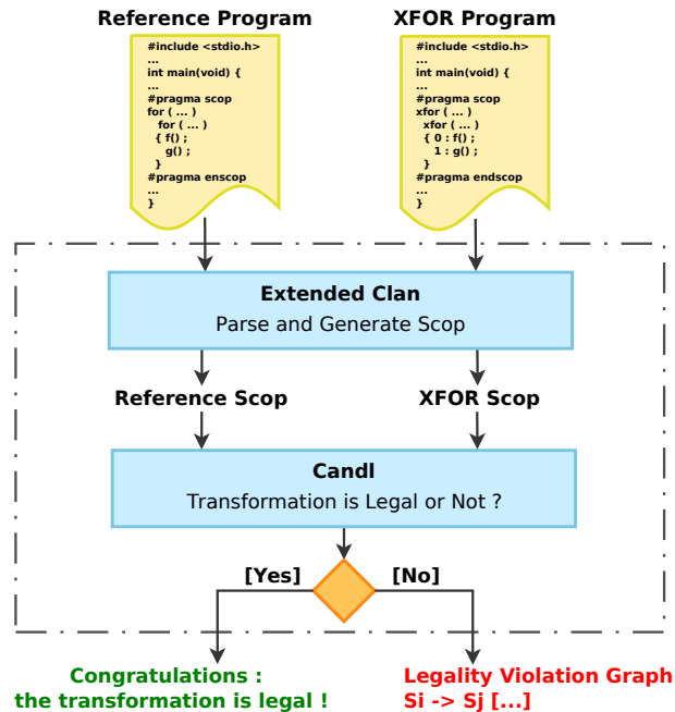
Figure 7.1 – XFORSCAN Architecture.
