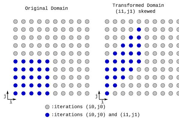
Figure 9.2 – Example 1: Skewing with XFOR.
