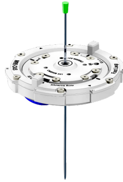
Figure B.1 – Second version of the needle MRE driver, based on a ring-shaped piezoelectric actuator.
