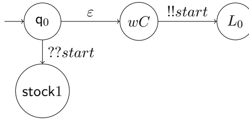
Figure 4.6: Initialization phase for REACH[ \mathcal{LC} ].
