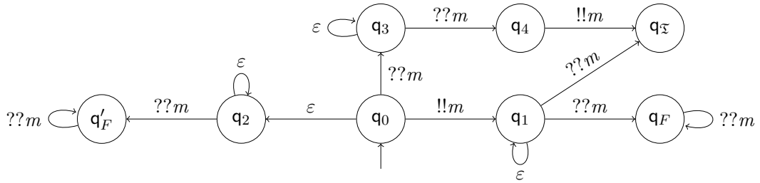
Figure 2.1: Example of a broadcast protocol.
