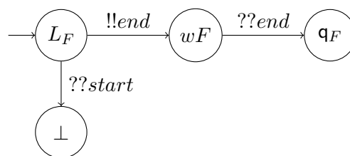
Figure 4.10: Ending phase for \text{REACH}[\mathcal{LC}] .
