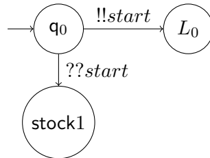
Figure 4.11: Initialization phase for \text{SYNCH}[\mathcal{LC}] .
