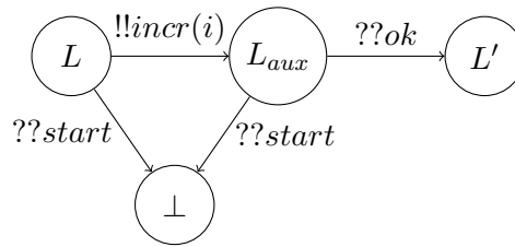
Figure 4.7: Encoding an increment L : c_i := c_i + 1 ; goto L' .
