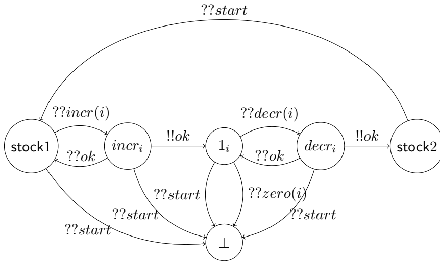
Figure 4.9: Encoding counter c_i .
