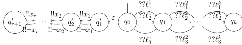
Figure 3.3: Encoding a 3-SAT formula into a broadcast protocol.
