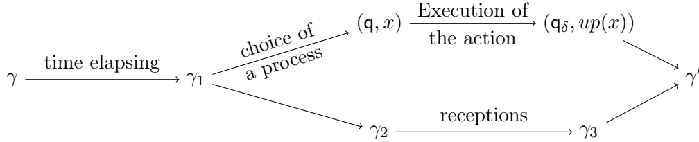
Figure 2.3: Graphical representation of a non-deterministic transition.
