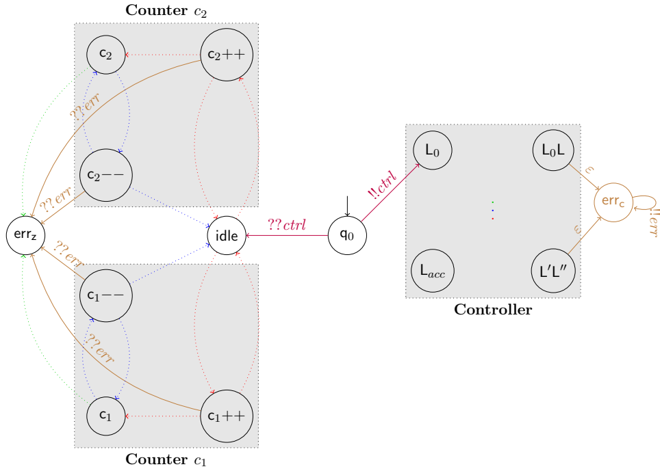
Figure 3.9: Reduction for REACH_{> 0}^\forall(\mathcal{C}) .
