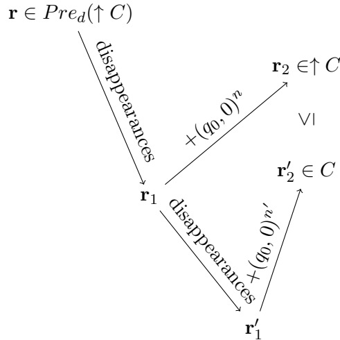
Figure 4.11: Graphical representation to show \text{Pre}_d(\uparrow C) \subseteq \text{Pre}_d(C) .
