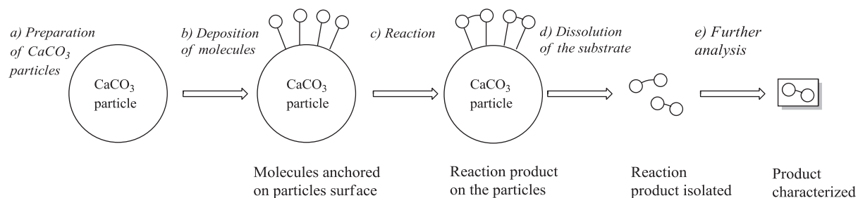
Figure 3.1 Coupling reactions on \text{CaCO}_3 particles.
