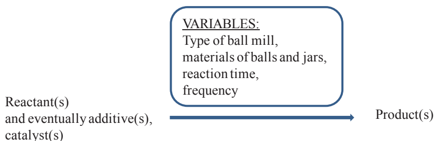
Figure 4.4 Variables in mechanochemistry reaction, readapted from the literature 1 .
