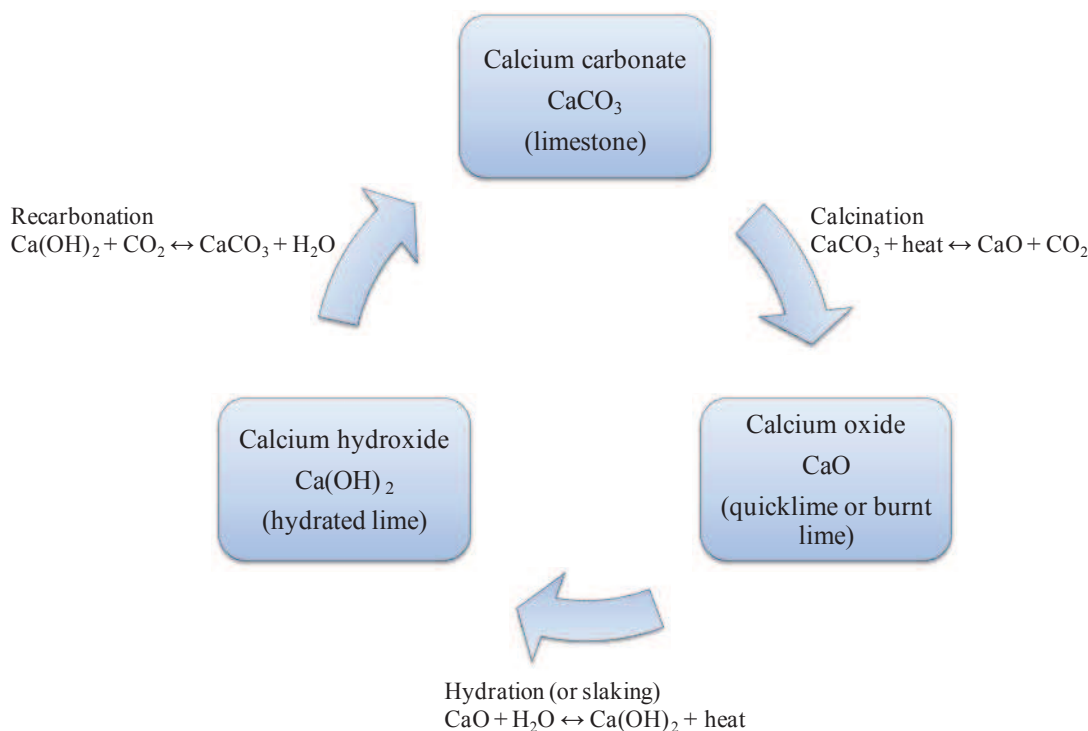
Figure 3.5 \text{CaCO}_3 life cycle.
