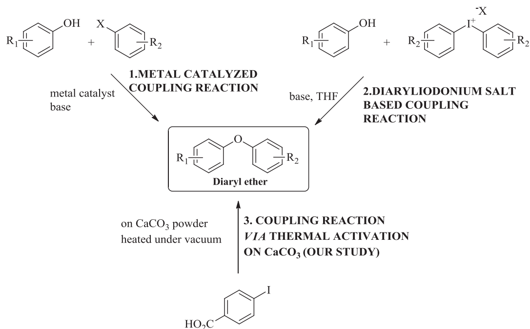
Figure 4.9 Principal synthetic strategies in order to obtain diaryl ethers.
