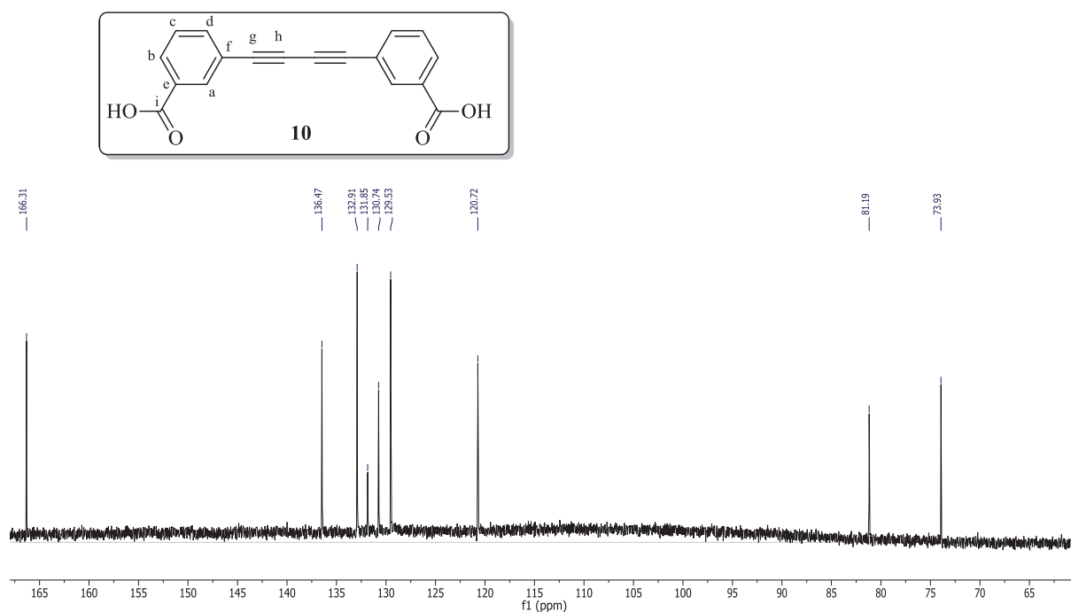
Figure 2.18 ^{13}\text{C} NMR of molecule 10 .
