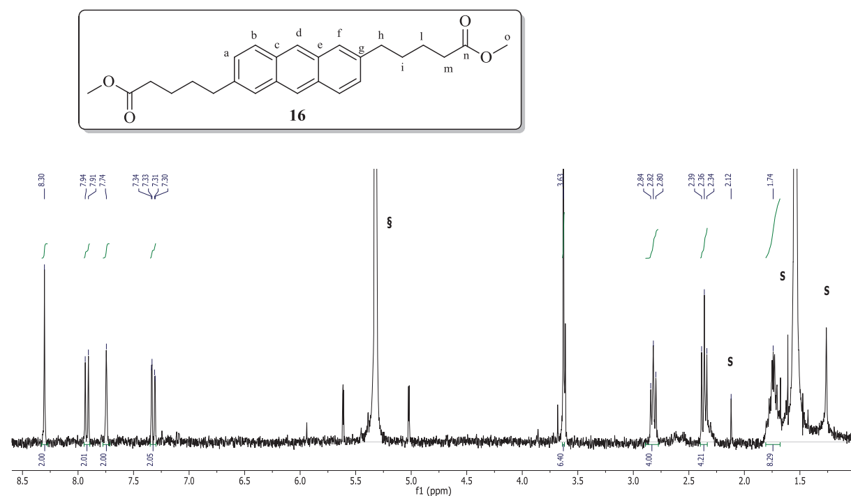
Figure 2.40 ^1\text{H} spectra of molecule 16 . Signals marked with “S” at 2.12, 1.52 and 1.26 ppm are acetone, water and grease respectively; signal marked with “§” is \text{CD}_2\text{Cl}_2 .
