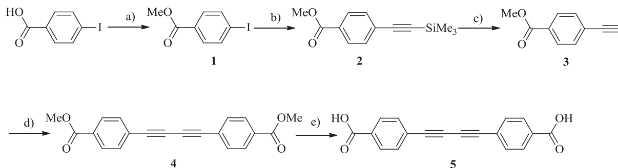
Figure 2.4 Synthesis of target molecule 5 . Conditions: a) MeOH, reflux, overnight, 81%; b) TMSA, \text{Pd}(\text{PPh}_3)_3\text{Cl}_2 (3%), CuI (5%), \text{Et}_3\text{N} , 25 °C, 2h, 94%; c) \text{K}_2\text{CO}_3 , MeOH/ \text{CH}_2\text{Cl}_2 , 25 °C, 3h, 87% ; d) \text{I}_2 , \text{Pd}(\text{PPh}_3)_3\text{Cl}_2 (2.5%), CuI (6.3%), i\text{Pr}_2\text{NH} , 25 °C, 6h, 81%; e) LiOH, THF, 25 °C, 5 days, 61%.
