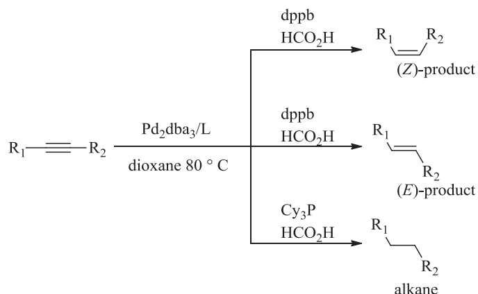
Figure 2.37 Hydrogenation of alkyne to alkenes or alkane with palladium catalyst and formic acid, readapted from the literature 45 .
