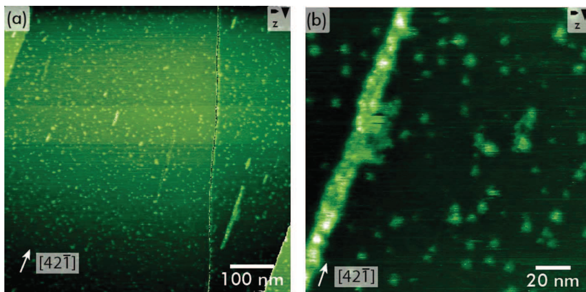
Figure 2.20 a-b) 3-ethynylbenzoic acid ( 10 ) dimer on CaCO 3 .
