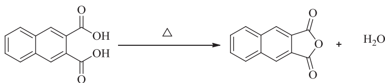
Figure 4.14 Dehydration of carboxylic acid.
