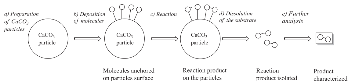
Figure 4.1 Coupling reactions on \text{CaCO}_3 particles.
