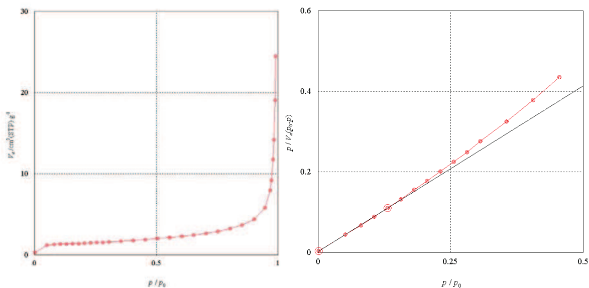
Figure 3.30 Adsorption isotherm and BET plot of sample 5 (SP at 500 °C) after the heating treatment.
