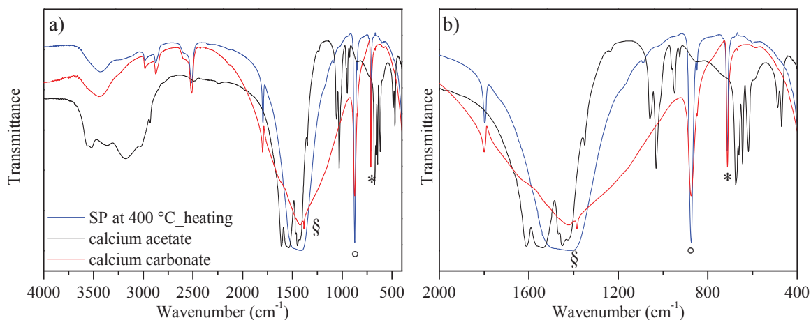
Figure 3.22 a) FTIR of sample 3 (SP at 400 °C) after heating treatment, calcium acetate and calcium carbonate between 4000 and 400\text{ cm}^{-1} . b) FTIR of sample 3 (SP at 400 °C) after heating treatment, calcium acetate and calcium carbonate between 2000 and 400\text{ cm}^{-1} . The main peaks corresponding to calcite are marked with symbols (§, ° and *), as reported in Table 3.7. The legend is the same, for clarity reason is not reported in the second graph.
