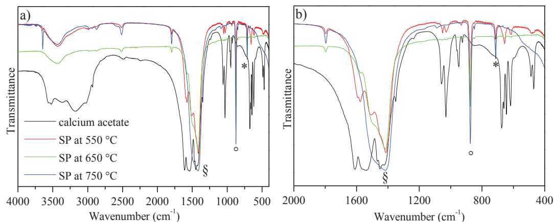
Figure 3.14 a) FTIR of samples 6-7-8 (SP at 550-650-750 °C) and calcium acetate, between 4000 and 400 \text{cm}^{-1} . b) FTIR of samples 6-7-8 (SP at 550-650-750 °C) and calcium acetate, between 2000 and 400 \text{cm}^{-1} . The peaks corresponding to calcite are marked with symbols (§, ° and *), as reported in Table 3.7. The legend is the same, for clarity reason is not reported in the second graph.
