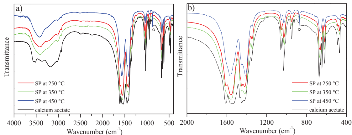
Figure 3.13 a) FTIR of samples 1-2-4 (SP at 250-350-450 °C) and calcium acetate, between 4000 and 400 \text{cm}^{-1} . b) FTIR of samples 1-2-4 (SP at 250-350-450 °C) and calcium acetate, between 2000 and 400 \text{cm}^{-1} . Only sample 4 (SP at 450 °C) shows a peak corresponding to calcite, marked with a symbol ( \circ ), as reported in Table 3.7.
