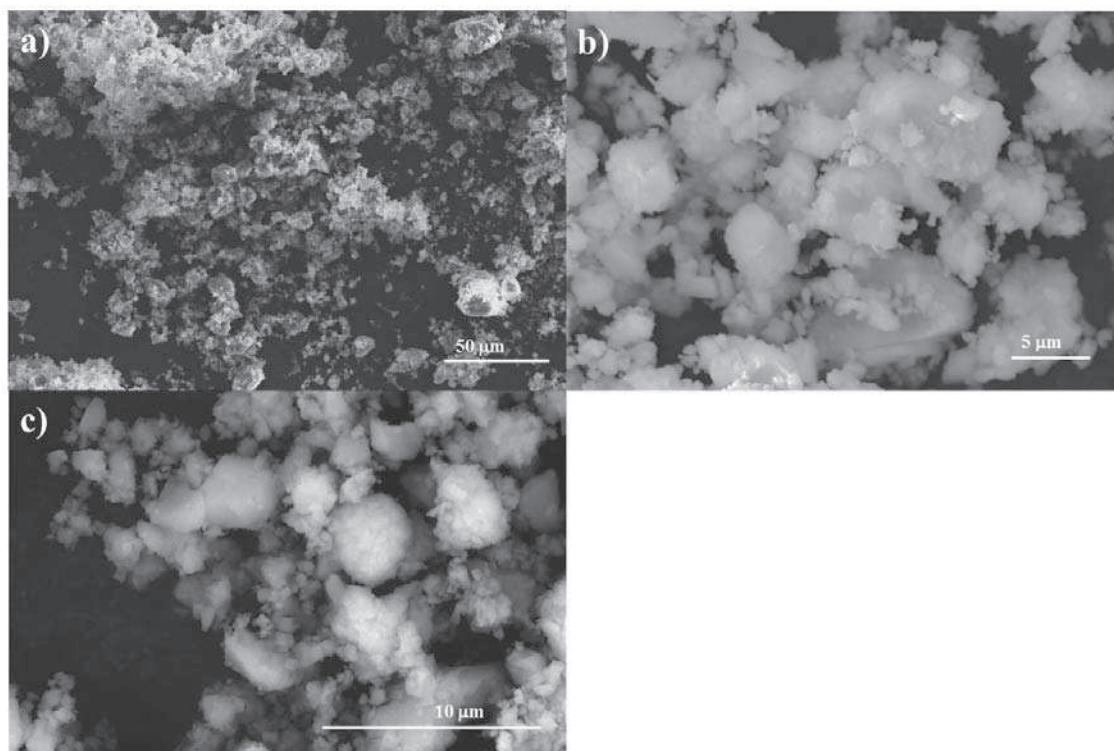
Figure 3.9 SEM images of commercial \text{CaCO}_3 after grinding.
