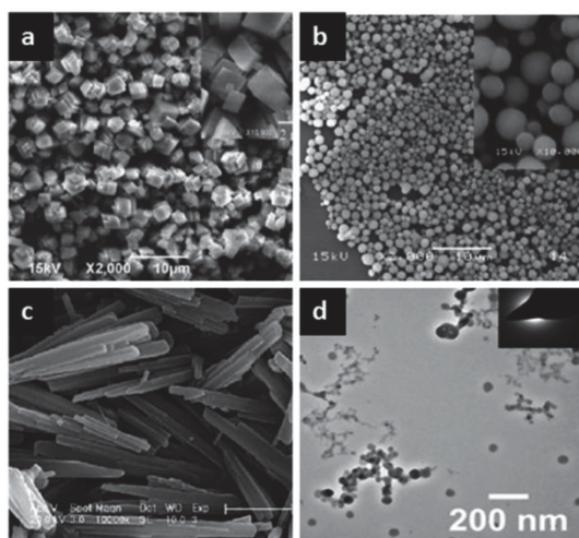
Figure 3.3 Different \text{CaCO}_3 polymorphs: a) calcite, rhombohedral; b) vaterite, spherical; c) aragonite, rod-like and d) ACC, seed. From ref. 2 .
