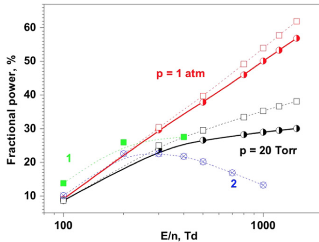
Figure 2.7: The fraction of the total electron power transferred into heat in dry air at 20 Torr and 1 atm as a function of the reduced electric field at which the energy was deposited in a high-voltage nanosecond discharge. The calculations were carried out for n_{ef} = 10^{15} \text{ cm}^{-3} (solid curves) and 10^{14} \text{ cm}^{-3} (dash curves). Curve 1 corresponds to calculations of Flitti and Pancheshnyi (2009) and curve 2 corresponds to the calculations of Popov (2001) assuming that 28% of the energy that was spent on the excitation of electronic \text{N}_2 and \text{O}_2 states was quickly transferred into gas heating. Reproduced from Aleksandrov et al. (2010).
