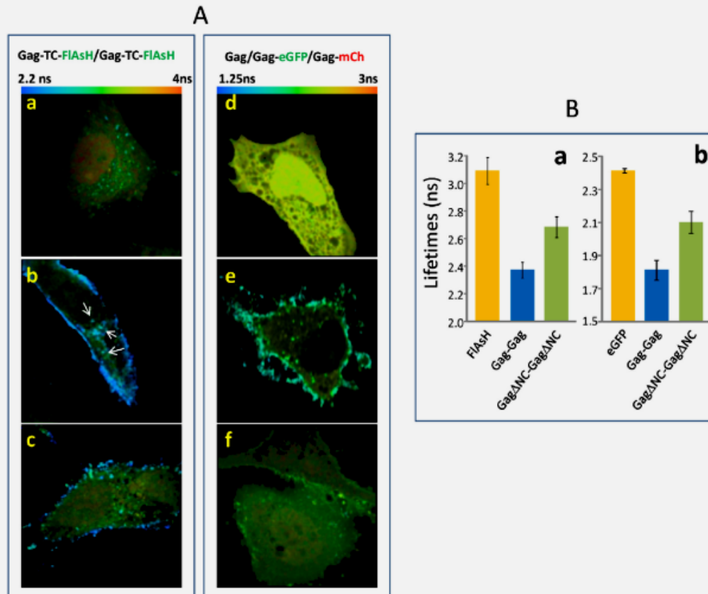
Fig. 5. HIV-1 Gag assembly imaged by FLIM. (A) FLIM images of cells expressing Gag-TC and labeled with -FIAsH (left) and cells expressing Gag-eGFP and Gag-mCherry (right). Since FIAsH and eGFP exhibit different lifetimes, the lifetime color scales on the top of panels a and d are different. (a) FIAsH chromophore alone, (b) Gag-TC-FIAsH, (c) GagΔNC-TC-FIAsH, (d) eGFP, (e) Gag/Gag-eGFP/Gag-mCherry and (f) GagΔNC/GagΔNC-eGFP/GagΔNC-mCherry. (B) Histograms representing the mean lifetime values of FIAsH (a) and eGFP (b) determined from measurements on at least 30 cells. FLIM measurements were performed using the time-correlated single-photon counting technique on a two-photon microscope (Azoulay et al., 2003; Clamme et al., 2003). Excitation at 900 nm was provided by a mode-locked titanium-sapphire laser (Tsunami, Spectra Physics). Photons were collected using a short-pass filter with a cut-off wavelength of 680 nm and a band-pass filter of 520 \pm 17 nm and were directed to a fiber-coupled APD (SPCM-AQR-14-FC, Perkin Elmer) connected to a SPC830 electronic card (Becker & Hickl, Germany). Data were analyzed using the SPCImage V2.8 software (Becker & Hickl, Germany).
