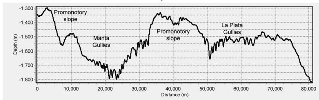
A-A' Bathymetric Profile
