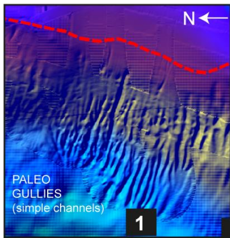
Figure 4.3: Map of Manta Peninsula-Plata area shows the bathymetry of the shelf, the slope, the trench and the eastern flank of the Carnegie Ridge.
