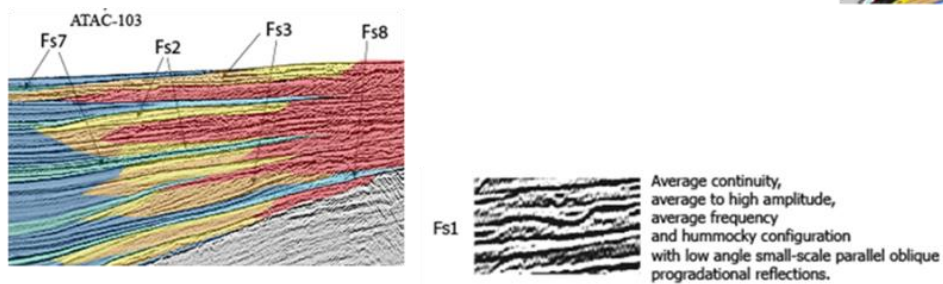
Figure 3.5: Steps followed for the seismic data interpretation.
