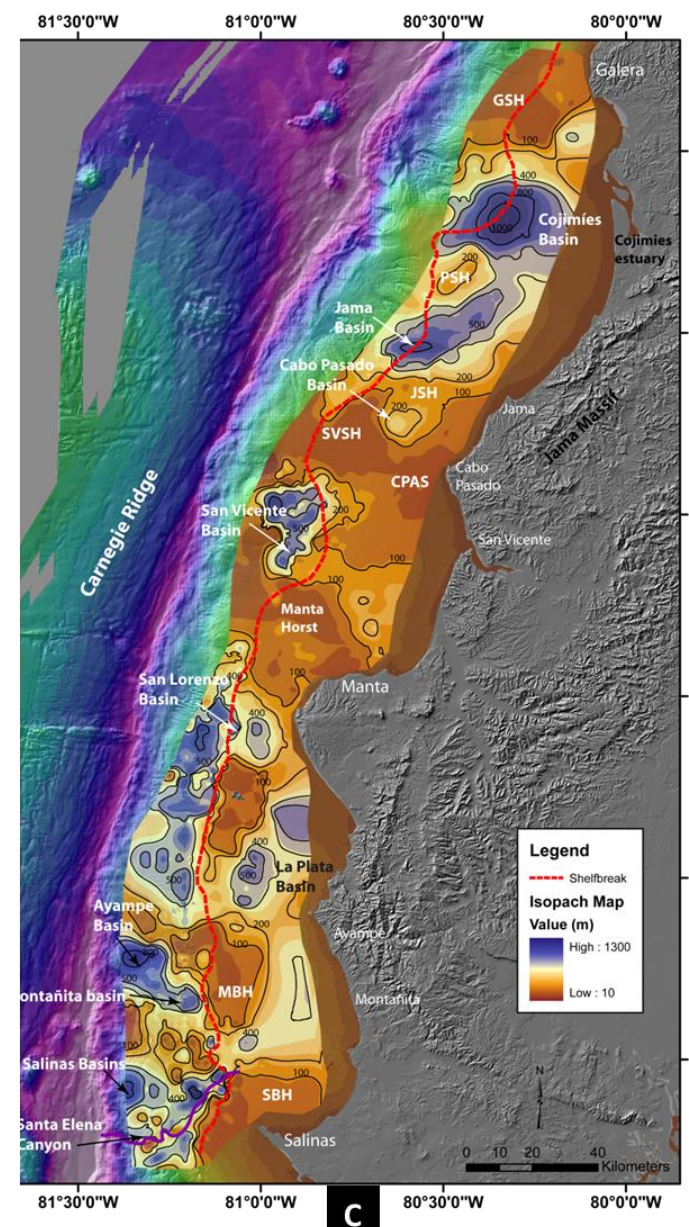
Figure 5.4: Isobath grid for the Pleistocene acoustic basement (left) and Isopach grid of the Pleistocene deposits along the central Ecuadorian margin.
