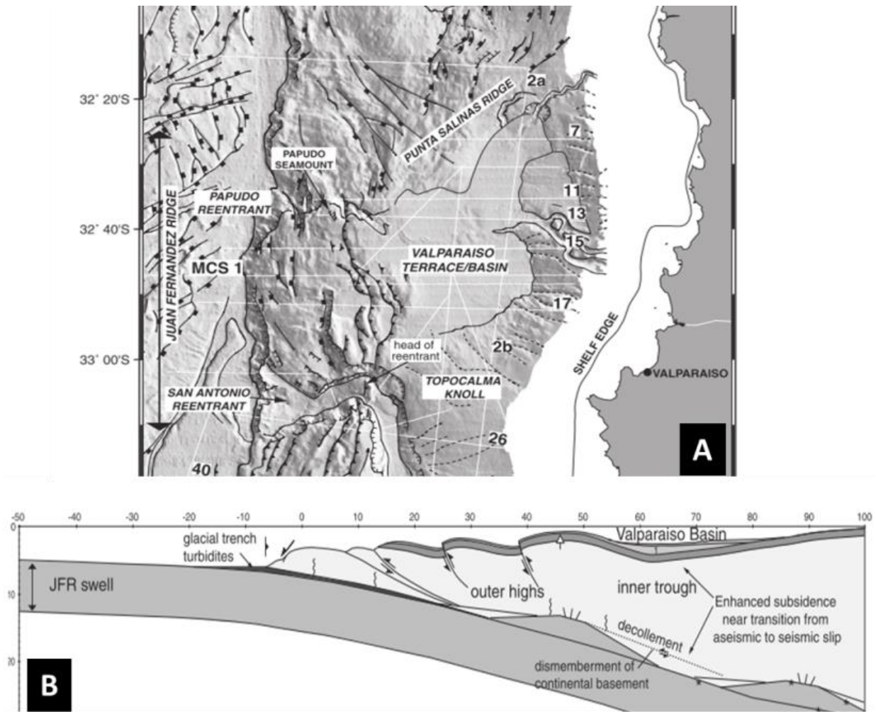
Figure 1.10: Structural interpretation made by Laursen et al., (2002) of seafloor around of the Valparaiso forearc basin. (A)The Valparaiso basin is located at the margin of the over-riding plate subducted by Juan Fernandez Ridge (JFR swell). (B)This image displays one of the evolution stages of this basin interpreted by the same authors, which suggests a continuous subduction of JFR (elongated asperity) and the eventual subduction of the seamounts (“punctual”asperities).
