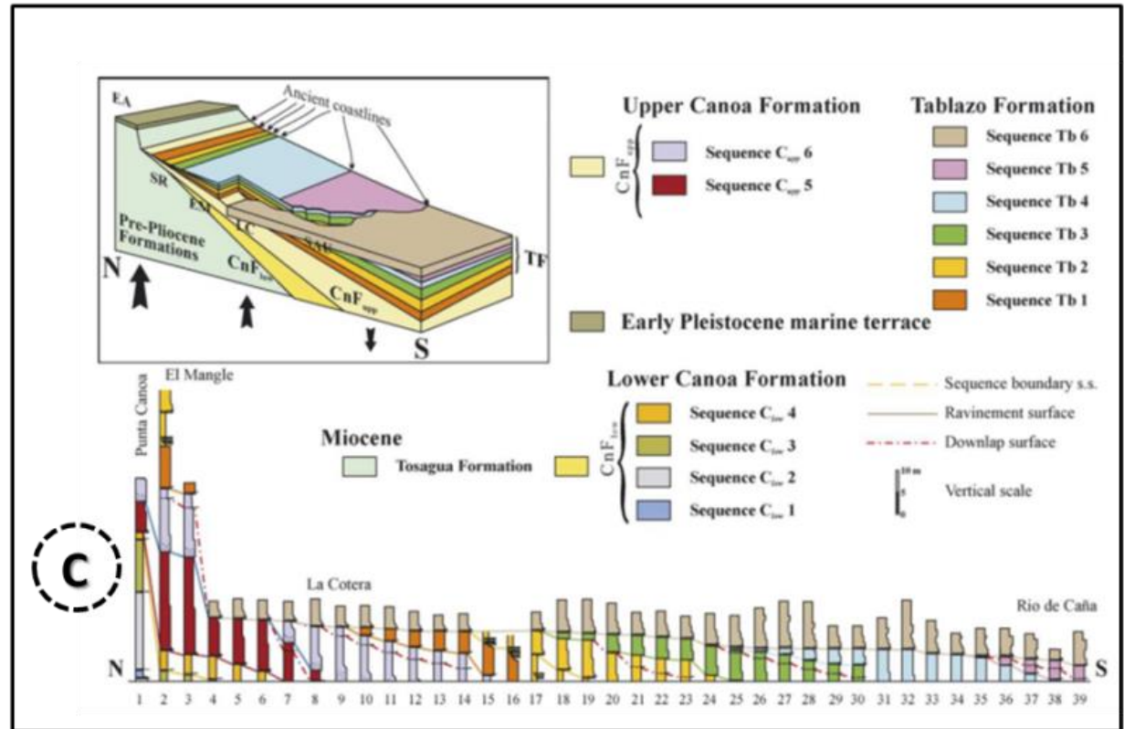
Figure 2.9: Jama and Canoa Formations. J) Stratigraphic section of the Punta Ballena Member of the Jama Formation (from Cantalamessa et al. 2005, see the location in Figure 2.8). C) Stacking pattern and block diagram of the depositional sequences of the Canoa and Tablazo Formations (from Cantalamessa and Di Celma, 2004; see the location in Figure 2.8).
