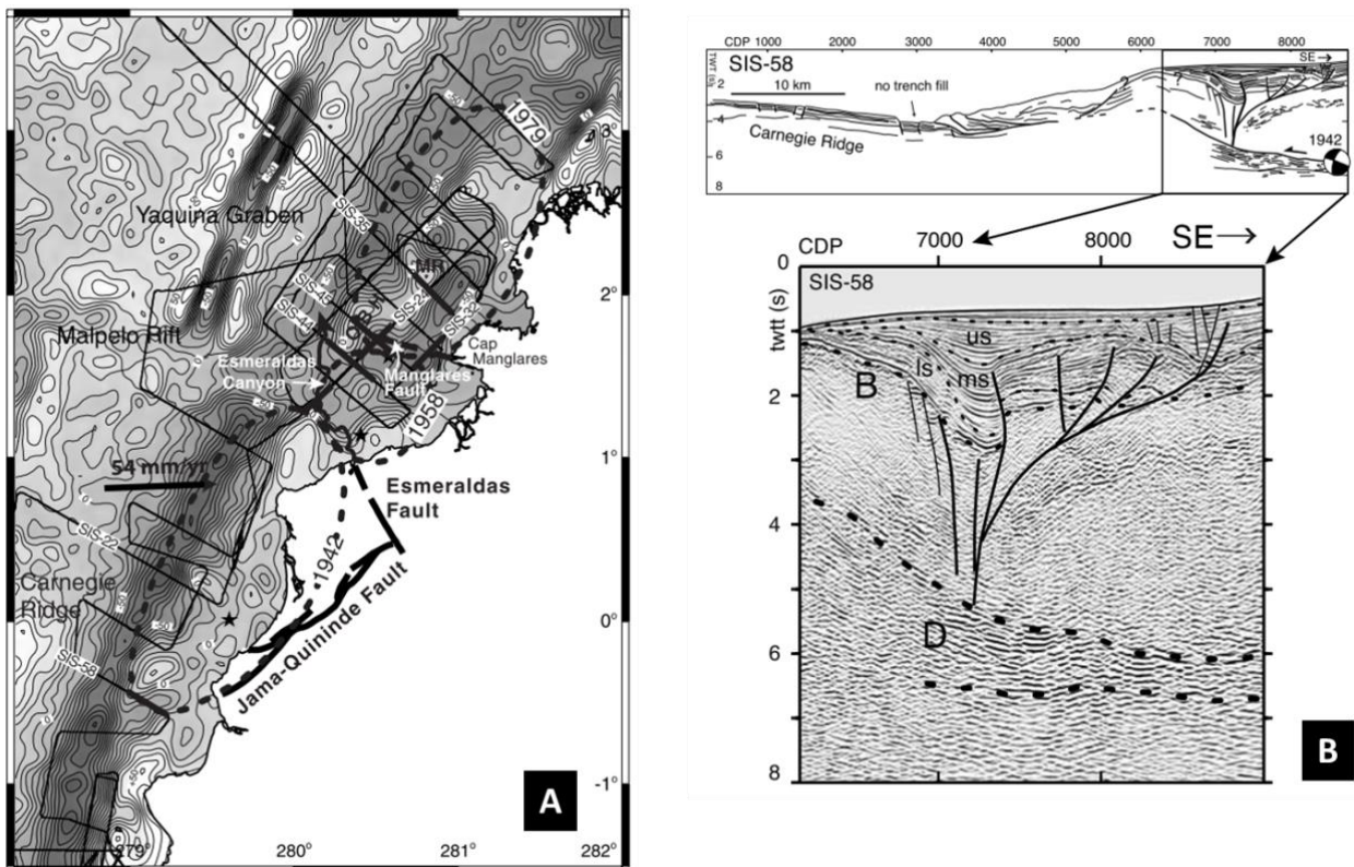
Figure 2.14: Offshore prolongation of the Jama fault system (Collot et al., 2004). A) Gravity anomaly map and location of the Jama fault system (Jama-Quininde Fault). B) Seismic profile showing a flower structure, which prolongs the offshore the Jama fault system.
