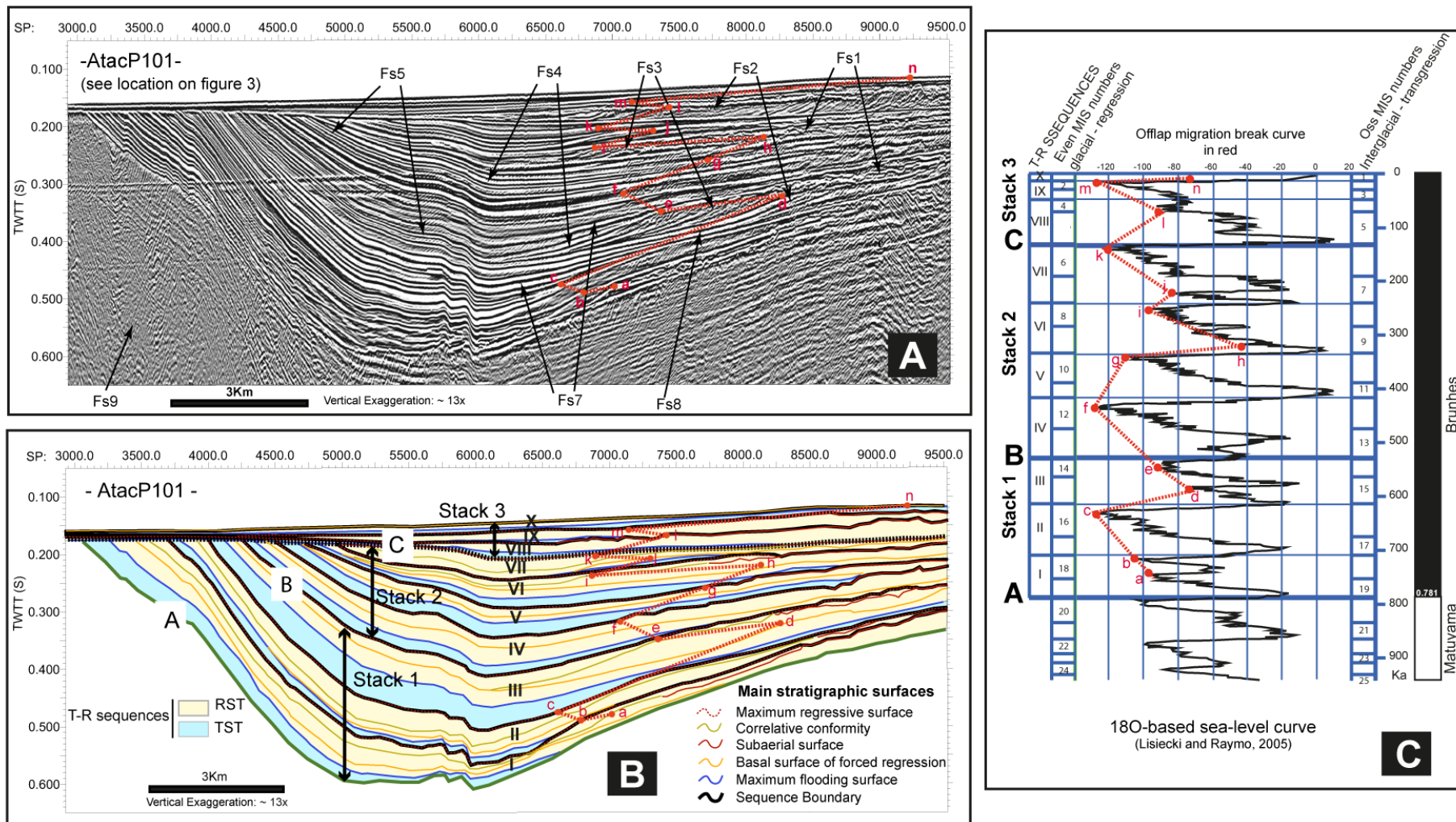
Figure 4.11: Comparison of the Pleistocene ^{18}\text{O} -based sea-level curve (Lisiecki and Raymo, 2005) with the migration in space and time of the point of offlap break (i.e. maximum seaward shift of the shoreline) of each T-R seismic sequence picked along a seismic line perpendicular to the present day shoreline.
