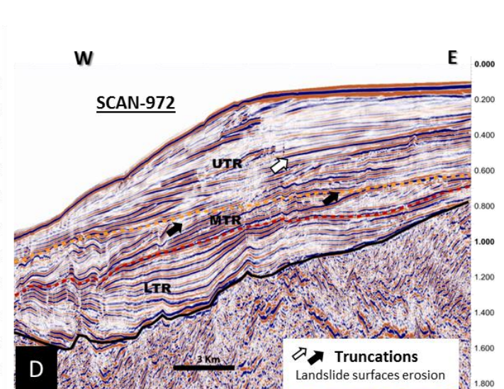
Figure 5.7: Seismic profile showing in the Cojimies basin: the seismic facies, the T-R sequences and System Tracts
