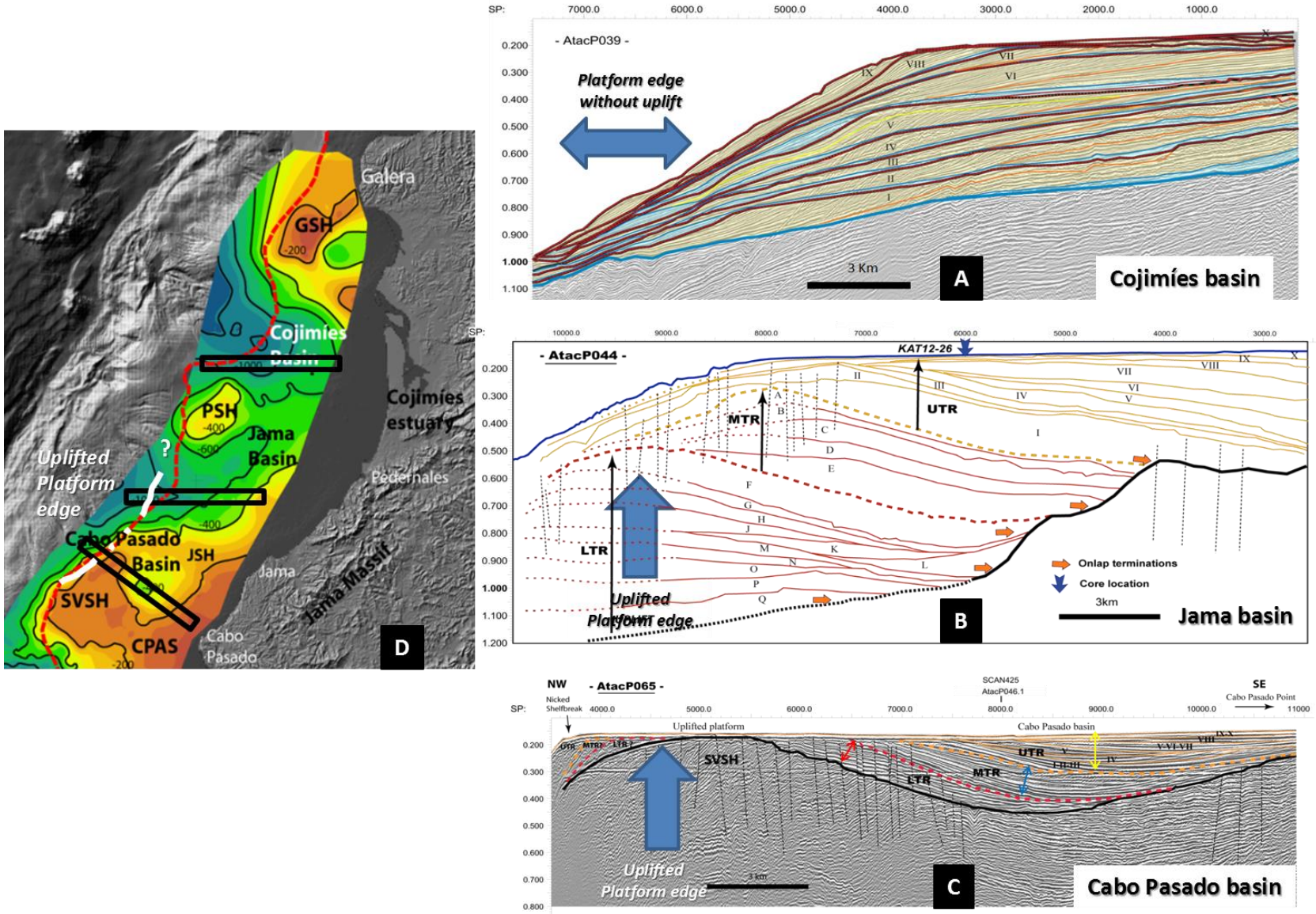
Figure 6.4: Differential behavior of the Platform edge displayed in the Northern basin, showing the uplift from the south side of the Jama basin.
