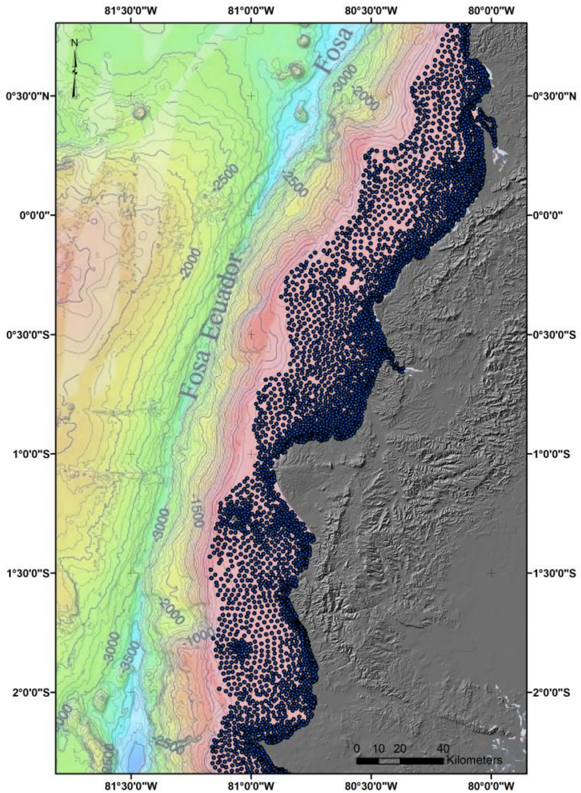
Figure 3.3: Single bean bathymetry data at the Ecuadorian central shelf. Data obtained from I.O.A.-1:100.000 nautical charts (INOCAR- different years).
