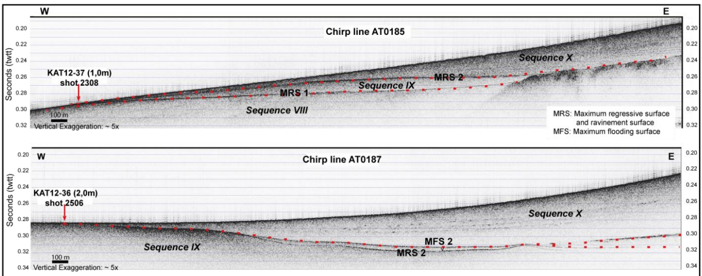
Figure 4.9: Piston core data collected in front of Manta peninsula. Piston core KAT12-37 samples T-R seismic sequences VIII to X, whereas piston core KAT12-36 samples T-R sequences IX and X as shown on the 3.5KHz chirp lines AT0185 and AT0187. See text for details and the interpretation of shell beds. The shell beds underline stratigraphic surfaces that correlate to depositional sequences exposed along the coast.
