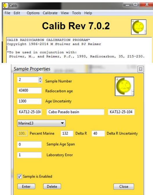
Figure 3.8: Software and marine reservoir database used for calibrating the laboratory-measured ages from the shell. The used correction parameters were taken from the nearest and most recent measurement of marine reservoir age obtained from the Marine13 dataset located near of Talara (Etayo et al. 2014).
