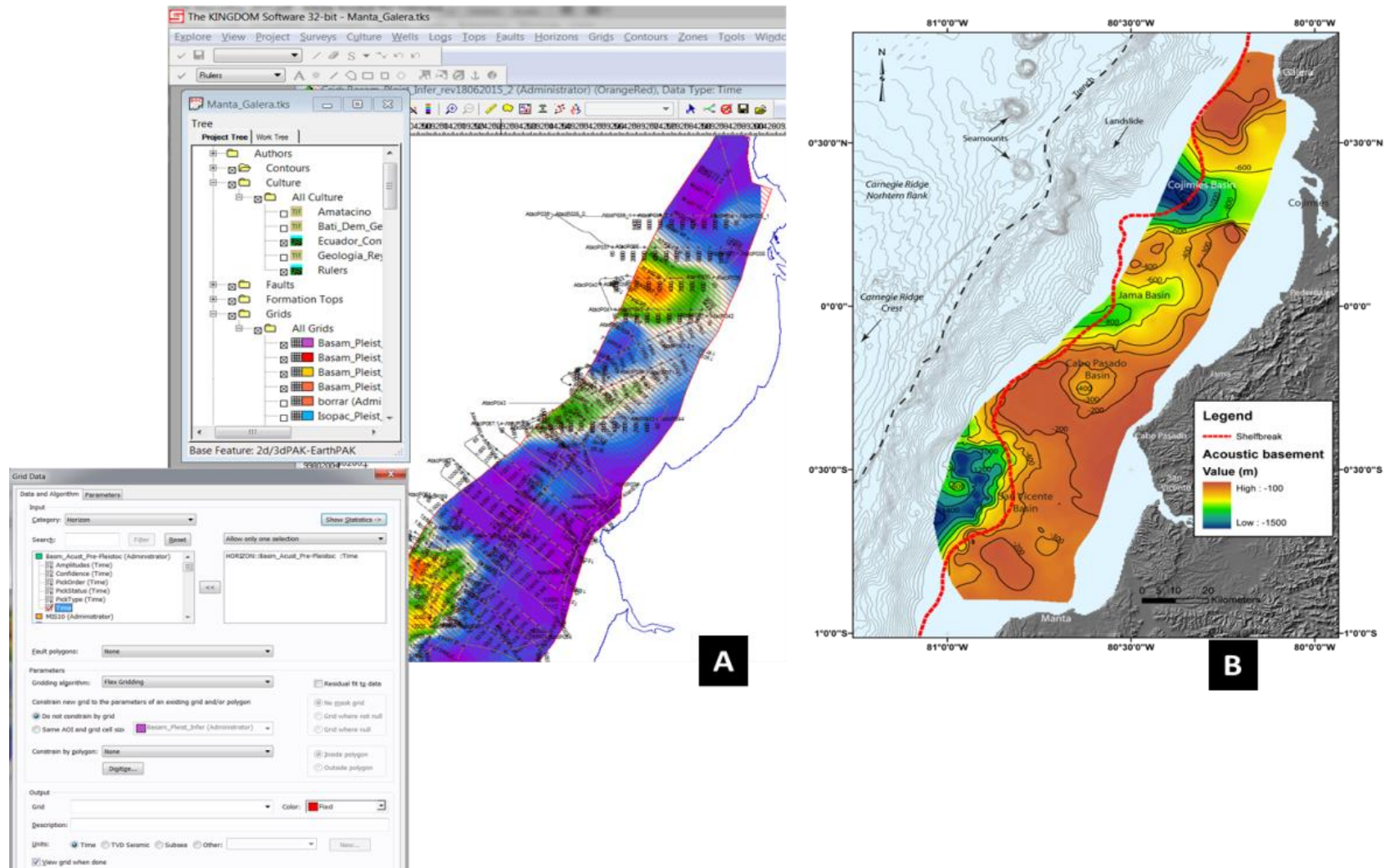
Figure 3.6: A) The Quaternary bottom-grid deduced from seismic data using the Kingdom software. B) The depth conversion of the grid was carried out using the Arcgis software, assuming a sound velocity of 1900 m/s.
