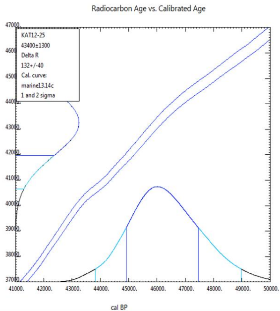
Figure 3.8: Software and marine reservoir database used for calibrating the laboratory-measured ages from the shell. The used correction parameters were taken from the nearest and most recent measurement of marine reservoir age obtained from the Marine13 dataset located near of Talara (Etayo et al. 2014).
