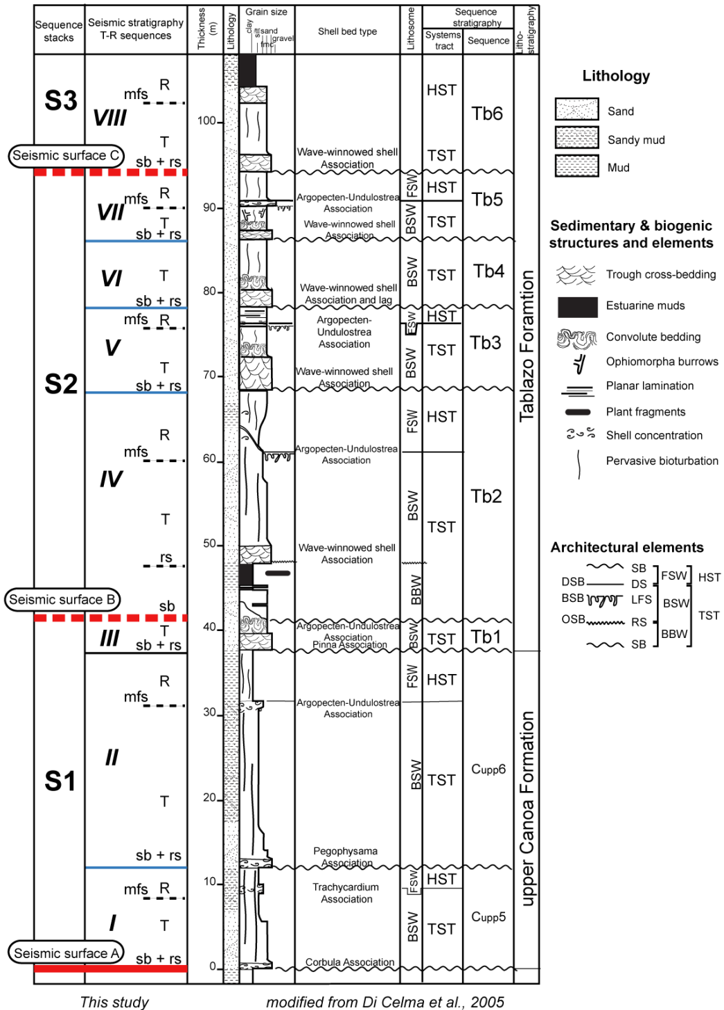
Figure 4.10: Details of the correlation of the T-R seismic sequences with the depositional sequences described onshore by Di Celma et al. (2005). Unconformities A and C at base of stacks of T-R sequences 1 and 3, correspond on land to angular unconformities at base of depositional sequence Cupp5 and Tb6. Seismic surface B correlates to a sharp surface at base of Tb2. The
