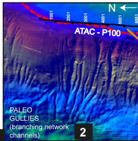
Figure 4.3: Map of Manta Peninsula-Plata area shows the bathymetry of the shelf, the slope, the trench and the eastern flank of the Carnegie Ridge.
