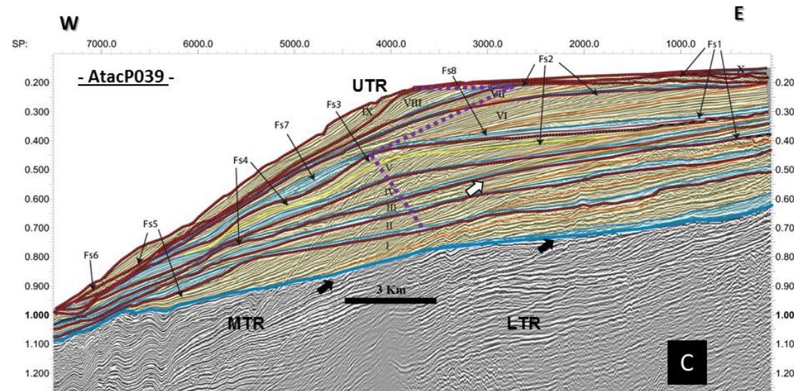
Figure 5.7: Seismic profile showing in the Cojimies basin: the seismic facies, the T-R sequences and System Tracts
