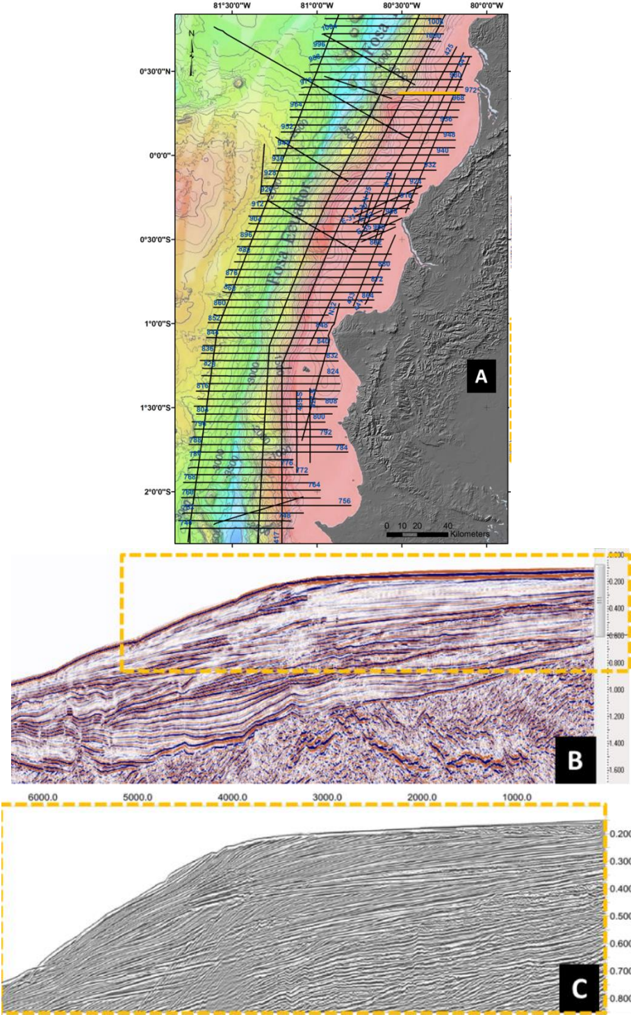
Figure 3.2: A) SCAN multichannel seismic data location. B) Example of the SCAN seismic profile. C) Example of the ATACAMES seismic line. We can note the significant differences in resolution and penetration between the SCAN and ATACAMES seismic data. SCAN data were used in places where Quaternary basins are very thick and difficult to identify with the ATACAMES seismic profiles.
