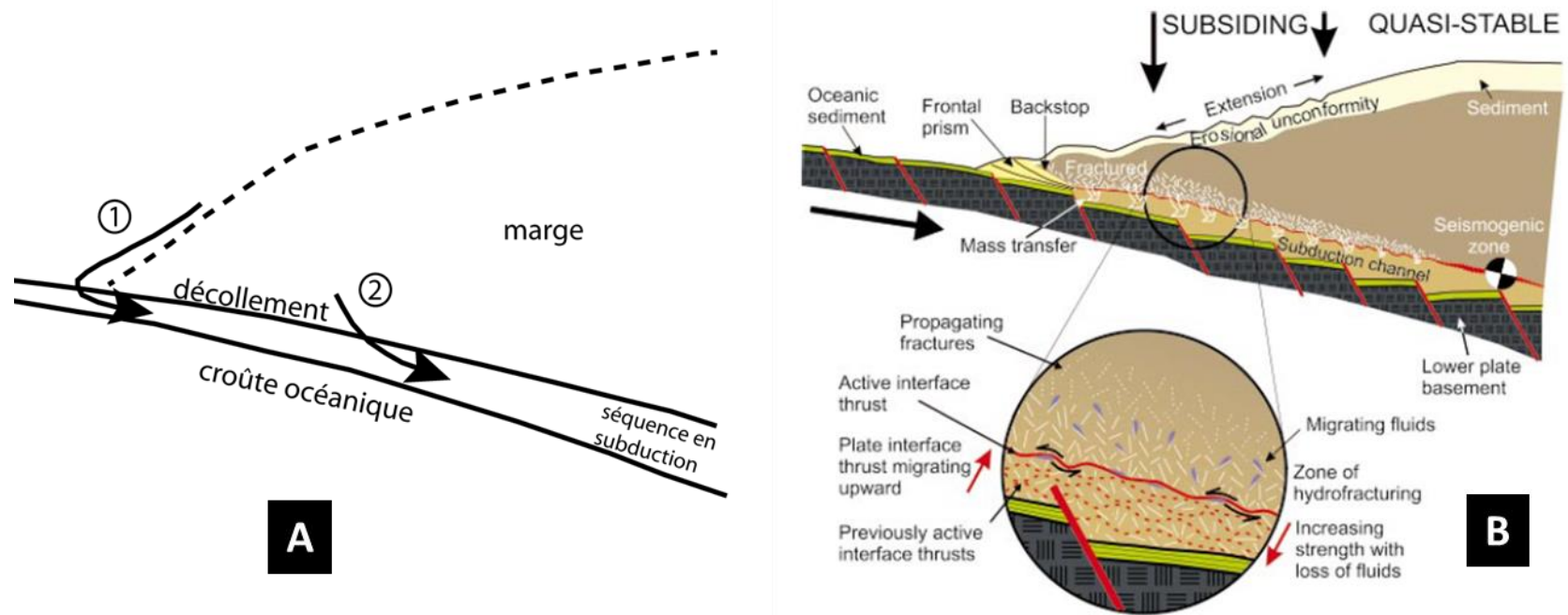
Figure 1.3: The subduction erosion process. Diagrams A from Lallemand (1992) and B from von Huene et. al (2004) show the two types of tectonic erosion of a subduction margin. A) Frontal erosion is caused by surface collapse over the slope's base, transporting the eroded material to the subduction interplate zone (arrow 1). The basal erosion drags the material from the prism to the subduction channel (arrow 2). B) Basal erosion is caused by hydro-fracturing in the interplate zone and fractures propagation at the base of the overriding plate.
