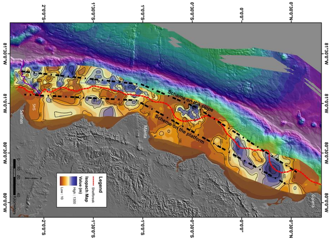
Figure 6.1: Stratigraphic scheme profiles on the slope (Figure 6.1A) and on the platform (Figure 6.1B). See the profile in the two next pages.
