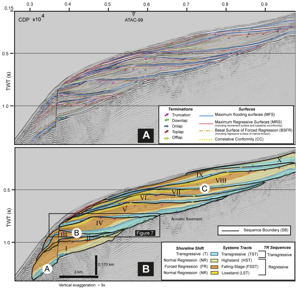
Figure 4.6: Seismic profile ATAC_P092 (see location map on figure 4) showing the seismic reflector terminations with interpreted surfaces (A), systems tracts, depositional sequences and regional unconformities labeled A, B, and C (B).
