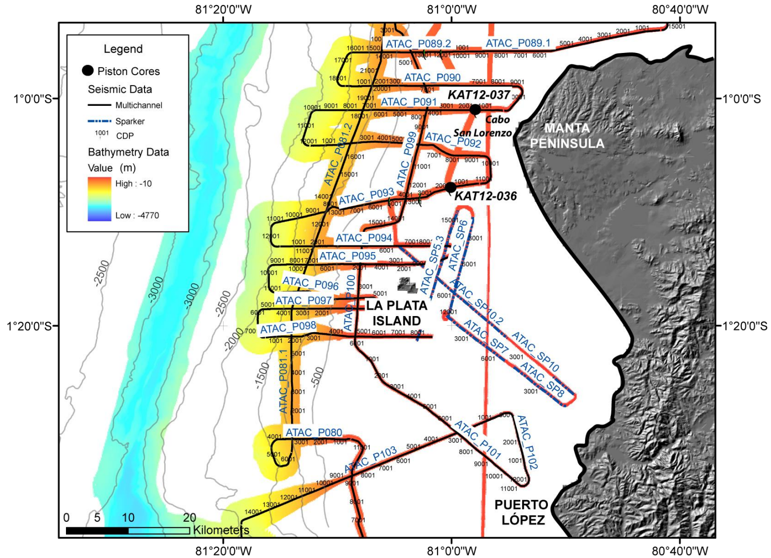
Figure 4.4: Location map of the bathymetry, 3.5 KHz chirp, sparker and MCS seismic data acquired during the ATACAMES (CNRS-IRD) campaign in 2012 in Manta-Plata area as well as the location of the two piston cores considered in this study.
