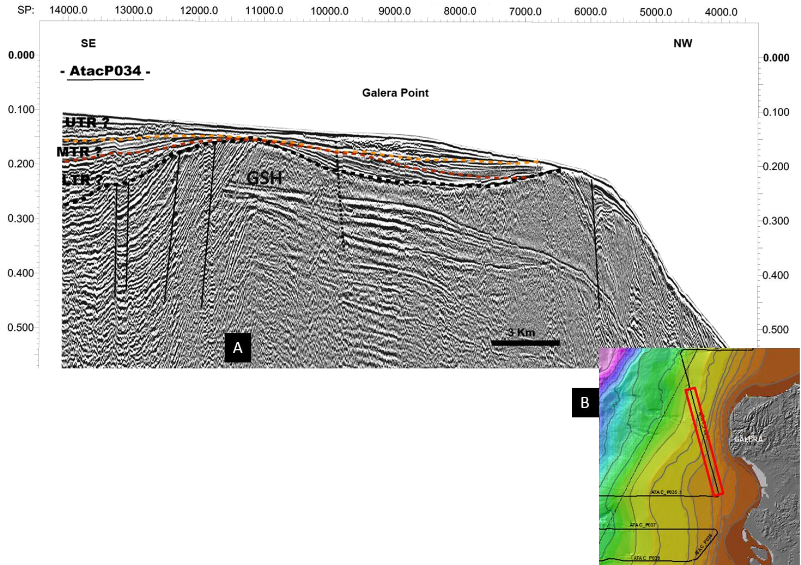
Figure 5.6: Seismic profile interpretation showing the interpreted TR sequences in front of Galera Cape. A) AtacP034 seismic profile, showing the interpreted TR sequences in front of Galera Point. We can note the uplift of the Galera Structural High (GSH), which borders the Cojimies basin on the northern side. B) Location of the seismic line in the margin.
