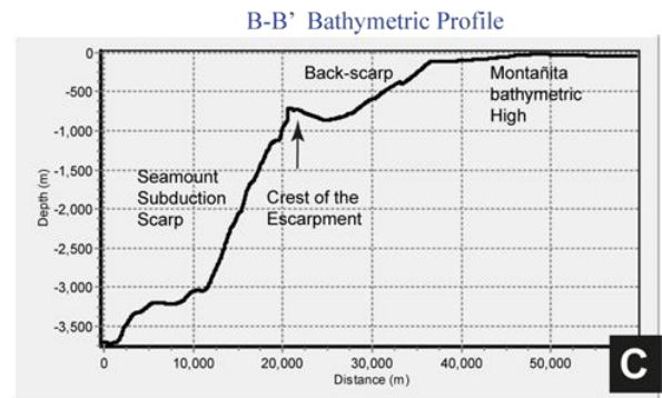
Figure 5.3: Seafloor morphology of the Southern zone (Salango Island-SalinasCape).
