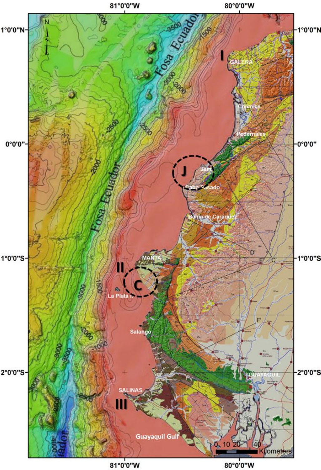
Figure 2.8: Geological map showing the onshore Quaternary outcrops. Composition map from Reyes (2013) and Michaud et al. (2006).
