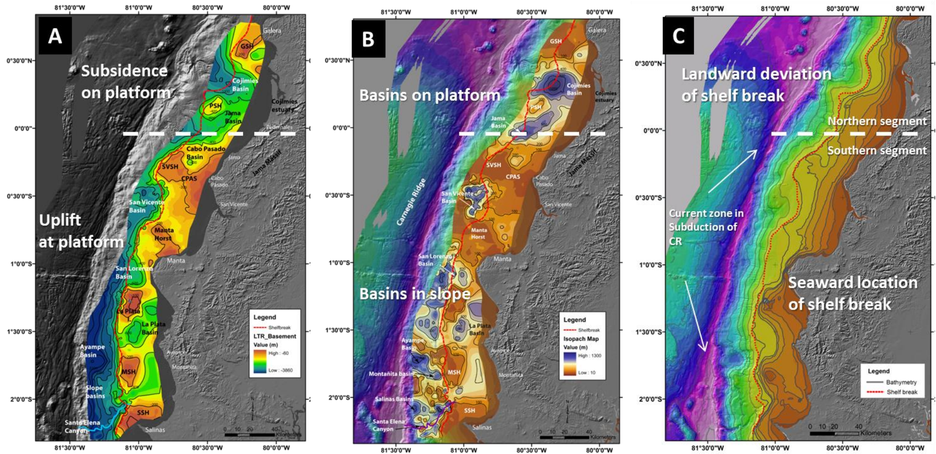
Figure 6.10: Different behaviors between the Northern and Southern segments displayed on the grids of the Acoustic Basement, the Isopach map and Seafloor Morphology. A) Grid of the acoustic basemen showing the subsidence at platform in the northern zone and the uplift at platform in the southern zone. B) The isopach map displaying the location of the basins along of the margin. C) The bathymetry grid presenting the different behavior of the shelf break between the northern and the southern zones.
