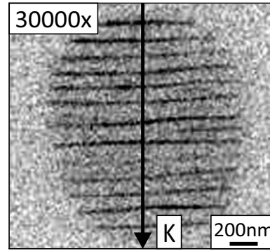
FIGURE 3.4: Scanning electron microscope image of silica glass surface showing light induced nano-grating formed by focused femtosecond laser beam irradiations. Arrow illustrates the direction of the nano-grating wavevector that is parallel to incident beam polarization direction. Adapted from Ref. [42].
