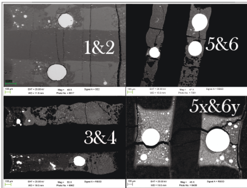
Figure 56 SEM-BSE images showing all the multi-anvil experiments. All experiments were done at 8GPa and 1950° C. The darker phases in the sample are corundum and spinel crystals.
