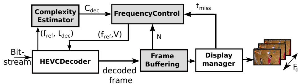
Figure 5.12: Boosted DVFS HEVC Decoder software setup
