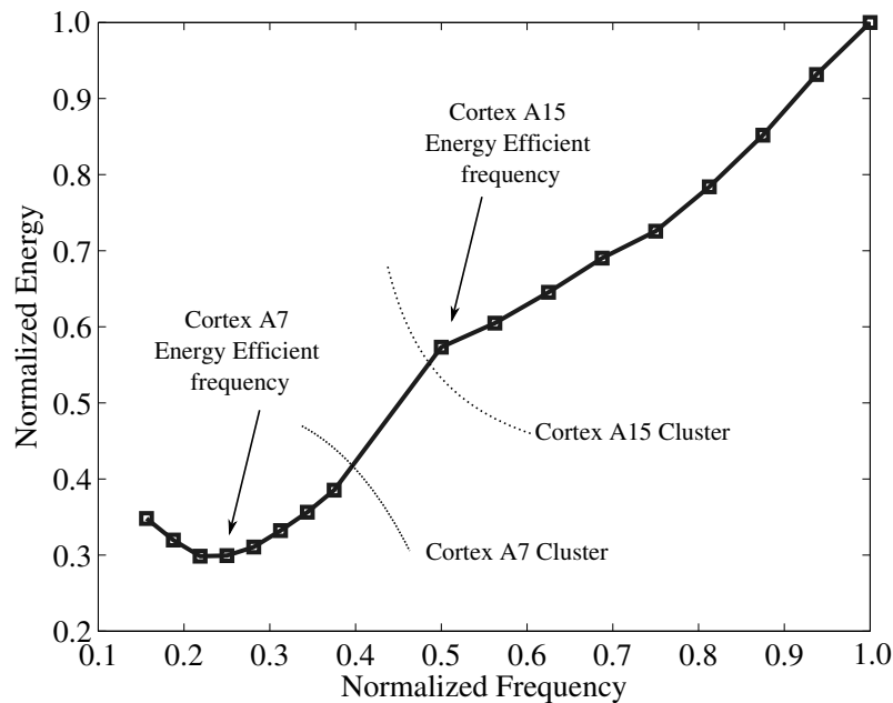
Figure 4.12: Energy per cycle as a function of normalized operating frequency of a fully loaded Exynos 5410
