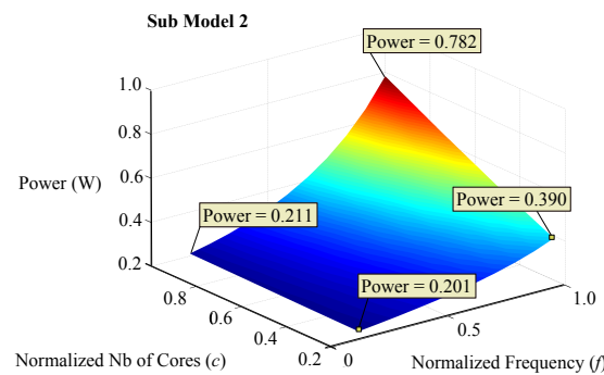
Figure 4.23: Sub-Model 2: Power characteristics
