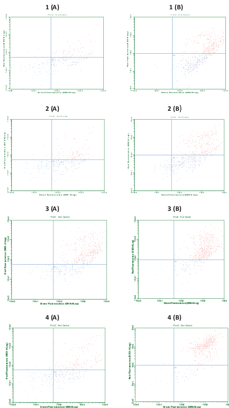
Figure 3.6. Cytoplots of the four idiosyncratic drugs (1) trovafloxacin, (2) nimesulide, (3) nefazodone and (4) telithromycin in absence (A) and presence (B) of pro-inflammatory stimuli. After incubating HepG2 cells with the four idiosyncratic drugs in absence (A) and presence of LPS and TNF- \alpha (B) for 24 hours, hepatocellular death was assessed following the simultaneous staining of cells with AnnexinV-FITC and PI by capillary flow cytometry. The amplified hepatocellular death observed when drugs were co-administered to cells along with LPS and TNF is illustrated in the presented cytoplots by an increase in both green and red fluorescence.
