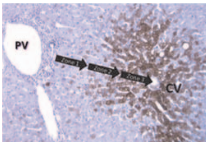
Figure 1.2. Structural and functional zonation of the liver. Immunostaining of human liver tissue with antibodies against CYP3A4 (brown stain) showing the differential expression of CYP enzymes across the zones of the liver microstructure. The greatest expression of CYP enzymes is predominantly in pericentral hepatocytes (zone 3) with a distinct boundary or gradient at the mid-lobular region (zone 2) PV: Portal Vein; CV: Central Vein. ( Adapted from LeCluyse et al. 2012 ).
