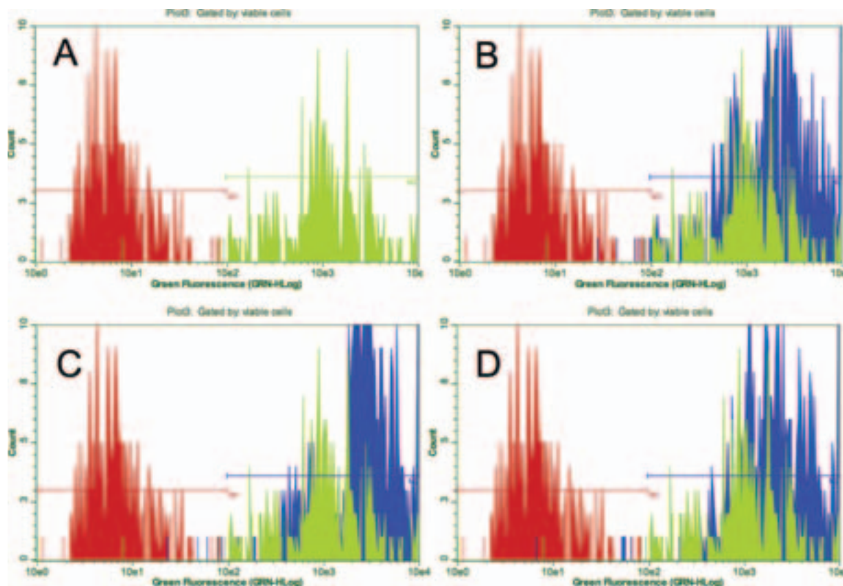
Figure 3. Intracellular retention of rhodamine 123 in HepG2 cells in the presence of 0.5 \mu M Rhodamine 123 (A), 100 \mu M Verapamil (B), 70 \mu M Nefazodone (C), and 175 \mu M Telithromycin (D). Prior to cytometry analysis cells were treated as described under Materials and Method . Histograms represent the cell counter numbers versus geo-mean fluorescent intensity (AU). In each figure, three overlaid histograms represent, from left to right, the peak from auto-fluorescence of control cells without rhodamine 123, the peak from rhodamine loaded-cells and the peak from rhodamine loaded-cells in the presence of verapamil (B), nefazodone (C), and telithromycin (D). [Color figure can be viewed in the online issue which is available at wileyonlinelibrary.com ]
