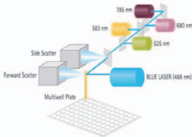
Figure 2.1. Optical layout of Guava EasyCyte Plus capillary flow cytometer. (Adapted from http://www.millipore.com ).
