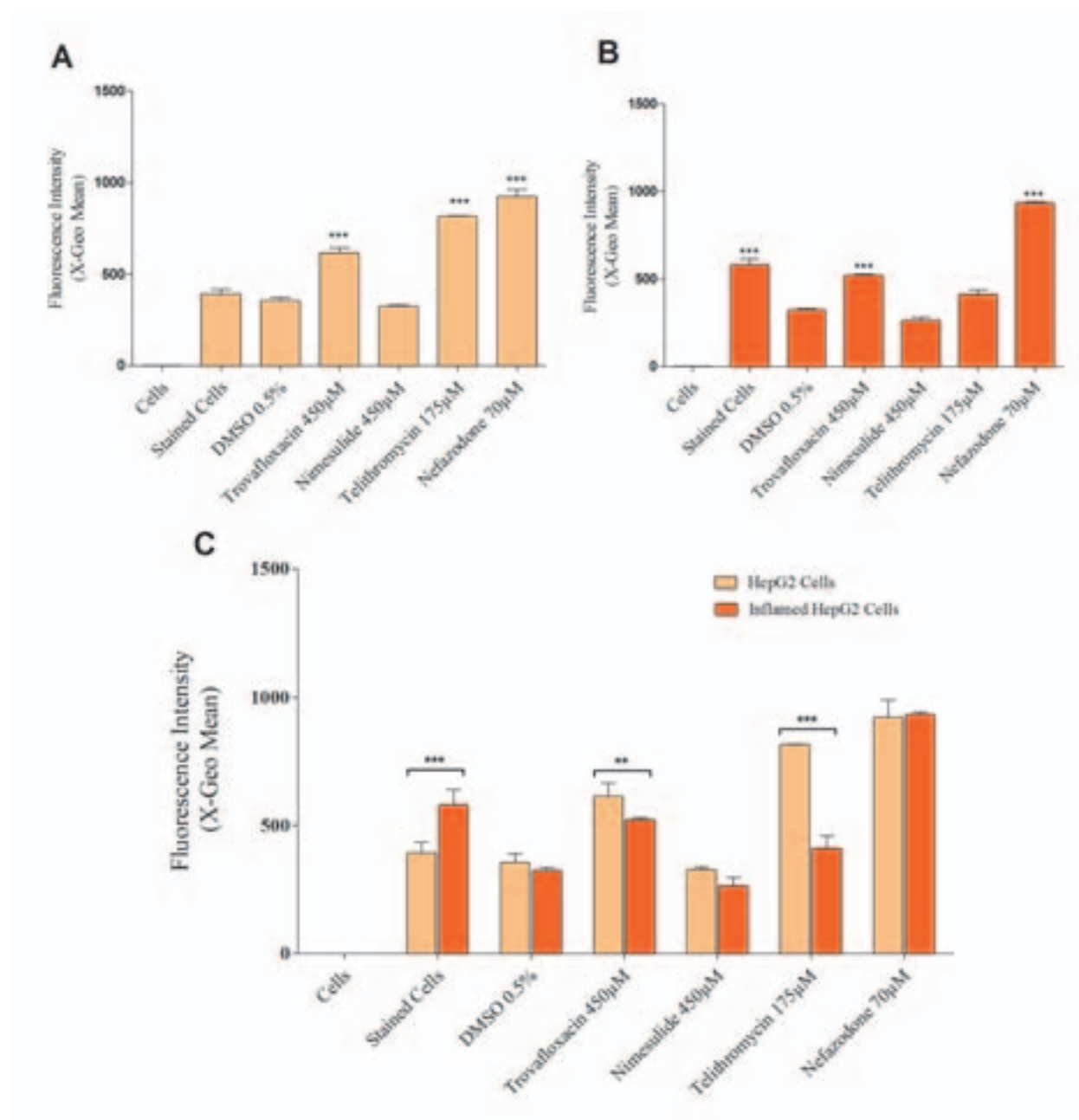
Figure 3.9. The steatotic effect of idiosyncratic drugs in non-inflamed and inflamed HepG2 cells. After co-incubating HepG2 cells with the four idiosyncratic drugs in absence (A) and presence of LPS and TNF- \alpha (B) for 24 hours, the intracellular accumulation of lipids, otherwise known as steatosis was assessed using BODIPY 493/503 by flow cytometry. Graph C represents the steatotic potential of the four tested idiosyncratic drugs in absence and presence of LPS and TNF- \alpha . Bars represent the accumulated intracellular fluorescence of BODIPY 493/503 in terms of X-geometric mean (AU). Data is represented as Mean \pm S.E.M (n=3). Statistical analysis was performed using one way (for graphs A and B) and two way ANOVA (for graph C) followed by Bonferroni post test. ** and *** represents P < 0.01 and P < 0.001 , respectively, and refers to the variation in steatotic potential between DMSO-treated and drug-treated HepG2 cells in graphs A and B. In graph C the p-value corresponds to the variation in steatotic potential between non-inflamed and inflamed HepG2 cells.
