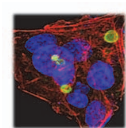
Figure 2.6. Immunostaining of HepG2 cells with anti-MRP2 (green), DY-554 phalloidin (red) and DRAQ5 (bleu pseudocolor). (Adapted from Cell Signaling technology official website: http://www.cellsignal.com/products/4446.html ).
