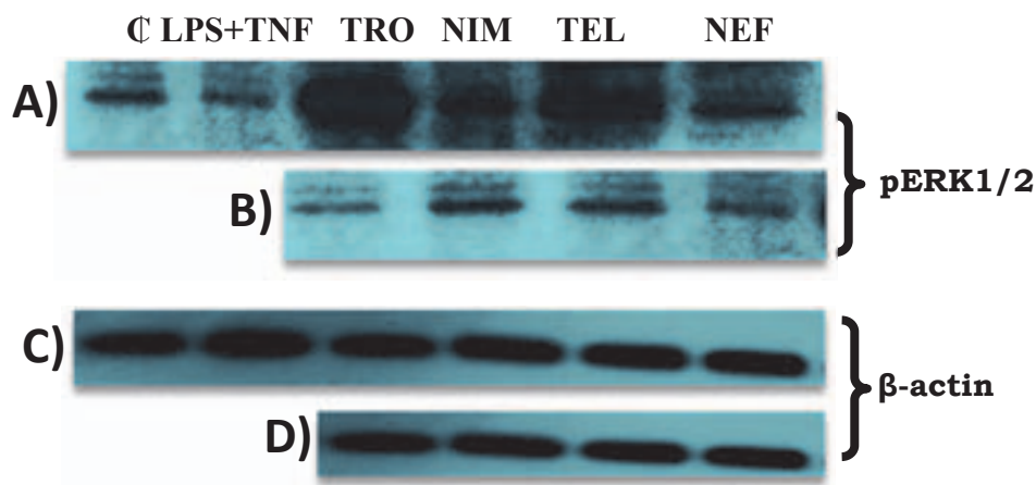
Figure 5.8 (A). Effect of idiosyncratic drugs on the expression of pERK \frac{1}{2} proteins in HepG2 cells in absence and presence of pro-inflammatory stimuli. Immunoblot analysis of pERK \frac{1}{2} protein expression was performed following 24 hours incubation of HepG2 cells with the four idiosyncratic drugs in presence (Lane A) and absence (Lane B) of LPS and TNF- \alpha . Lanes C and D demonstrate the expression of \beta -actin corresponding to every loaded sample (internal control). The attained results demonstrate that trovafloxacin, nimesulide and telithromycin induce the expression of pERK \frac{1}{2} when co-administered to HepG2 cells along with LPS and TNF- \alpha ( C: negative control; TRO: trovafloxacin, NIM: nimesulide; TEL: telithromycin; NEF: nefazodone ).
