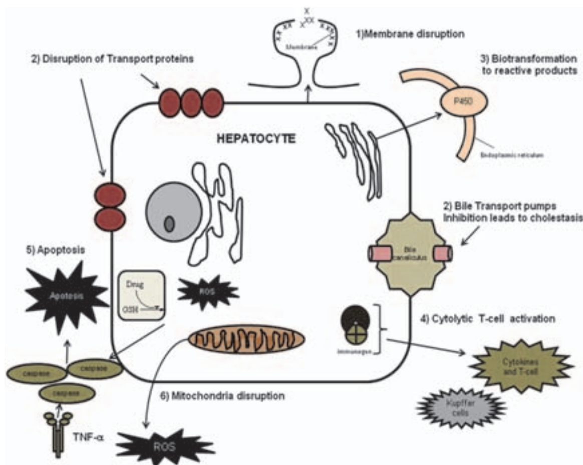
Figure 1.5. Mechanisms of hepatotoxic injury. Common cellular sites of hepatocyte injury are shown: 1) Membrane disruption (X) leads to disassembly of actin fibrils at the cell surface causing blebs and rupture of membrane; 2) Disruption of transport proteins or specifically bile transport proteins at the canalicular membrane interrupting bile flow; 3) Biotransformation by cytochrome P450 to reactive metabolites; 4) Cytolytic T-cell activation by resident macrophages, Kupffer cells in response to protein drug adduct acting as immunogen; 5) Apoptosis by TNF- \alpha or fas mediated activation of caspase pathway; and 6) Mitochondria disruption resulting in oxidative stress (ROS). (Adapted from Lee, 2003).
