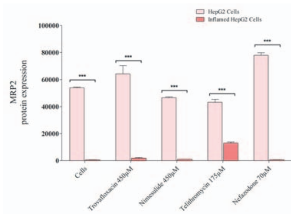
Figure 4.4 (B). Quantification of MRP2 protein expression by ImageJ in non-inflamed and inflamed HepG2 cells. After incubating HepG2 cells with the four idiosyncratic drugs in absence and presence of LPS and TNF- \alpha for 24 hours, the expression of MRP2 protein was assessed by western blot and quantified by image J. Bars represent the densitometric analysis of three different experiments (n=3). Data is represented as Mean \pm S.E.M. Statistical analysis was performed using two way ANOVA followed by Bonferroni post test. *** represents P < 0.001 and refers to the variation in MRP2 protein expression between non-inflamed and inflamed HepG2 cells. These results indicate that the co-presence of LPS and TNF- \alpha along with idiosyncratic drugs favor the reduction of MRP2 protein expression in an extremely significant manner.
