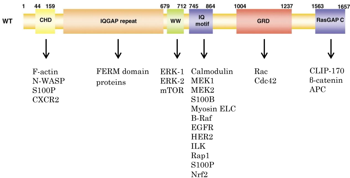
Figure I-13. IQGAP1 domains and its effector proteins. It shows the different domains of IQGAP1 and the principal molecules that bind each domain. CHD: calponin homology domain; WW: polyproline binding region; IQ motif: calmodulin binding repeat; GRD: RasGAP related domain; RGCT: RasGAP C terminus (154).
