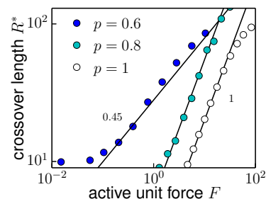
Figure 6.9: Crossover radius as a function of the active force, for 2D triangular lattices with variable depletion parameter. The black lines indicate power-law fits. Stretching-dominated networks ( p > p_c \approx 0.65 ), either depleted or regular, are well described by Equation 6.16. On the other hand, bending-dominated networks exhibit a clearly different behaviour, with smaller exponent. Parameters: R = 200 , \mu = 10^3 , average over 100 systems in disordered case.
