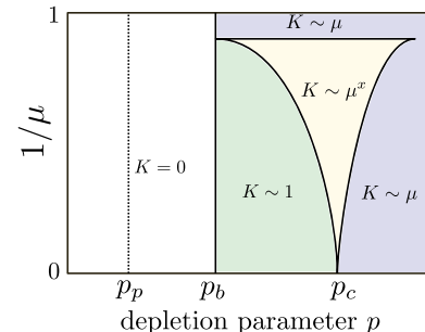
Figure 3.9: Schematic scaling diagram for the linear elastic modulus, as discussed in the text. We show the stretching-dominated regime (blue), the bending-dominated regime (green) and the intermediate, mixed regime around p_c (yellow). Floppy networks have vanishing modulus (white). For better legibility, the y -axis is the inverse of the stretching rigidity \mu .
