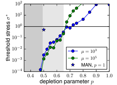
Figure 3.25: The typical stress \sigma^* for geometrically non-linear response. The buckling stress \sigma_b = 1 is indicated as a comparison (black line).
