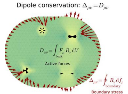
Figure 4.1: Dipole conservation relates local active forces to the resulting far-field stresses in linear elastic media.
