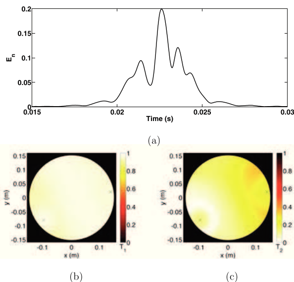
FIG. 6. (Color online) Reconstruction quality indicators for full DLTR imaging process: (a) E_n (best value: E_n = 0 ), (b) T_1 (best value: T_1 = 1 ), (c) T_2 (best value: T_2 = 0 ).
