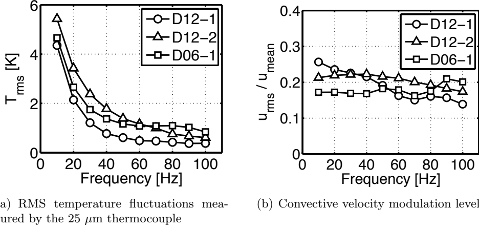
Figure 2.11: Root-mean-square temperature fluctuations T_{rms} and modulation level u_{rms}/u_{mean} as a function of the forcing frequency for the optimized operating conditions.
