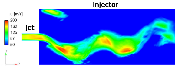
Figure 6.12: A snapshot of axial velocity from the 2D LES test of the jet in the case op13-5-0-85 showing the flapping movement of the jet.
