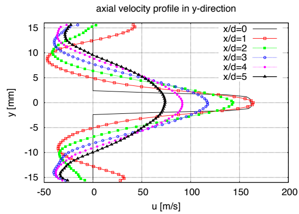
Figure B.2: Axial velocity profile along y -direction
