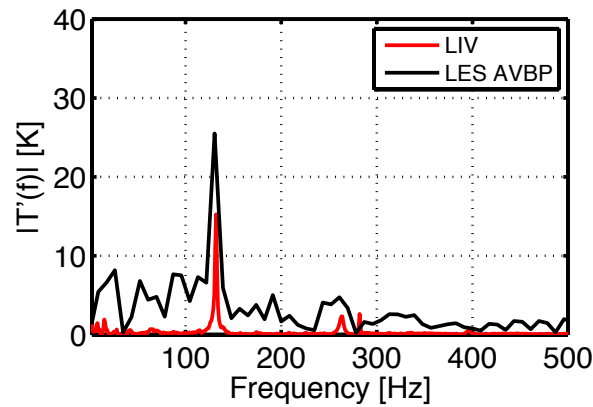
Figure 6.21: Amplitude spectrum of surface-averaged temperature fluctuations at x = 122.5 mm. LES (black line) and LIV (red line).
