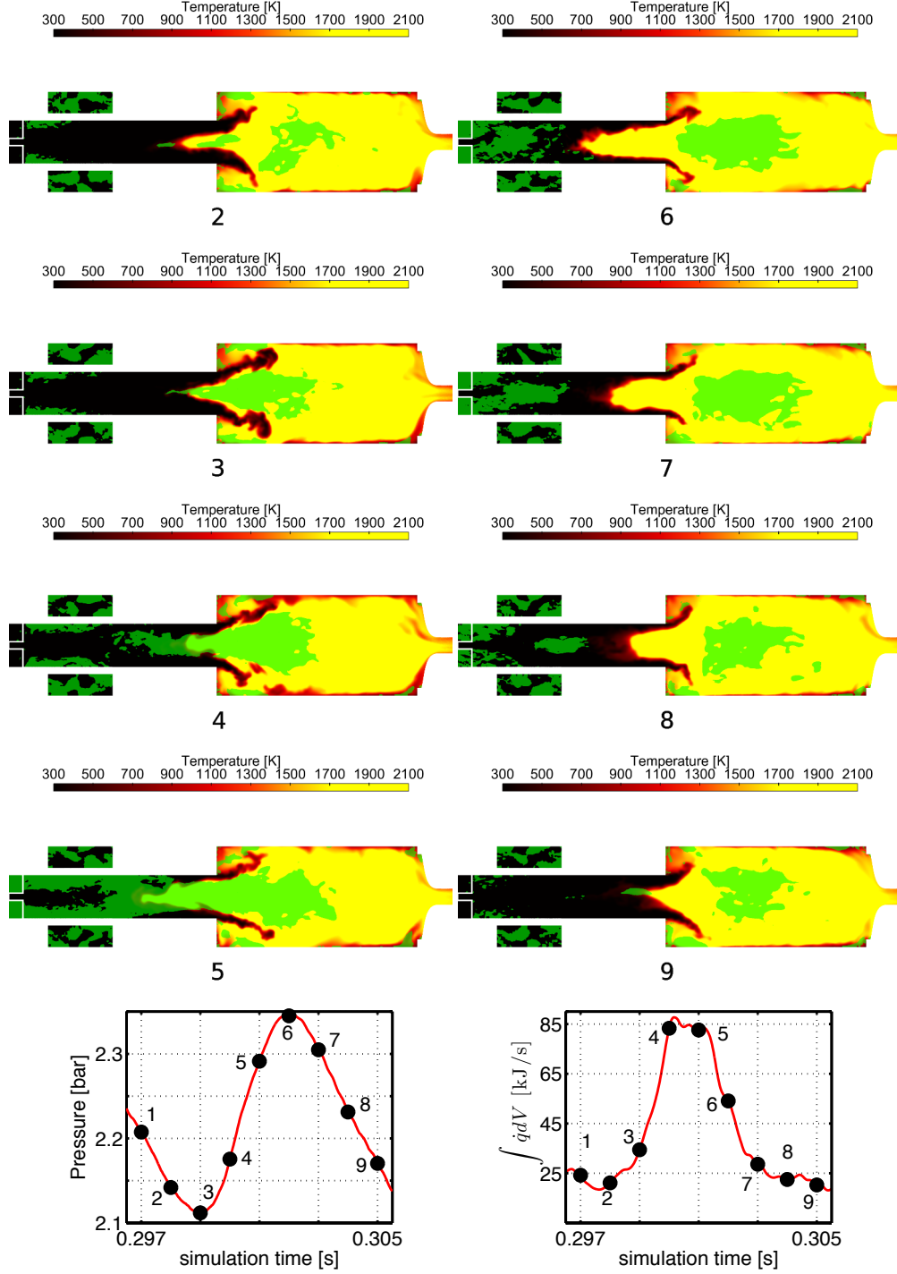
Figure 6.14: LES snapshots of temperature field for case op16-2-0-85. The green zone corresponds to the flow with non positive axial velocity u \leq 0 . Snapshot numbers are shown in the pressure signal from probe located at (x, y, z) = (0, 0, 0) , and also in volume integrated heat release rate. The time interval between 2 snapshots is 1 ms.
