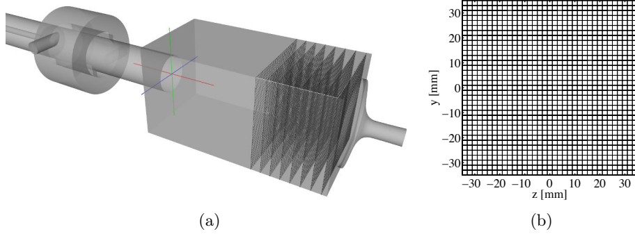
Figure 6.17: Interpolation grid. Eight 70 \times 70 \text{ mm}^2 transversal planes starting from x = 87.5 to x = 136.5 \text{ mm} with an equal distance of 7 \text{ mm} and discretized by square grids of 2 \times 2 \text{ mm}^2 .
