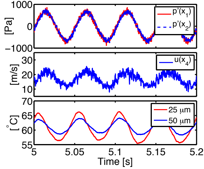
(a) Nozzle D12, M_u = 0.050 , u_{\text{rms}}/u_{\text{mean}} = 0.24 , modulation at f=20 Hz.
