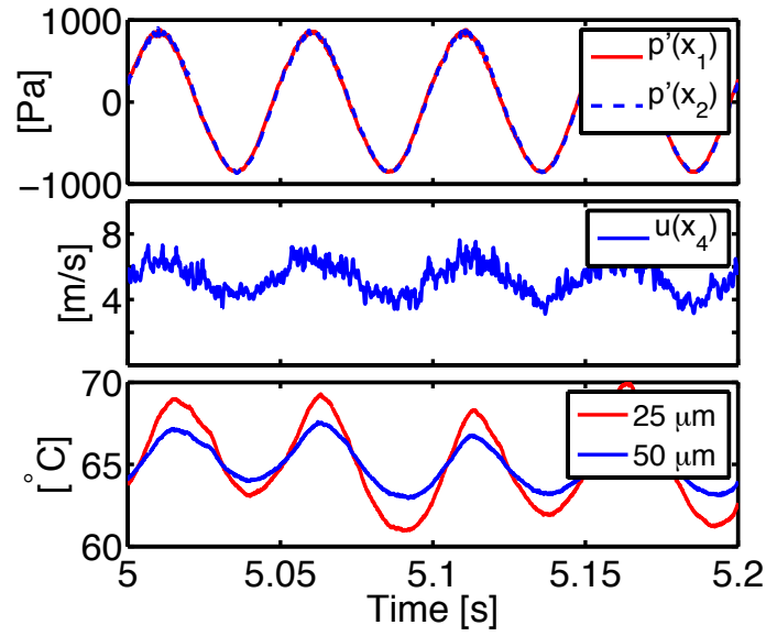
(b) Nozzle D06, M_u = 0.016 , u_{\text{rms}}/u_{\text{mean}} = 0.21 , modulation at f=20 Hz.
