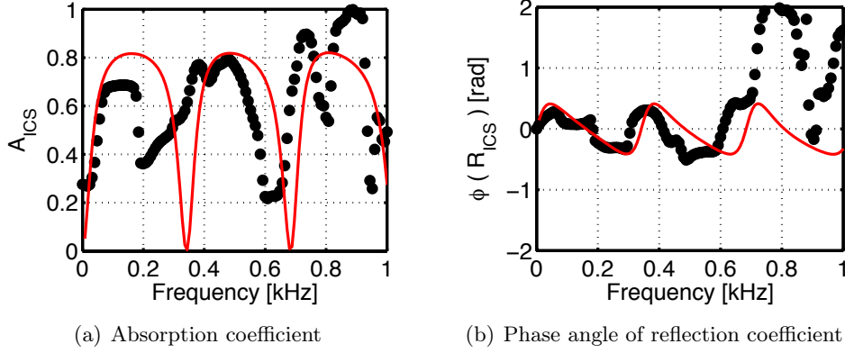
Figure 5.6: Acoustic properties of the perforated plate with a back cavity from LES (symbols) and analytical modified Howe's model (line). Case op16-0-2-85
