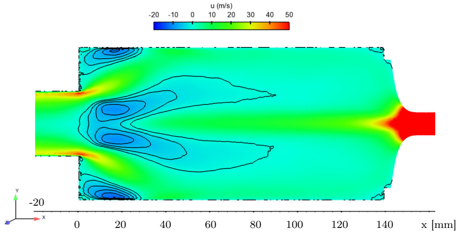
Figure 6.3: Axial velocity field from time-averaged non reactive simulation of the case op16-0-2-85 in the plane Z = 0 . Black lines indicates negative axial velocity u < 0 .
