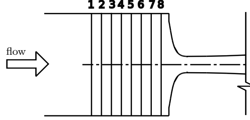
Figure 7.1: Schematic view of the 1D configuration for combustion noise analysis. 1st plane at x = 87.5 mm, 8th plane at x = 136.5 mm
