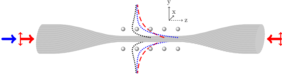
Figure 4.2: Two-color trapping scheme. An attractive red-detuned beam (dashed) and a shorter-range repulsive blue-detuned beam (dotted) are combined, resulting in a potential minimum in the fiber vicinity (solid line). An array is obtained by forming a standing wave with the red-detuned beams. The trapping sites are located in the yOz plane thanks to the use of red-detuned light quasi-polarized along y .
