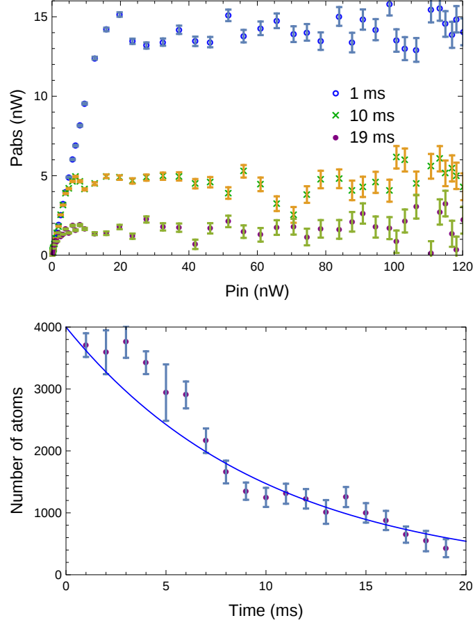
Figure 4.13: Top: Saturation of the absorbed power from a probe resonant on \{6S_{1/2}, F=4\} \rightarrow \{6P_{3/2}, F=5\} . The absorbed power ( P_{\text{in}} - P_{\text{out}} ) is given as a function of the input power. Bottom: Number of atoms derived with Eq. (2.3.1) as a function of time. The blue curve corresponds to an exponential decay with a 10 ms time constant.
