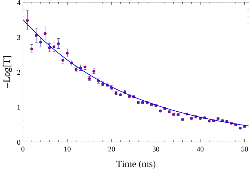
Figure 4.14: Transmission of a detuned probe as a function of time. The blue curve is an exponential decay with time constant 25 ms. The probe is detuned 15MHz away from the \{6S_{1/2}, F=4\} \rightarrow \{6P_{3/2}, F=5\} transition. Data from June 2015.
