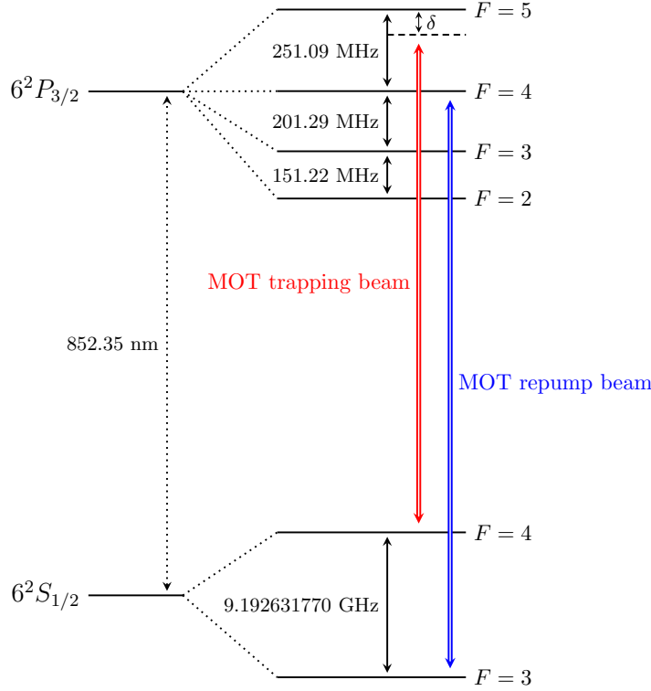
Figure 2.7: The D 2 line spectroscopic structure of cesium atoms, and the transitions used for the MOT implementation. The trapping beams are red-detuned by 10 MHz relative to \{6S_{1/2}, F=4\} \rightarrow \{6P_{3/2}, F=5\} transition.
