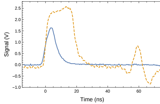
Figure A.5: APD detection pulse, before (solid line) and after shaping (dashed).
