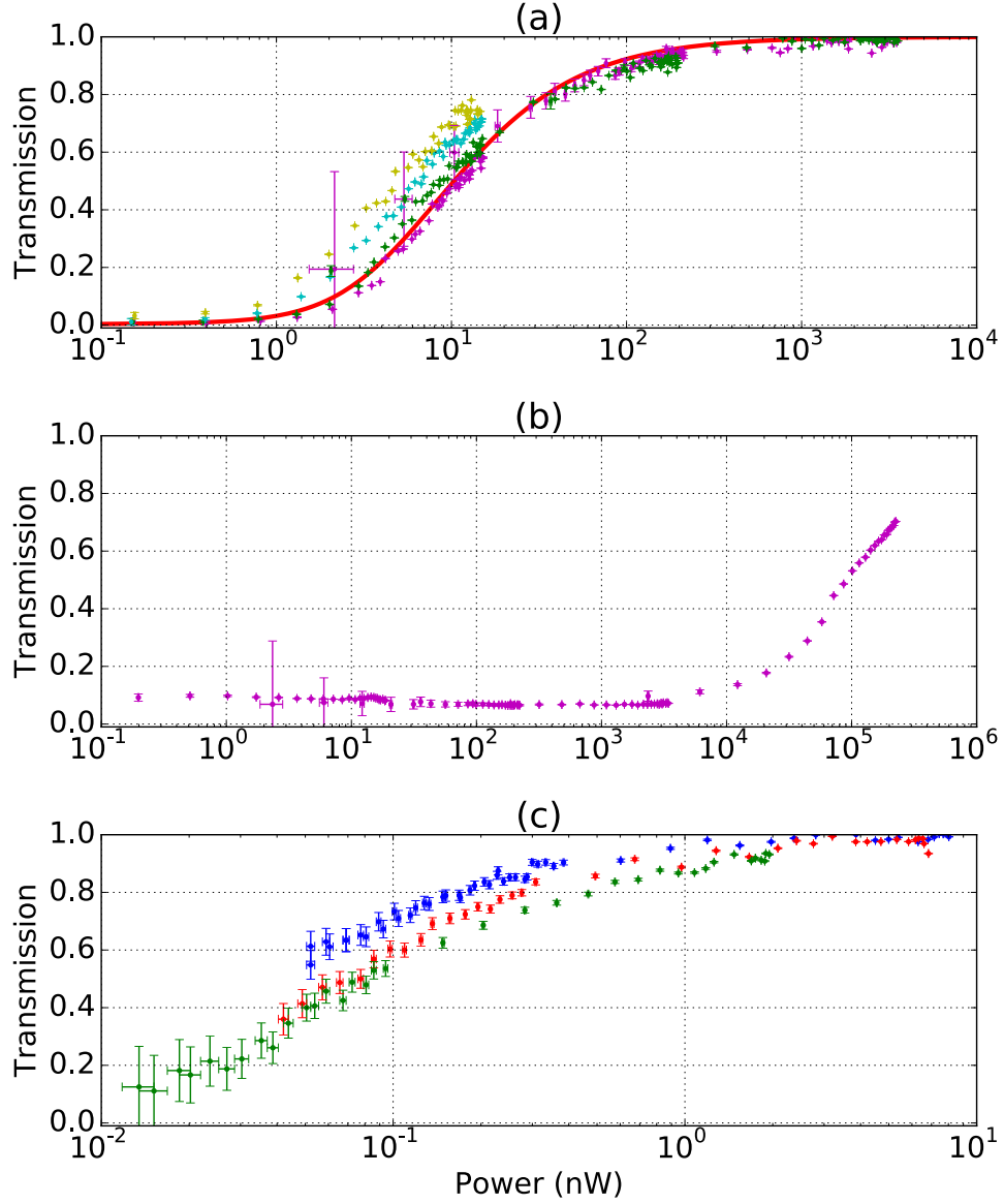
Figure 2.15: Absorption of a probe through a cold cesium cloud. (a) Probe on \{6S_{1/2}, F=4\} \rightarrow \{6P_{3/2}, F=5\} cyclic transition guided by the nanofiber. Different colors reflect shot to shot fluctuations of optical depth over an hour. The solid red curve is a fit described in the text. (b) Free-space probe (optical path described in subsection 3.2.1.1 ) on \{6S_{1/2}, F=4\} \rightarrow \{6P_{3/2}, F=5\} cyclic transition. (c) Guided probe on \{6S_{1/2}, F=4\} \rightarrow \{6P_{3/2}, F=4\} "pumping" transition. For this figure, the pulse durations are 10 \mu s (blue), 5 \mu s (red) or 1 \mu s (green). Error bars for all figures correspond to the lower signal/noise ratio at low powers. Points for higher powers ( > 10 nW) are measured with an attenuator in front of the detector.
