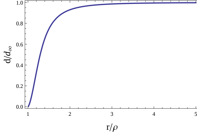
Figure 2.17: The atomic density close to the nanofiber surface. This result is obtained from Eq. (2.3.4) with T = 200 \mu\text{K} , U_{VdW}(r) = -\frac{C_g}{(r-\rho)^3} , and C_g = 1.56 \text{ kHz} \cdot \mu\text{m}^3 . The order of magnitude chosen for the temperature was later confirmed by time of flight measurements.
