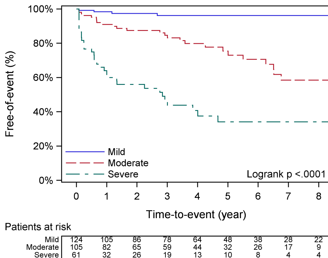
Figure 3.11. Kaplan Meier survival free of MACE according to VHD severity.
