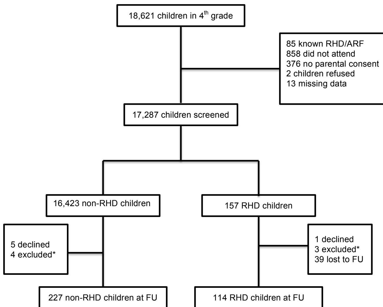
Figure 3.2. Flow chart of the cohort study on outcomes in asymptomatic echocardiography-screened RHD.*Other diagnosis after serial echocardiography (CHD).
