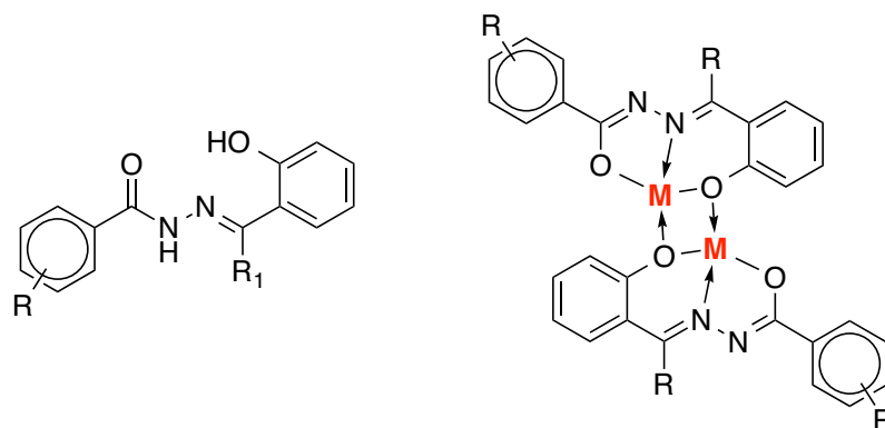
Figure 10. Complexes portant un ligand tridente aroyle-hydrazone N,O, \mu -O.
