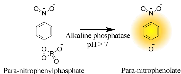
Figure 5.6: Transformation of para-nitrophenylphosphate in UV absorbant para-nitrophenolate under alkaline phosphatase activity.
