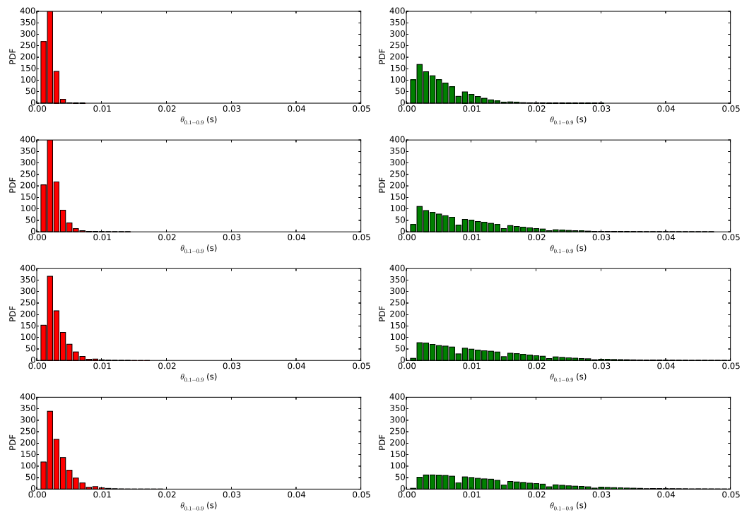
Figure 4.21: Histograms of the rise time for increasing propagation distances. Left: \sigma = 0.5 \text{ m}\cdot\text{s}^{-1} in red and right \sigma = 2.0 \text{ m}\cdot\text{s}^{-1} in green.
