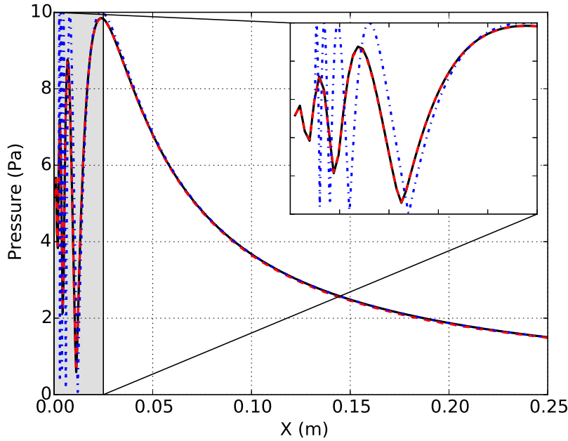
Figure 3.3: Pressure amplitude on the axis of a 3D pressure piston. — FLHOWARD computation, - - - Analytical solution and - . - . Analytical solution for the parabolic equation. The near-field is zoomed.
