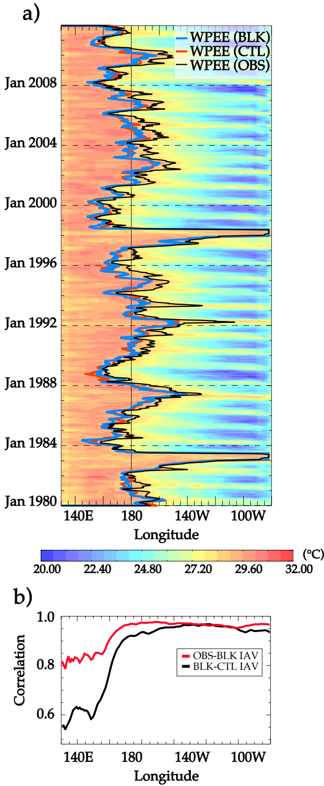
FIGURE IV.5 – (a) Equatorial (2°N-2°S average) time-longitude evolution of observed daily SST (Tropflux product) in the Pacific over the 1980-2012 period. The thick black line represents the observed position of the Warm Pool eastern Edge (WPEE) defined as the 28.5°C isotherm. The thick red and blue lines respectively depict the WPEE location in the CTL and BLK simulation respectively. b) Correlation coefficient of interannual SST variations along the equator (2°N-2°S average) between (black) the BLK simulation and observations and (red) BLK and CTL simulations as a function of longitude.
