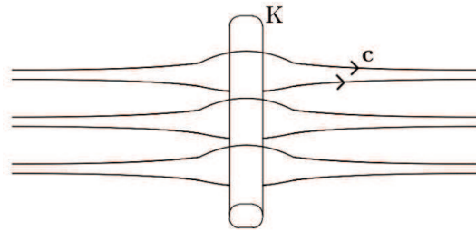
Figure 3.2: Vector field \mathbf{c} avoiding lateraly a tube K
