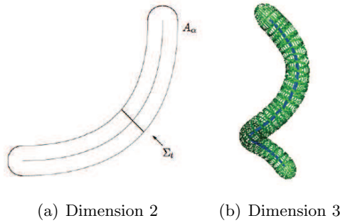
FIGURE 3.1. Tubes A_\alpha
