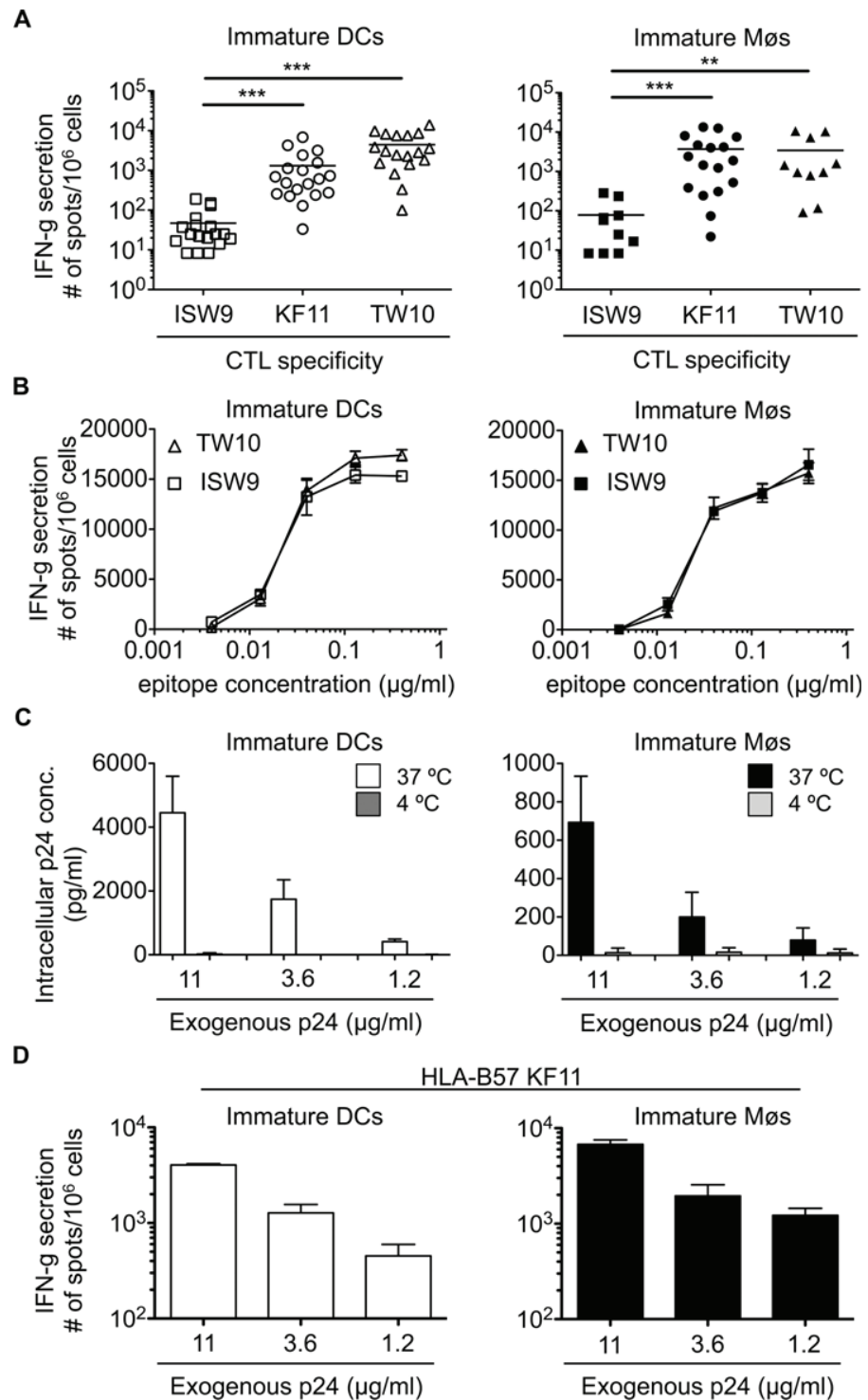
Fig 1. The immunodominant HLA-B57-restricted TW10 and KF11 epitopes are more efficiently cross-presented than subdominant ISW9 epitope. A. Immature DCs (open symbols) and MøS (solid symbols) were incubated with recombinant HIV-1 p24 protein and used as antigen presenting cells in an overnight IFN-gamma ELISPOT assay with HLA-B57 ISW9-specific (□), KF11-specific (○), and TW10-specific (Δ) CTL clones as effector cells. CTL responses in form of spot forming cells are shown for n ≥ 10 donors. B. CTL responses to immature DCs (open symbols) and MøS (solid symbols) pulsed with different concentrations of
