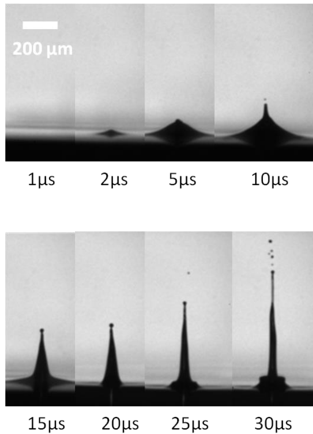
Fig. 1 : Experimental images of LIFT temporal evolution ( t=0 corresponds to the laser pulse). Focalization objective Numerical Aperture is 0.26 and the laser is an IR femtosecond laser (800 fs). The bioink is 10% glycerol (v/v) + 15 mg/ml BSA and the laser energy is 24 \mu\text{J} . At 2 \mu\text{s} there is a bubble formation, then until 5 \mu\text{s} the bubble is growing. The bubble collapse and jet formation are occurring from 10 to 15 \mu\text{s} . From 15 to 30 \mu\text{s} the jet is growing until its break off into droplets at 30 \mu\text{s} .
