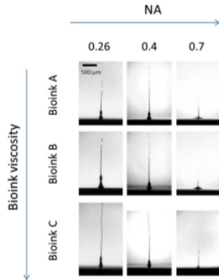
Fig. 5. Influence of the NA on the bioprinting jet for a laser pulse of 10 \mu\text{J} . TRI images of jet at h_{\text{max}} for the different bioinks with respect to NA.
