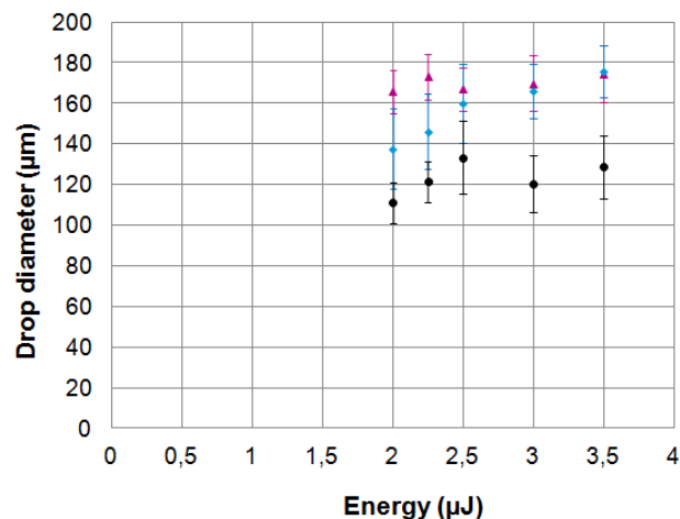
Figure 4. Printed drop diameter versus laser pulse energy.
