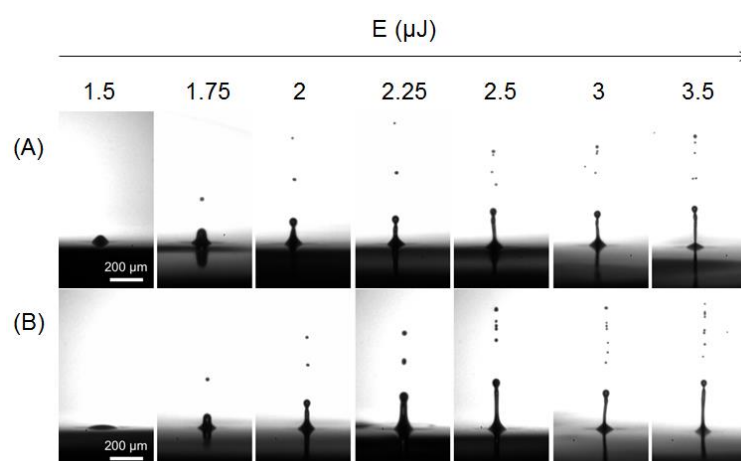
Figure 5. Time resolved imaging of the hydrodynamic interaction of the jet with laser, observed 90 \mu\text{s} after the laser pulse arrival, as a function of laser energy. Results are presented for bioinks without cells: A and B.
