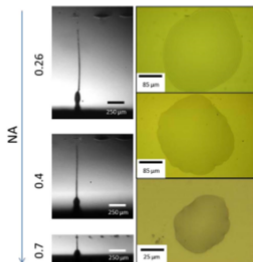
Fig. 6. Influence of the NA on the bioprinting jet for a laser pulse of 10 \mu\text{J} . TRI images of jet with a receiver (left) and images of the corresponding bioprinted drops (right) for bioink B.
