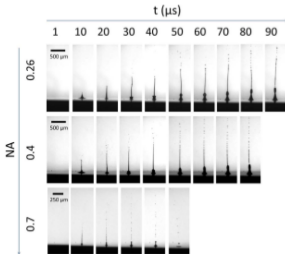
Fig. 4. Influence of the NA on the bioprinting jet for a laser pulse of 10 \mu\text{J} . Temporal evolution of the jet for bioink B for NA = 0.26 to 0.7.
