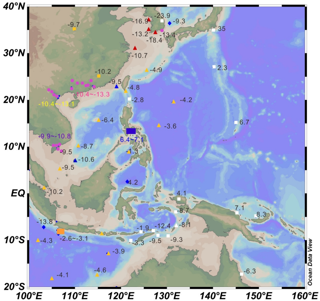
Fig 1.17. Map showing the distribution of sea surface water \epsilon Nd values from the SCS and the surrounding marginal seas (orange triangle). \epsilon Nd values of surface sediment and sediments from Asian rivers in the SCS and the surrounding marginal seas have also been included for comparison. Red triangles represent Korean and Yellow river sediments samples; blue diamonds represent core-top samples; yellow rectangles represent loess samples; white rectangles represent rocks samples; pink dots represent Pearl River/Mekong River/Red River sediments samples; blue triangles represent dust samples; blue rectangles represent Philippine river sediments samples. Data are from GEOROC database: http://georoc.mphmainz.gwdg.de/georoc/ , Liu et al. (2007), Goldstein et al. (1984), Goldstein and Jacobsen (1988), Amakawa et al. (2000).
