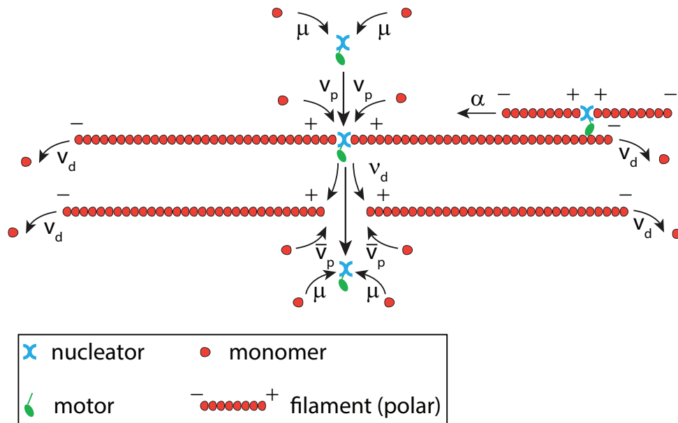
FIGURE 4.30: Schematic representation of the model. Nucleator nucleate two filaments with a rate \mu , giving rise to a bipolar filament. The filaments are attached with their (+)-ends to the nucleator and grow on this end with a speed v_p . They depolymerize at the (-)-end with a speed v_d . Bipolar filaments detach from the nucleator with a rate of \nu_d . Their polymerization speed at the (+)-end is then lowered to \bar{v}_p . Myosin is attached to formin. It moves towards the (+)-end of filaments. Its activity is denoted as \alpha . The figure was prepared by Karsten Kruse and is shown with slight modifications.
