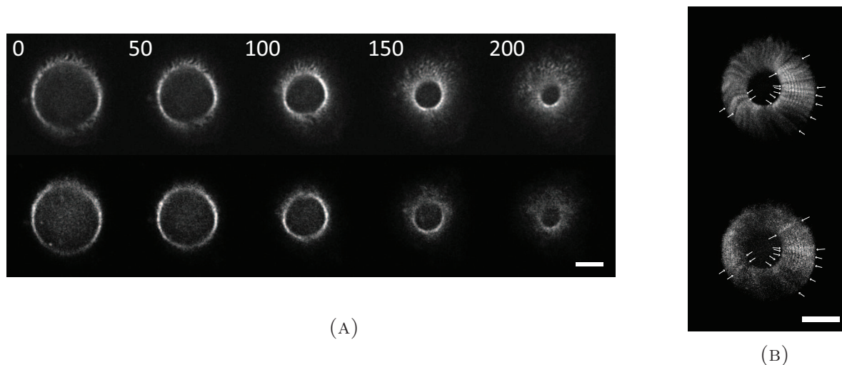
FIGURE 4.23: (A) Timelapse of a closing ring labeled in myosin (top) and mDia2 (bottom). Time in s, scale bar 5\ \mu\text{m} . (B) Overlay of 17 subsequent time frames (top: myosin, bottom: mDia2). mDia clusters move mainly radially. The comparison with the corresponding myosin pattern, show that formin colocalizes with myosin. Time between images 10 s, scale bar 5\ \mu\text{m} .
