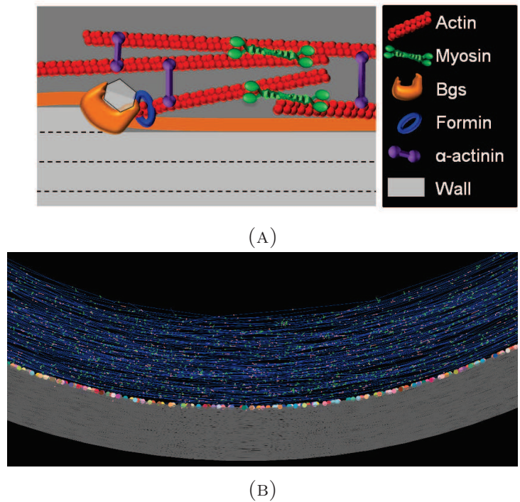
FIGURE 5.14: (A) Scheme of the simulated model. The ring is composed of actin, myosin and \alpha -actinin. The wall synthesis machinery (Bgs) is connected to actin nucleators (formin). (B) Representation of the Cytosim simulation. Nodes (various colors) are attached to the membrane and build the wall (grey) after being displaced. They are attached to filaments (blue), which interact with crosslinkers (pink) and motors (green).
