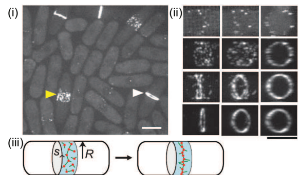
FIGURE 2.20: (i) A fission yeast culture expressing the labeled node protein Rlc1p-3GFP. Before division, nodes are distributed in a band (yellow arrow head). The cytokinetic ring is condensed (white arrow head). (ii) 3D reconstruction of cells at different stages of ring formation. Nodes are distributed in a band before they condense to a ring. (iii) Schematic representation of the search and capture model (nodes: red, actin: green). When a node “finds” the filament of a neighboring node, it pulls the other node: the ring condenses. Scale bars 5 \mu\text{m} . (Figure from [167].)
