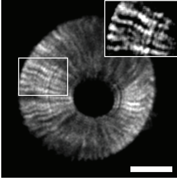
FIGURE 4.21: Overlay of 25 frames of a myosin ring. The inset shows a region of the ring, where myosin clusters split and fuse. Images are smoothed with ImageJ. Time between images 20 s, scale bar 5 \mu\text{m} .
