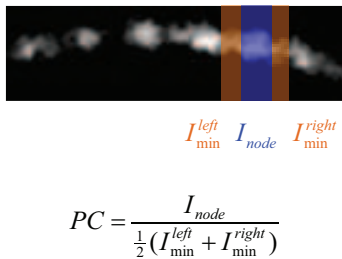
FIGURE 4.26: Schematic explanation of the definition of the pattern coefficient (PC). The PC is the ratio between the intensities of the myosin motifs and the neighbouring low intensity regions.
