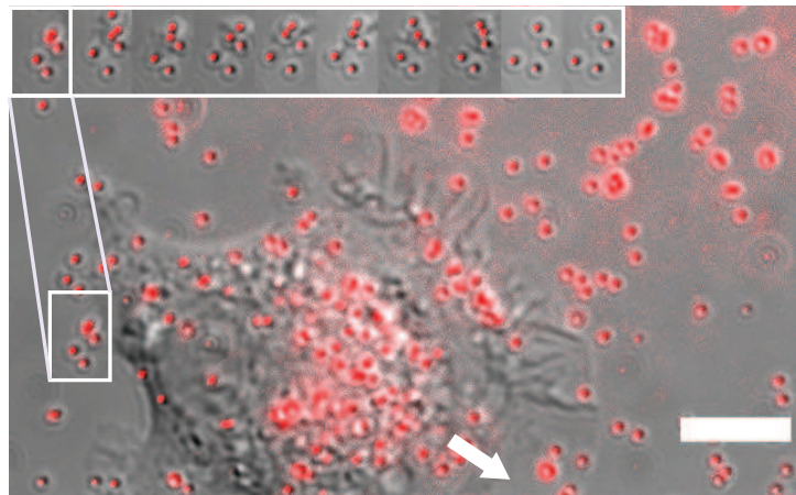
FIGURE 4.54: REF52 cell on a flat polyacrylamide gel of 10 kPa with red fluorescent beads. The cell deforms the surface and displaces the beads (inset) as it is moving to the bottom right (arrow). The inset illustrates the bead displacements. \Delta t = 15 min, scale bar 5 \mu\text{m} .
