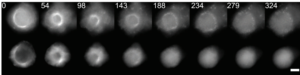
FIGURE 4.42: Timelapse of a ring after addition of Latrunculin A (top: myosin, bottom: actin). The ring continues to close and opens after about 1.5 min. Myosin reveals patches around the ring. The timelapse was acquired with an inverted epifluorescence microscope. Time in s, scale bar 5\ \mu\text{m} .
