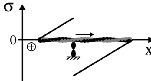
FIGURE 2.3: Displacement of filaments due to motors leads to the depicted tension \sigma profile. Filaments are considered as rigid rods being moved through a viscous medium. (Figure from [75].)
