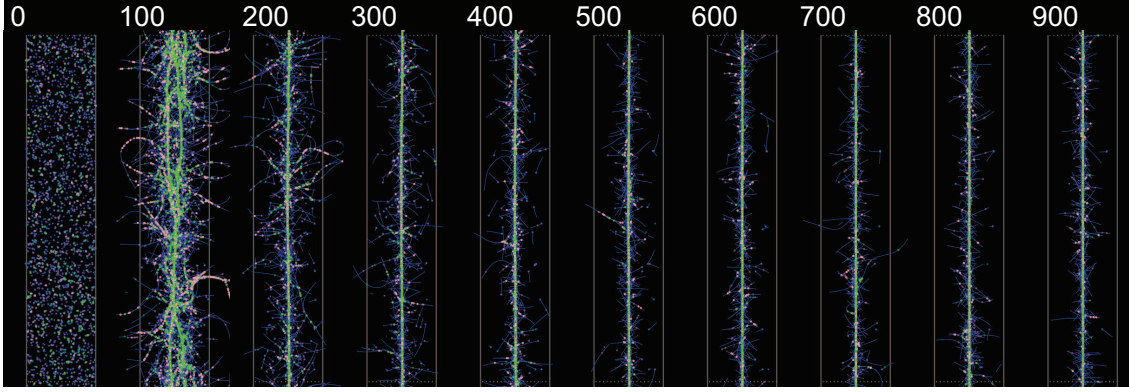
FIGURE A.20: Simulation of the condensation of the ring. The ring condenses essentially in less than 200s. Blue: actin filaments, green: myosin, pink: \alpha -actinin, time in s, the dimensions of the simulation are 1\text{ }\mu\text{m} \times 5\text{ }\mu\text{m} .
