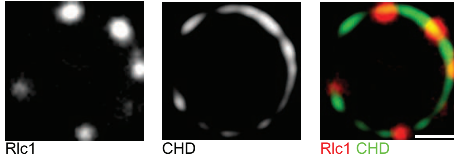
FIGURE 5.12: Overlay of 225 frames ( dt = 3\text{s} ) of CHD and Rlc1 signal of cells incubated with 10 \mu\text{M} of Latrunculin A. Rlc1 speckles are static. Actin speckles are still moving, but their location is restricted to the environment of Rlc1 speckles. Scale bar 1 \mu\text{m} .
