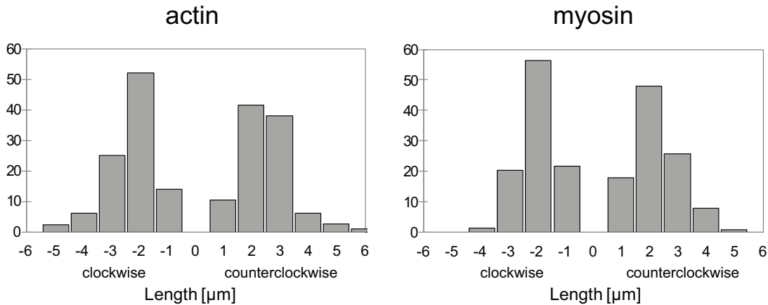
FIGURE A.22: Analysis of the rotation of actin and myosin speckles shows that motion is similar in both directions. Actin speckles move on average by 2.1 \pm 0.8\ \mu\text{m} (mean and standard deviation, n = 242 ), while myosin speckles move by 1.8 \pm 0.8\ \mu\text{m} (mean and standard deviation, n = 265 ).
