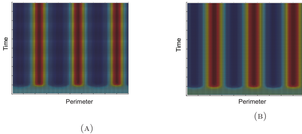
FIGURE 4.31: Solution of the set of differential equations describing the density changes. The concentrations are color coded and presented as kymographs, as a function of the position on the ring and the time. (A) shows the distribution of filaments in the ring and (B) the distribution of motors. For a critical myosin activity, in both cases a periodic pattern forms from an initially homogeneous distribution of material. The peaks of both distributions are centered around the same values.
