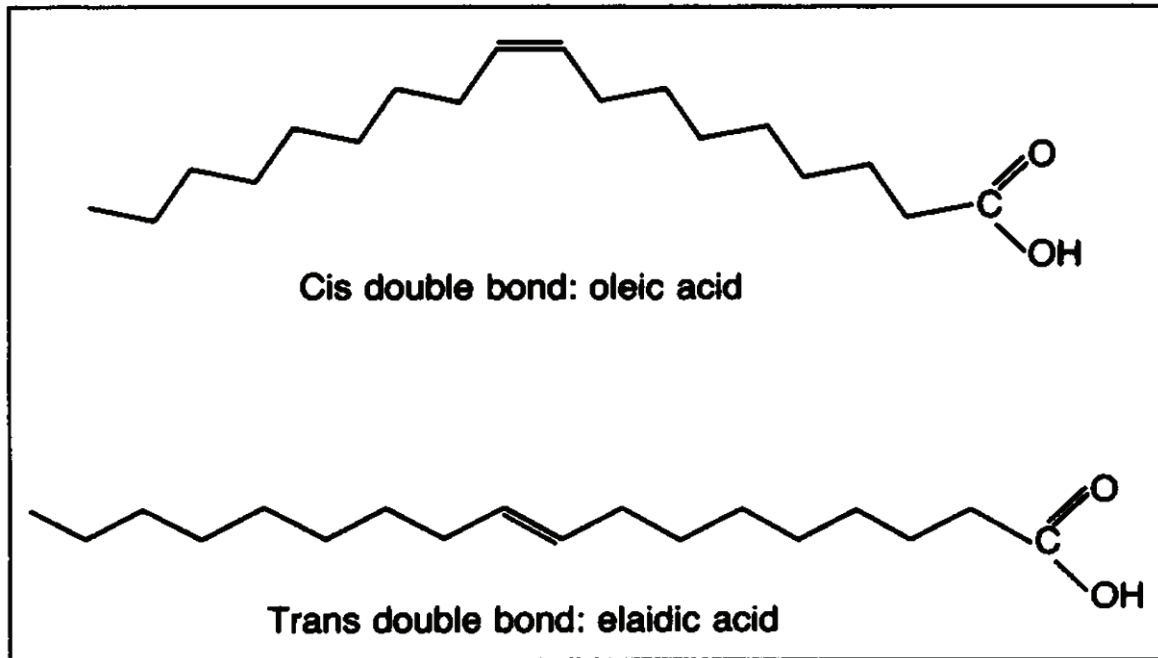
Figure 15 Trans fatty acids structure of oleic acid and elaidic acid (Mensink and Katan 1990).
