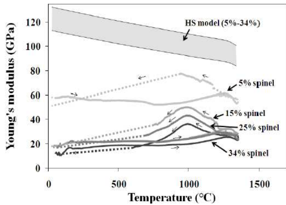
Figure IV-3: Evolution of the Young's modulus vs. temperature of the MSp composites with a spinel grain size of 1-3 mm and different spinel inclusion contents (Grasset-Bourdel, 2011)
