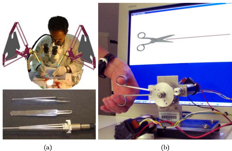
Figure 4.3: The haptic user interfaces for training in virtual environment: (a) The micro-surgery-training working scenario of the haptic tweezers and its comparison to real tweezers [Burdet 2004]. (b) The haptic scissors [Okamura 2003].
