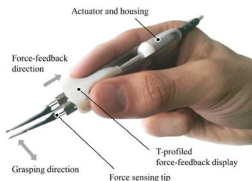
Figure 4.4: The haptic tweezers of the project NeuroArm for robotic surgery [Rizun 2006b].
