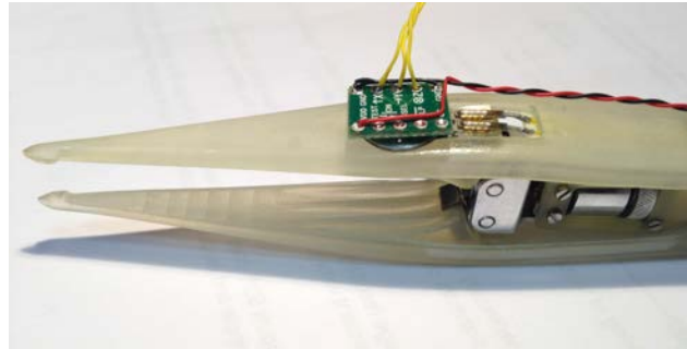
Figure 4.24: Accelerator setup to measure the bandwidth of the Télétweez.
