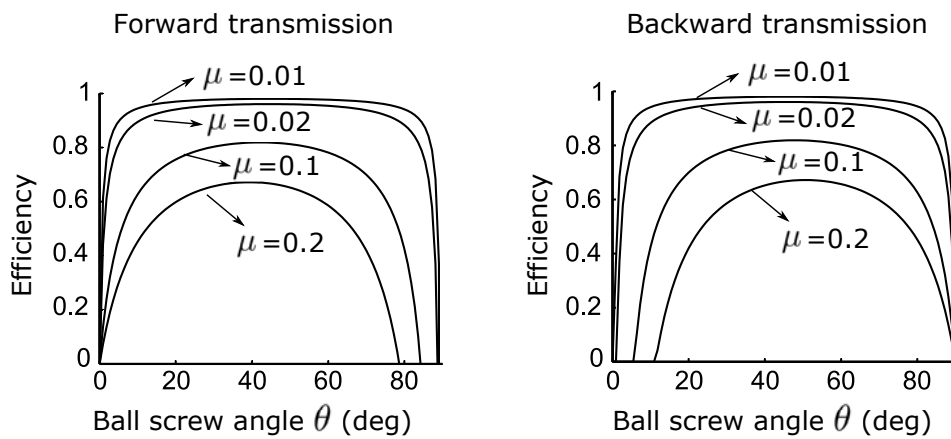
Figure B.2: Ball screw transmission efficiency.
