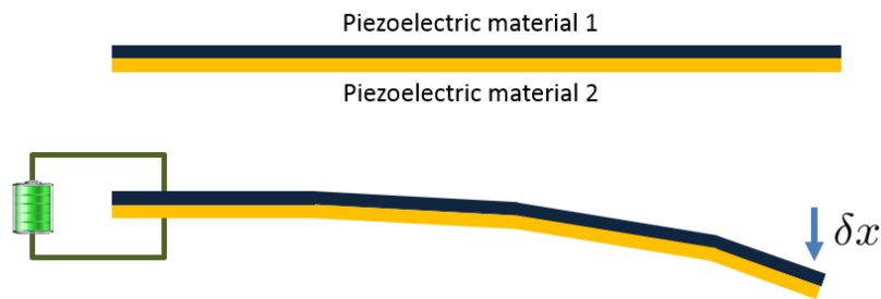
Figure 1.17: Bimorph actuator. With input power conditions being opposite to the upper layer and to the lower layer, one dilate and the other contract. This finally results flexion of the entire structure. The tip can thus give rise to net displacement and output force.
