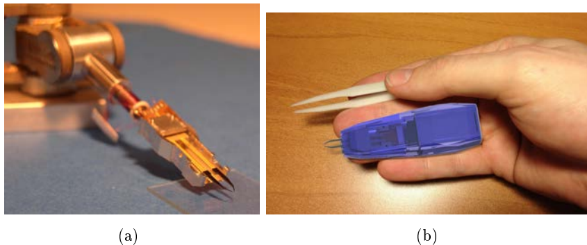
Figure 1.14: (a) PiezoGripper mounted on a miniature robotic arm; (b) Fully integrated PiezoGripper.
