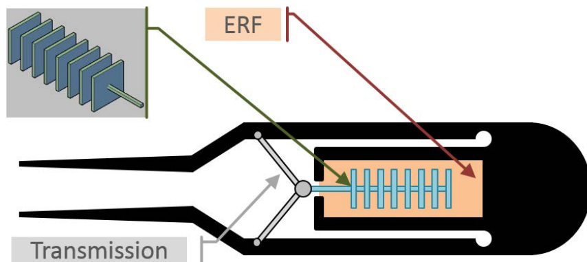
Figure 4.13: The actuator system concept with piston filled with ERF.
