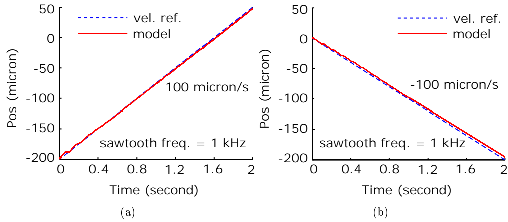
Figure 2.19: Velocity control simulation with partial dynamic model. The sawtooth frequency is set to 1 kHz. The speed reference is set to 100 micron/s for both forward and backward motion.
