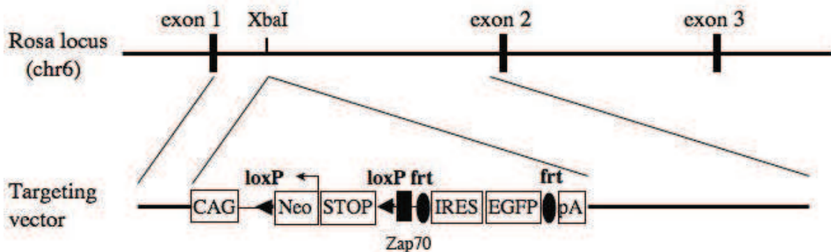
Figure 30. Zap70 mouse coding sequence cloning into CTV vector construct that will permit in insertion of conditionally expressed gene into mouse ROSA26 locus (see text).
