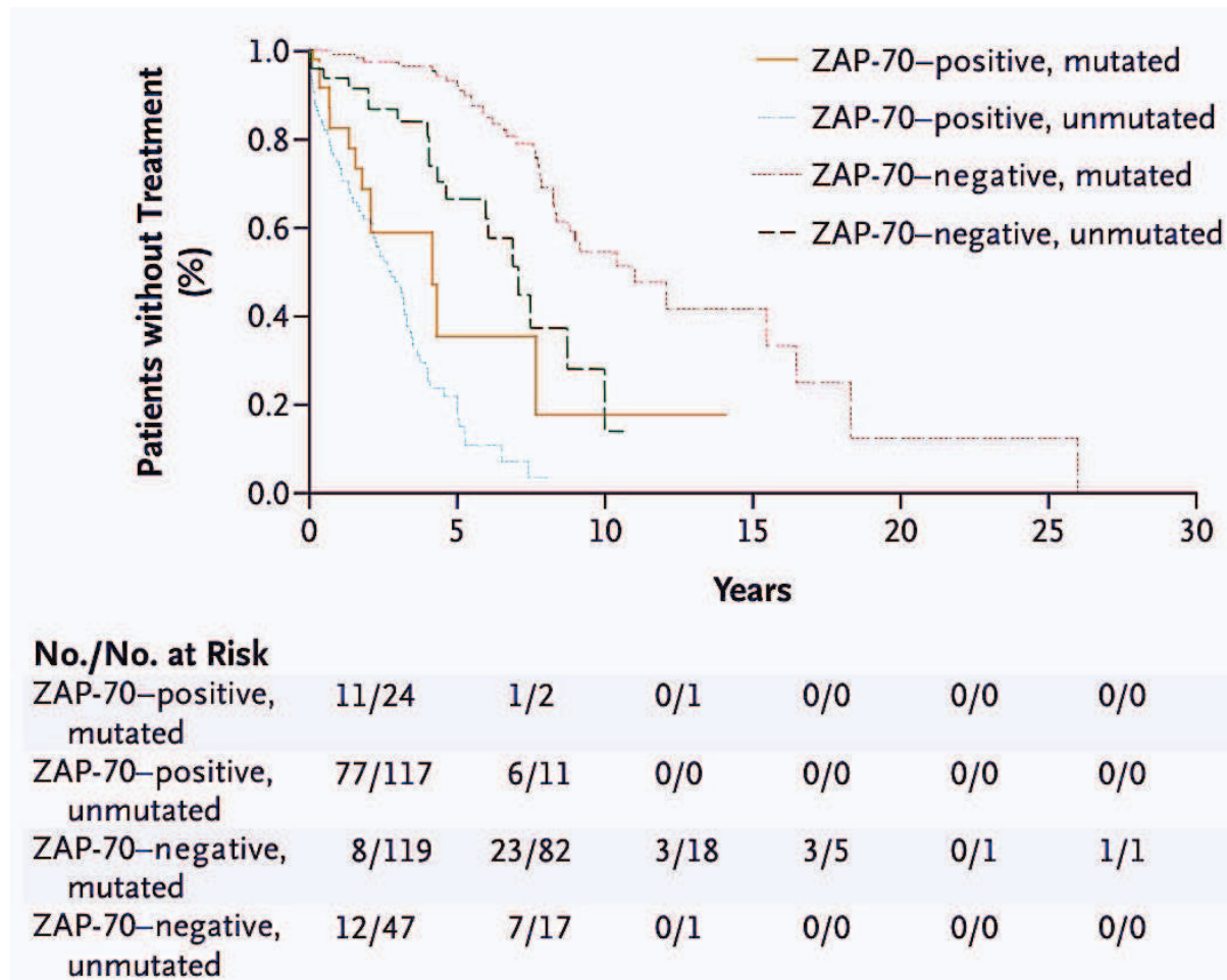
Figure 14. Relationship between ZAP-70 expression, IGHV mutational status, and the time from diagnosis to initial treatment. Kaplan-Meier curves depict the proportion of untreated patients with CLL according to the time since diagnosis (Rassenti et al. 2004).
