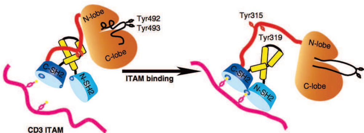
Figure 28. Model for the activation of ZAP-70 following ITAM binding (Wang et al. 2010).
