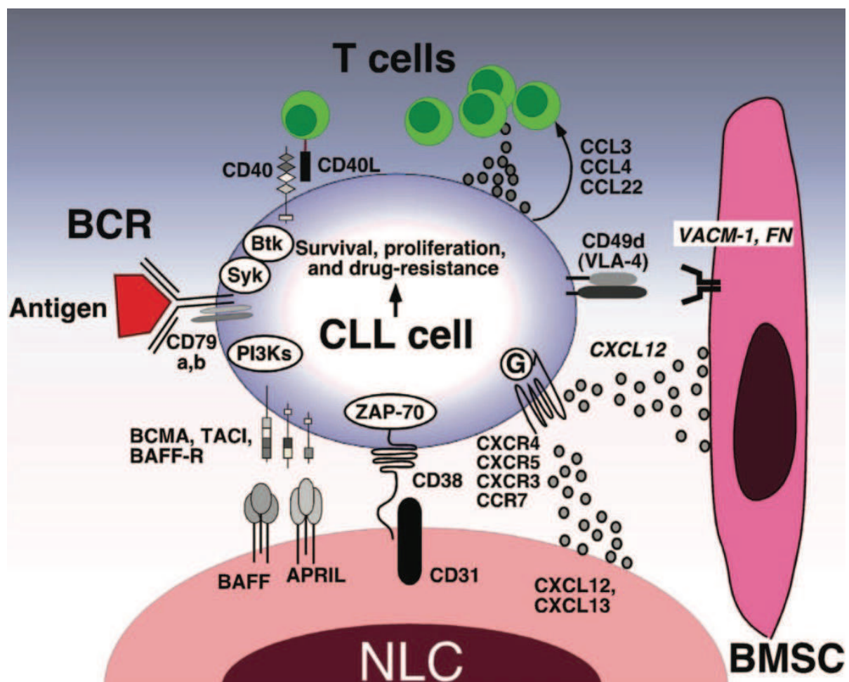
Figure 7. CLL microenvironment (Burger 2011).
