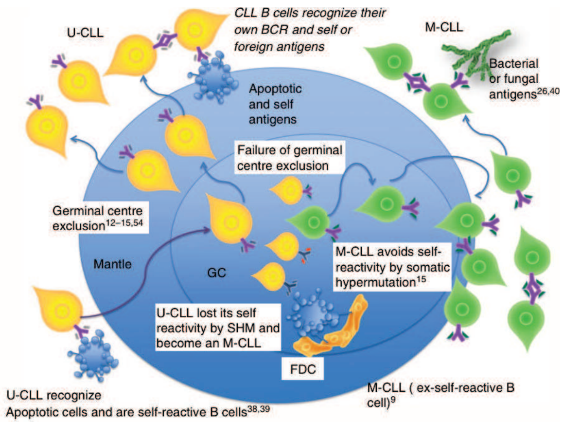
Figure 4. Tolerance mechanisms in the germinal center possible involved in CLL pathogenesis.
