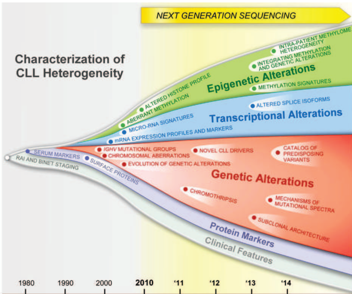
Figure 9. Evolution and growth of our understanding of CLL heterogeneity over time (Gruber and Wu 2014).
