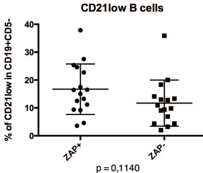
Figure 52. Percentage of CD21 low in ZAP-70 + vs. ZAP-70 - normal CD19 + CD5 - B cells from CLL patients in flow cytometry (unpaired t test).
