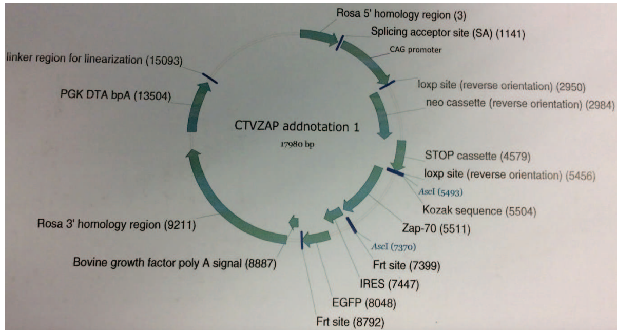
Figure 31. CTVZAP addnotated vector, used to generate conditional Zap70 KI mice by homologous recombination into embryonic stem cells of Zap70 loxP into Rosa site.
