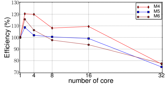
(f) Assembly efficiency (weak scalability)
