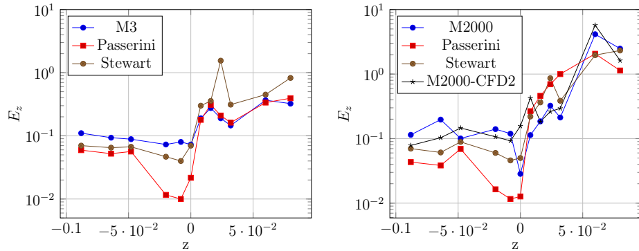
(a) Validation metric E_z , Re_t = 500 (b) Validation metric E_z , Re_t = 2000
