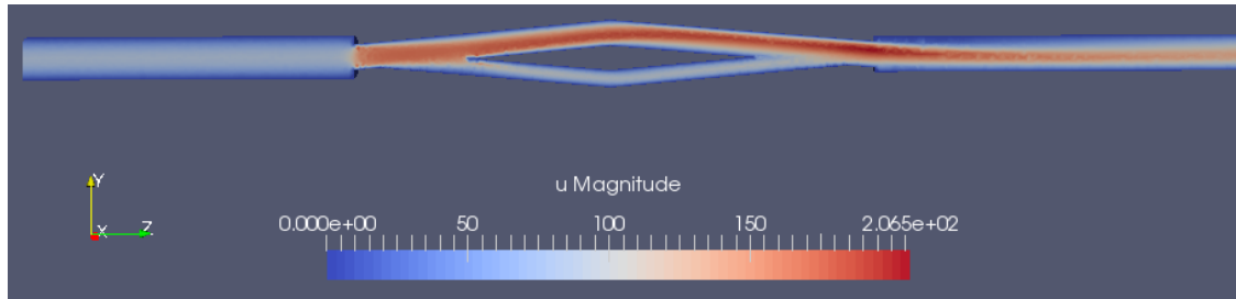
FIGURE 14. Velocity magnitude, M3 mesh, constant flow.
