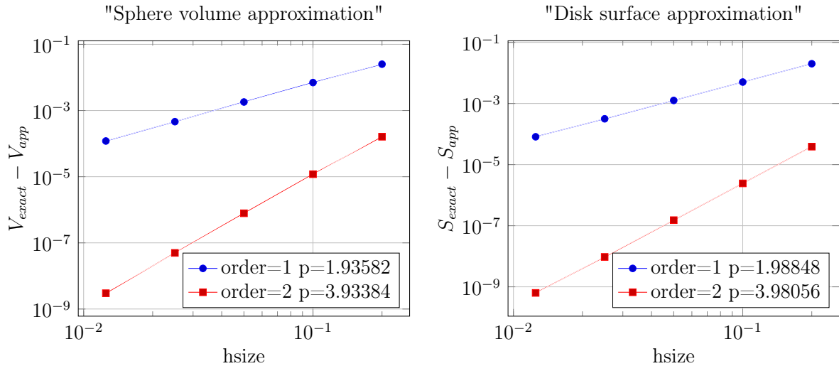
Figure 1.6: High order geometry approximation: error plots for |\int_{\Omega} 1 - \int_{\Omega_h} 1| , \Omega being a sphere (left) and a disk (right).
