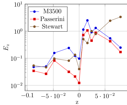
(c) Validation metric E_z , Re_t = 3500
