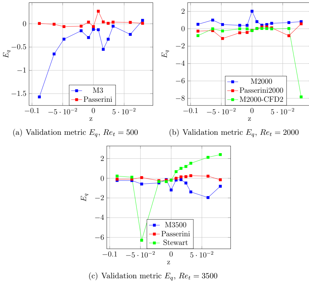
Figure 7.17: Comparison of mass error metric E_Q (Eq 7.6) as a function of the position along the z axis with respect to Passerini et al. CFD data for (a) Re_t = 500 , (b) Re_t = 2000 and (c) Re_t = 3500 .
