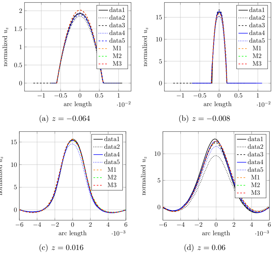
Figure 7.7: Comparison between experimental data profiles of the normalized axial velocity (Eq 7.5), for Re_t = 500 .
