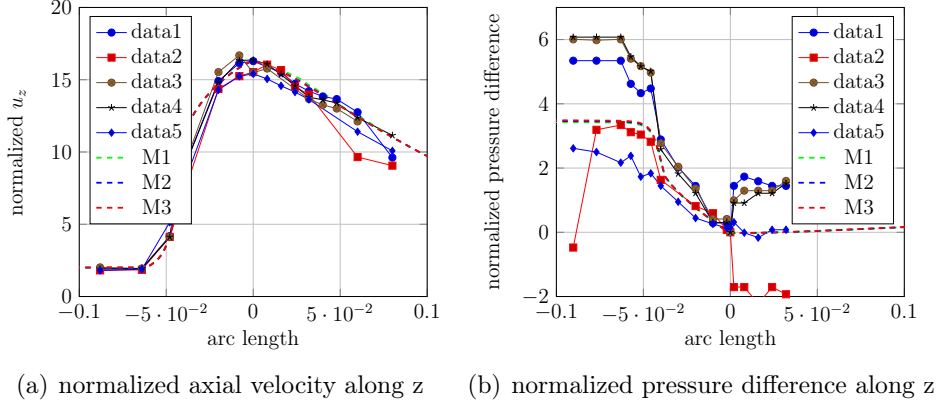
Figure 7.6: (a) Comparison between experimental data and numerical results for the normalized axial velocity along z (Eq 7.5) and (b) the normalized pressure difference along z (Eq 7.4), for Re_t = 500 .
