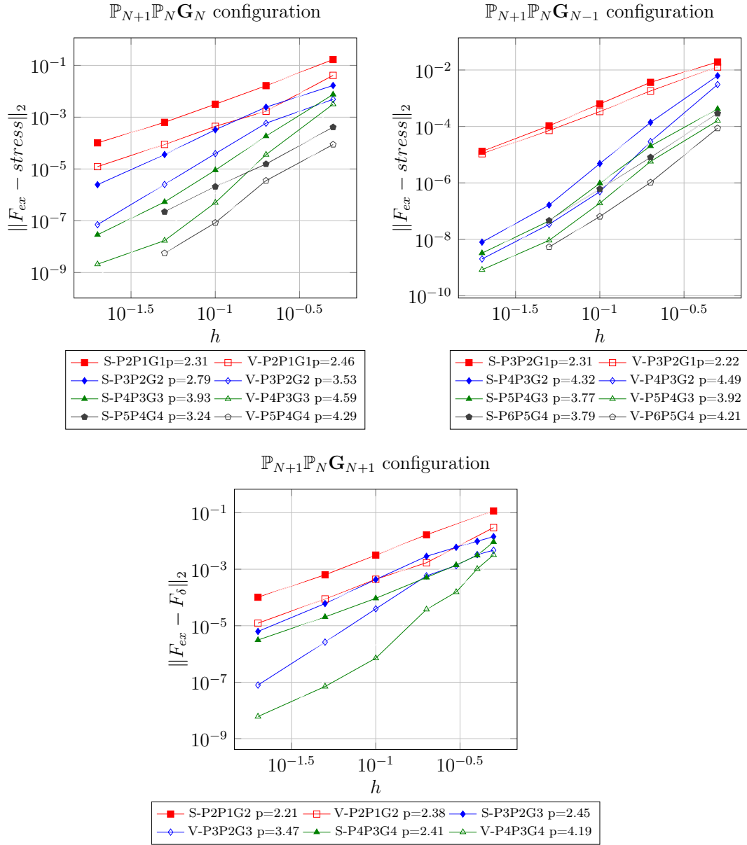
Figure 6.10: Convergence analysis for the \mathbb{P}_{N+1}\mathbb{P}_N\mathbf{G}_N , \mathbb{P}_{N+1}\mathbb{P}_N\mathbf{G}_{N+1} and \mathbb{P}_{N+1}\mathbb{P}_N\mathbf{G}_{N-1} configurations on a curved boundary.
