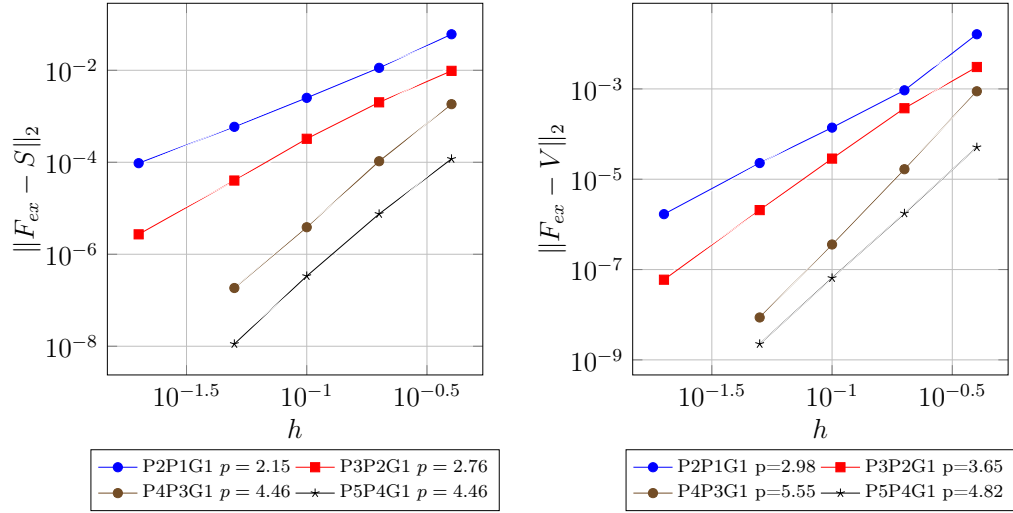
Figure 6.6: Convergence analysis for the \mathbb{P}_{N+1}\mathbb{P}_N\mathbf{G}_1 configuration on a straight boundary.
