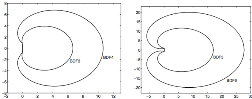
Figure 2.1: BDF absolute stability contours.[116]
