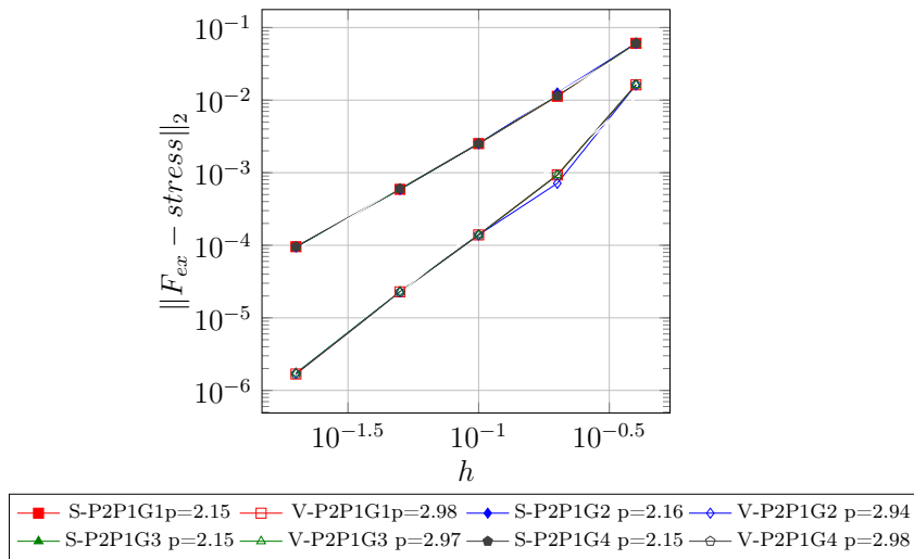
Figure 6.7: Convergence analysis for the \mathbb{P}_2\mathbb{P}_1\mathbf{G}_N configuration on a straight boundary.
