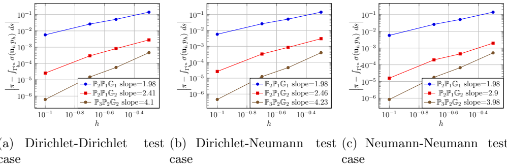
Figure 6.3: F_\delta convergence using \mathbb{P}_{N+1}\mathbb{P}_N G_N , N = 1, 2 approximations and \mathbb{P}_2\mathbb{P}_1 G_2 approximation.
