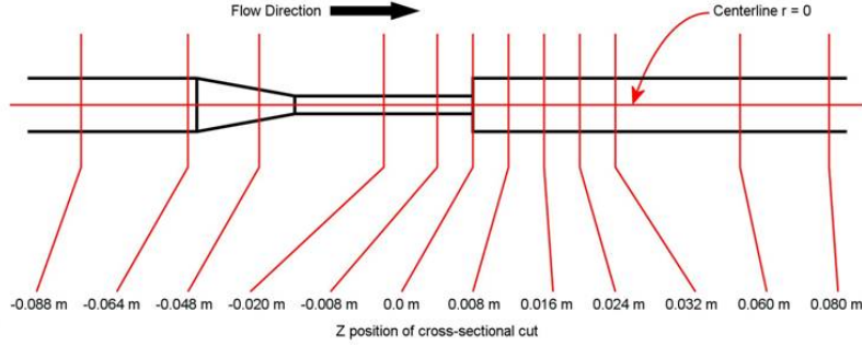
Figure 7.3: Radial sections at which the numerical results are compared with experimental data.
