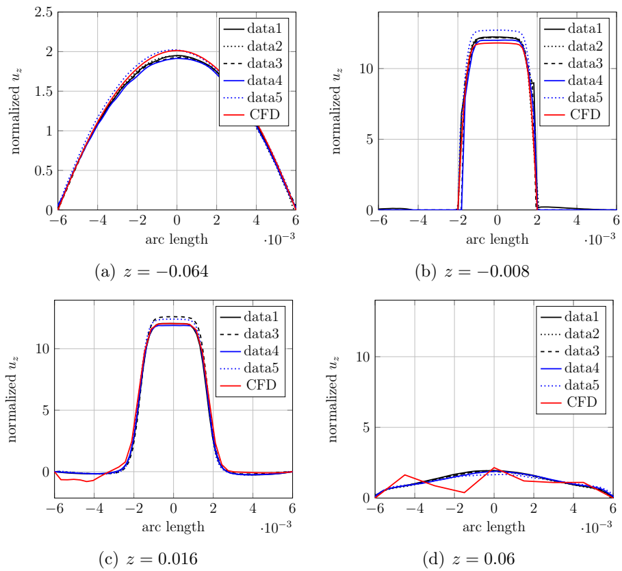
Figure 7.14: Comparison between CFD data and experimental data profiles of the normalized axial velocity (Eq 7.5), for Re_t = 3500 .
