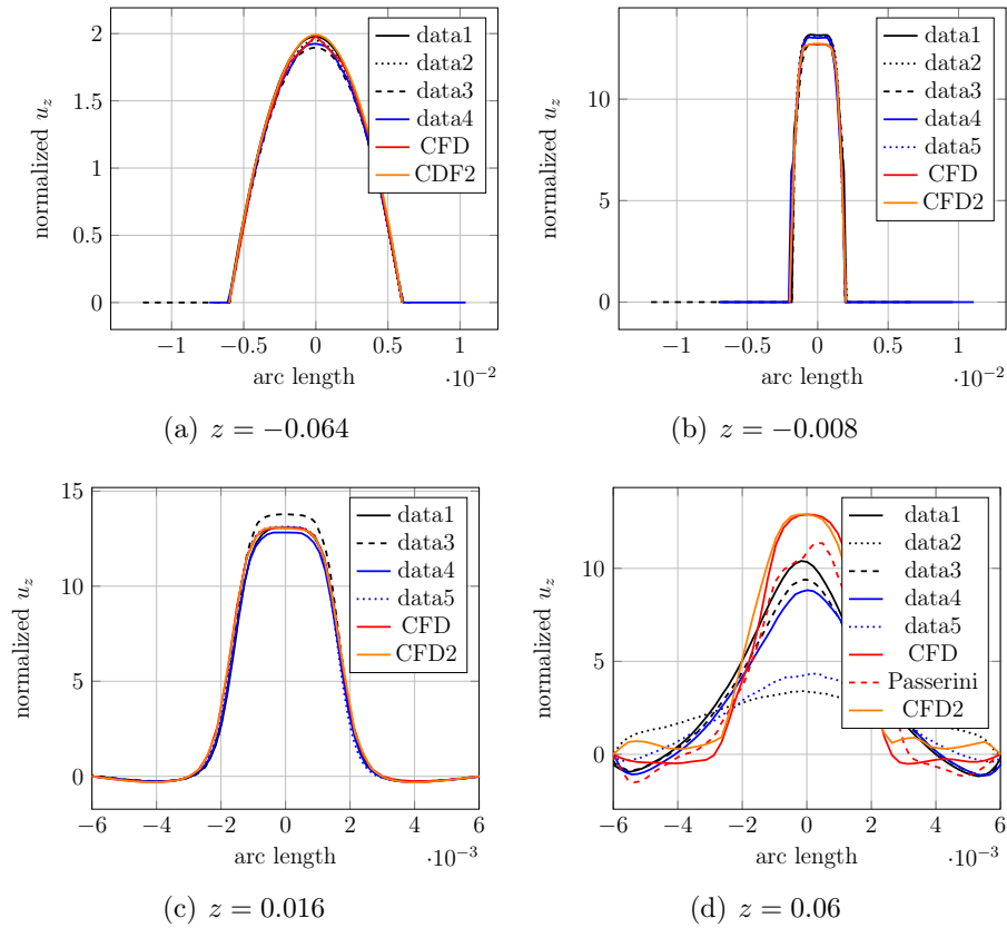
Figure 7.12: Experimental data profiles vs CFD data profiles of the normalized axial velocity (Eq 7.5), for Re_t = 2000 .
