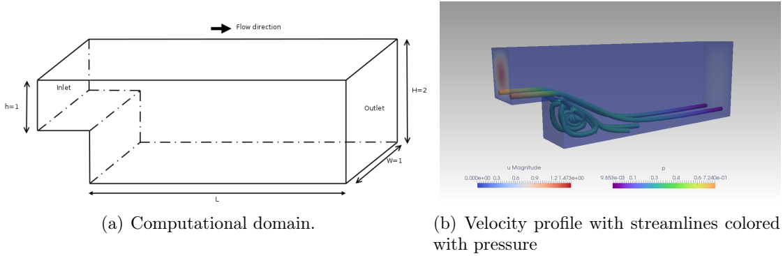
Figure 7.1: Computational domain and velocity profile with streamlines.
