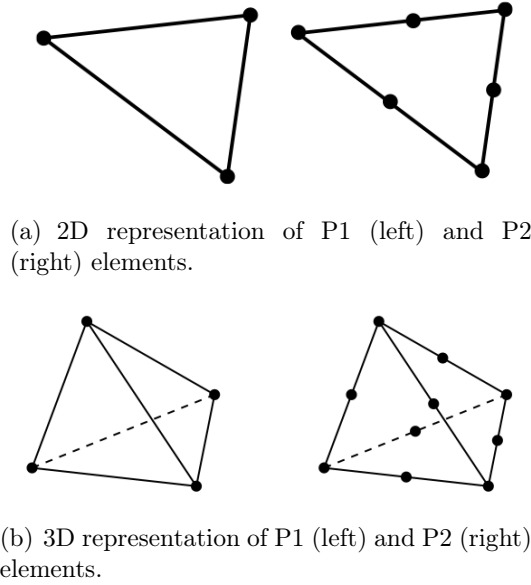
Figure 1.2: Element representation in 2D and 3D. [49]
