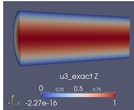
Figure 5.6: Reconstructed 3D velocity field of the exact Poiseuille velocity.
