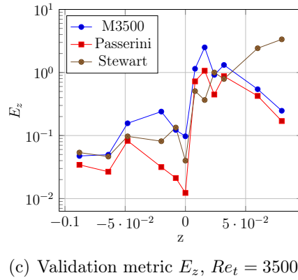
Figure 7.16: (a) Comparison of the E_z metrics (Eq (7.7)) with respect to Passerini et al. and Stewart et al. data in semi-logarithmic scale for Re = 500 , (b,c) Comparison of the E_z metrics with respect to Passerini et al. and Stewart et al. data in semi-logarithmic scale for Re = 2000 and Re = 3500 , respectively.
