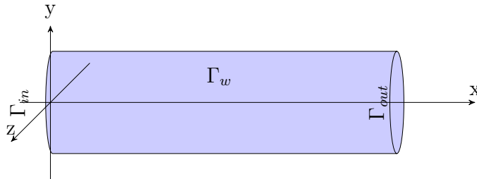
Figure 6.1: Geometry for convergence rates verification \Omega
