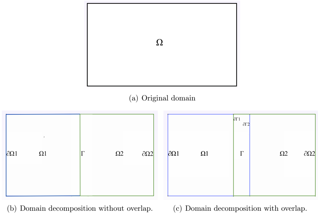
Figure 3.1: Decomposition of a 2D domain.
