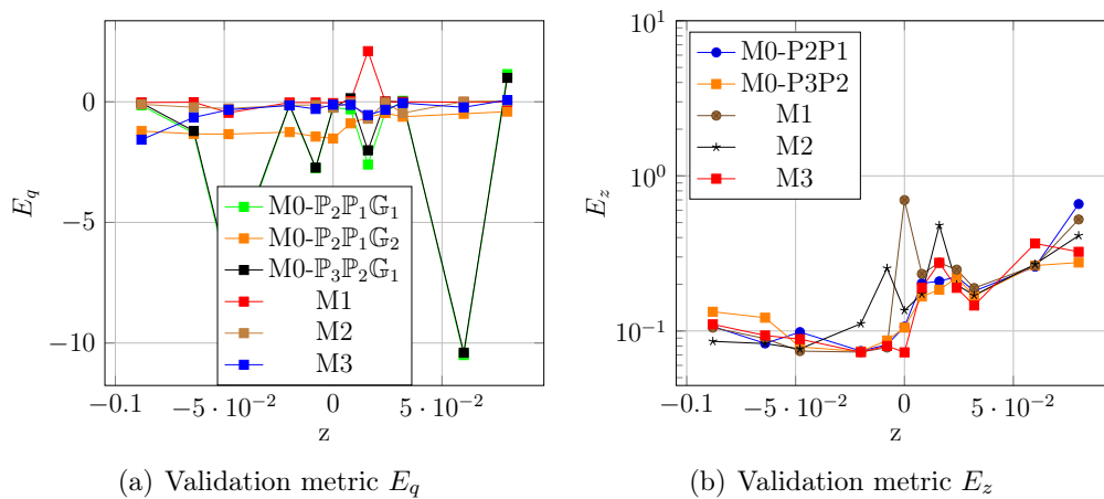
Figure 7.18: Validation metrics E_z (Eq (7.7)) and E_Q ((7.6)) for Re = 500 for the different mesh refinements
