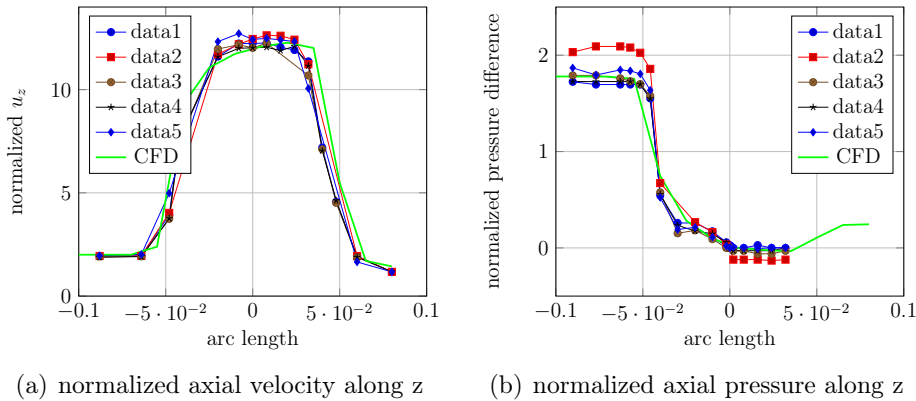
Figure 7.13: (a) Experimental data vs numerical results for the normalized axial velocity along z (Eq 7.5) and (b) the normalized pressure difference along z (Eq 7.4) for Re_t = 3500 .
