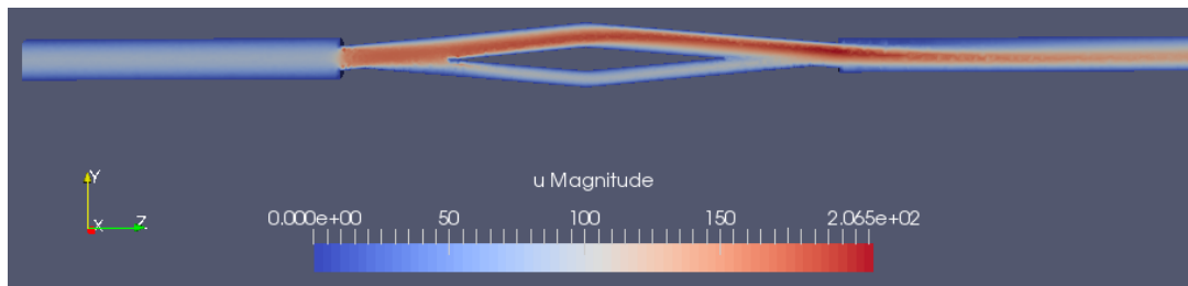
FIGURE 14. Velocity magnitude, M3 mesh, constant flow.
