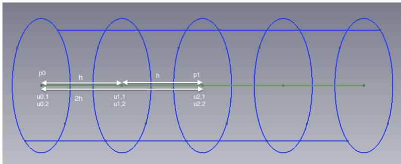
Figure 5.5: Velocity mesh of length h and pressure mesh of length 2h .
