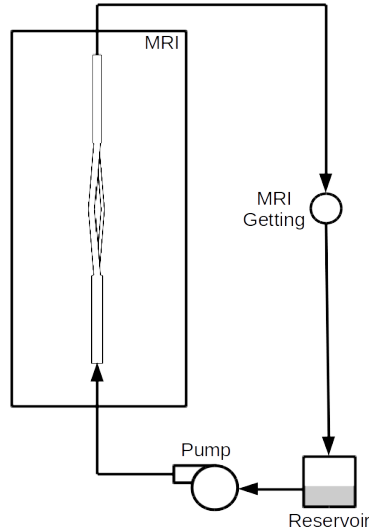
FIGURE 8. MRI benchmark.
