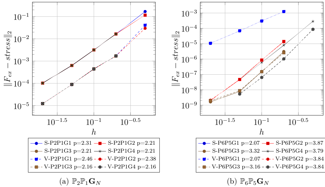
Figure 6.9: Convergence analysis for the \mathbb{P}_2\mathbb{P}_1\mathbf{G}_N and \mathbb{P}_6\mathbb{P}_5\mathbf{G}_N configurations on a curved boundary.
