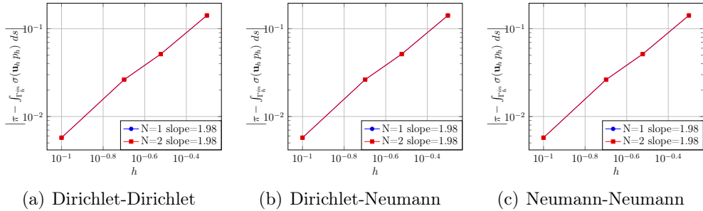
Figure 6.2: Output convergence using \mathbb{P}_{N+1}\mathbb{P}_N\mathbb{G}_1 approximation spaces, N = 1, 2 .
