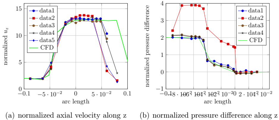
Figure 7.9: (a) Comparison between experimental data and numerical results for the normalized axial velocity along z (Eq 7.5) and (b) the normalized pressure difference along z (Eq 7.4) for Re_t = 2000 .
