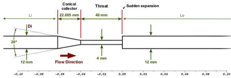
Figure 7.2: Geometry description.
