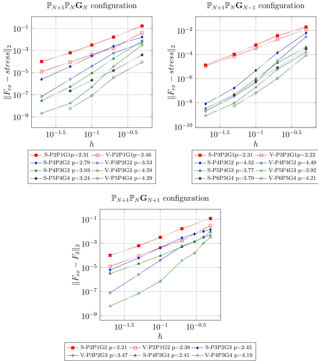
Figure 6.10: Convergence analysis for the \mathbb{P}_{N+1}\mathbb{P}_N\mathbf{G}_N , \mathbb{P}_{N+1}\mathbb{P}_N\mathbf{G}_{N+1} and \mathbb{P}_{N+1}\mathbb{P}_N\mathbf{G}_{N-1} configurations on a curved boundary.
