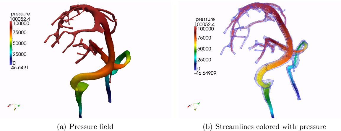
Figure 6.4: Numerical solution on the cerebrovenous system at time t = 0.00151 s.
