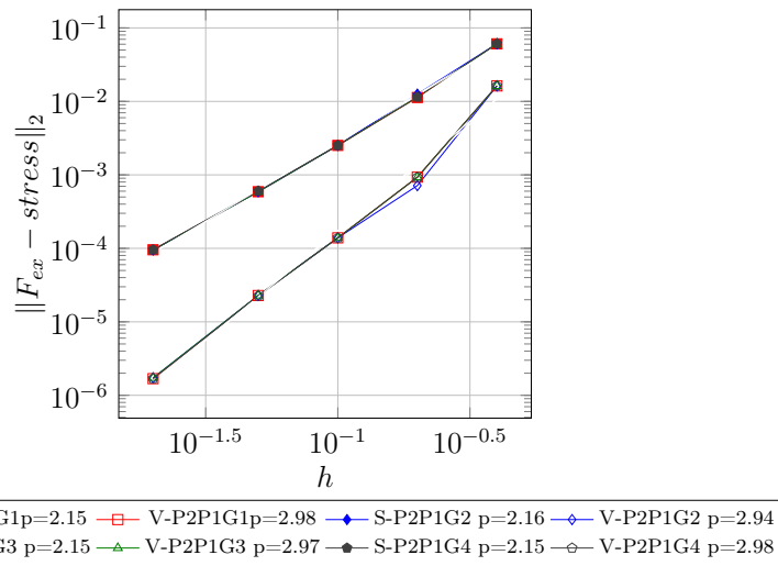
Figure 6.7: Convergence analysis for the \mathbb{P}_2\mathbb{P}_1\mathbf{G}_N configuration on a straight boundary.
