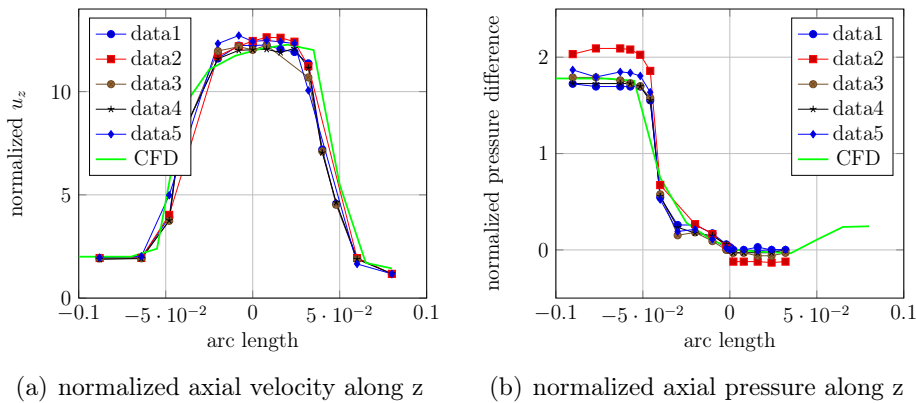
Figure 7.13: (a) Experimental data vs numerical results for the normalized axial velocity along z (Eq 7.5) and (b) the normalized pressure difference along z (Eq 7.4) for Re_t = 3500 .
