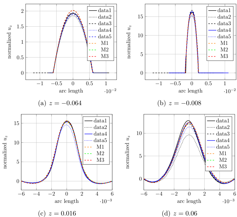
Figure 7.7: Comparison between experimental data profiles of the normalized axial velocity (Eq 7.5), for Re_t = 500 .
