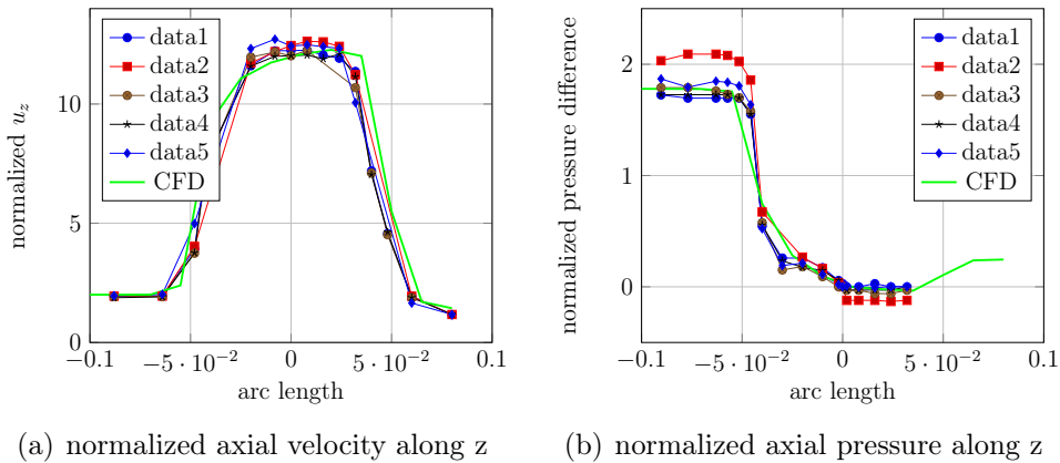
Figure 6.13: (a) Experimental data vs numerical results for the normalized axial velocity along z (Eq 6.5) and (b) the normalized pressure difference along z (Eq 6.4) for Re_t = 3500 .
