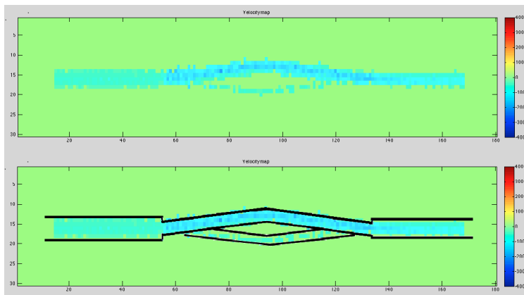
FIGURE 23. Above: Same image as Fig. 22, filtered with its corresponding magnitude image. Below: The filtered velocity map matches well with the initial phantom geometry, but we can notice a lack of particles in the lower branch.
