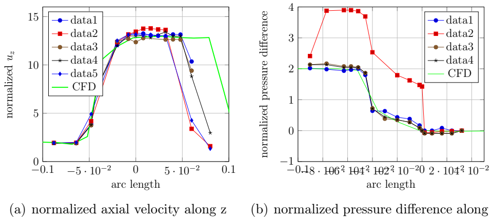
Figure 6.9: (a) Comparison between experimental data and numerical results for the normalized axial velocity along z (Eq 6.5) and (b) the normalized pressure difference along z (Eq 6.4) for Re_t = 2000 .
