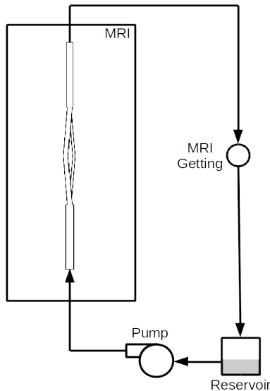
FIGURE 8. MRI benchmark.
