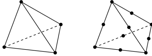
(b) 3D representation of P1 (left) and P2 (right) elements.
