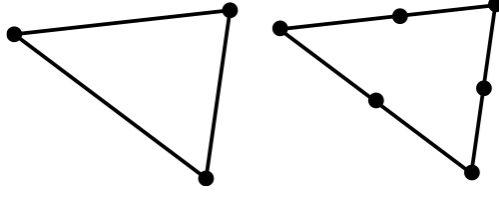
(a) 2D representation of P1 (left) and P2 (right) elements.
