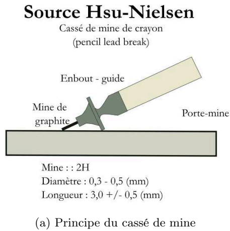
FIGURE C2: Cassé de mine HSU-Nielsen
