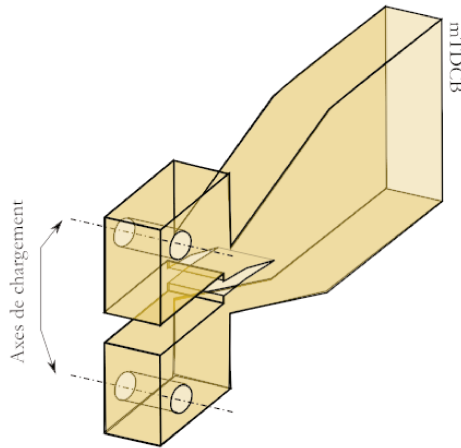
FIGURE 1.25: Eprouvette mTDCB
