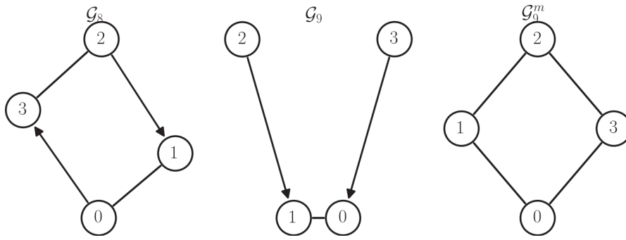
Figure 1.9 – Remarkable mixed graphs. Graph \mathcal{G}_8 is a mixed cyclic graph since it contains the directed 4-cycle 0, 3, 2, 1, 0. Graph \mathcal{G}_9 , which is a MAG , contains one u-shape inducing the immorality (2, 3). Graph \mathcal{G}_9^m , the moral graph of \mathcal{G}_9 , is not chordal as the immorality (2, 3) in \mathcal{G}_9 induced the addition of edge (2, 3) in comparison to its undirected version.
