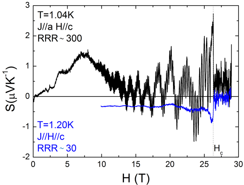
Figure 5.14: Isothermal thermopower measurements, S(H)|_{T=ctn} , at high magnetic fields for transverse (black) and longitudinal (blue) configurations at temperatures around T \sim 1\text{K} .
