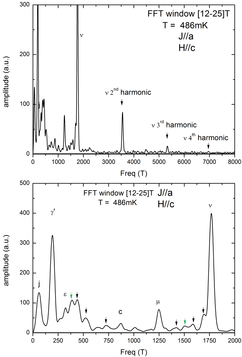
Figure 5.16: Spectrum of the AF_2 phase of CeRh_2Si_2 for a FFT window of [12 - 25]T obtained from isothermal thermopower measurements performed at T = 486\text{mK} . In the upper panel we show the main frequency \nu and its harmonics and in the down panel a zoom of the first harmonics of the AF_2 phase. The orbits of CeRh_2Si_2 are indicated by dHvA names and by arrows (new frequencies).
