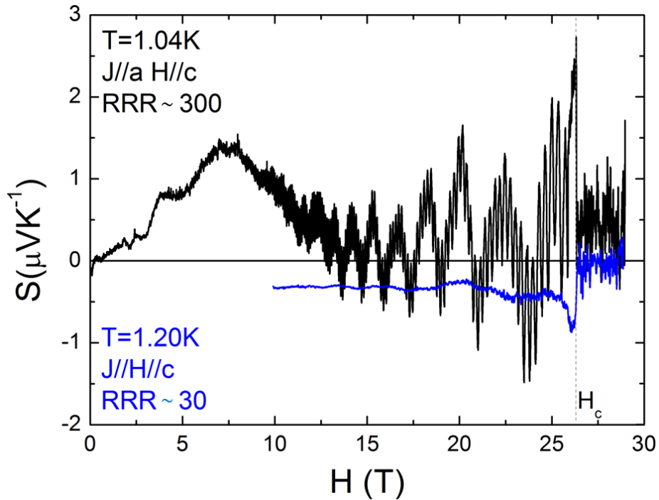
Figure 5.14: Isothermal thermopower measurements, S(H)|_{T=\text{ctn}} , at high magnetic fields for transverse (black) and longitudinal (blue) configurations at temperatures around T \sim 1\text{K} .
