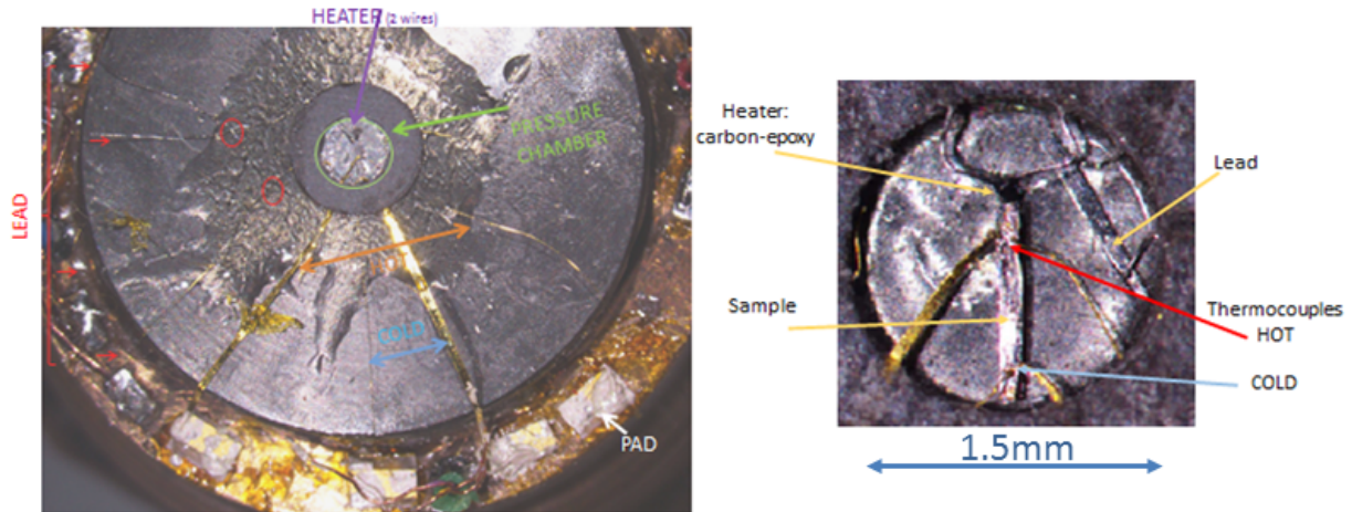
Figure 2.5: Photo of a real setup in a Bridgman Pressure Cell. Thermocouples, heater, manometer, pressure chamber and pad are indicated by legends and colored arrows. A zoom of the pressure chamber and its different components are shown on the right figure.
