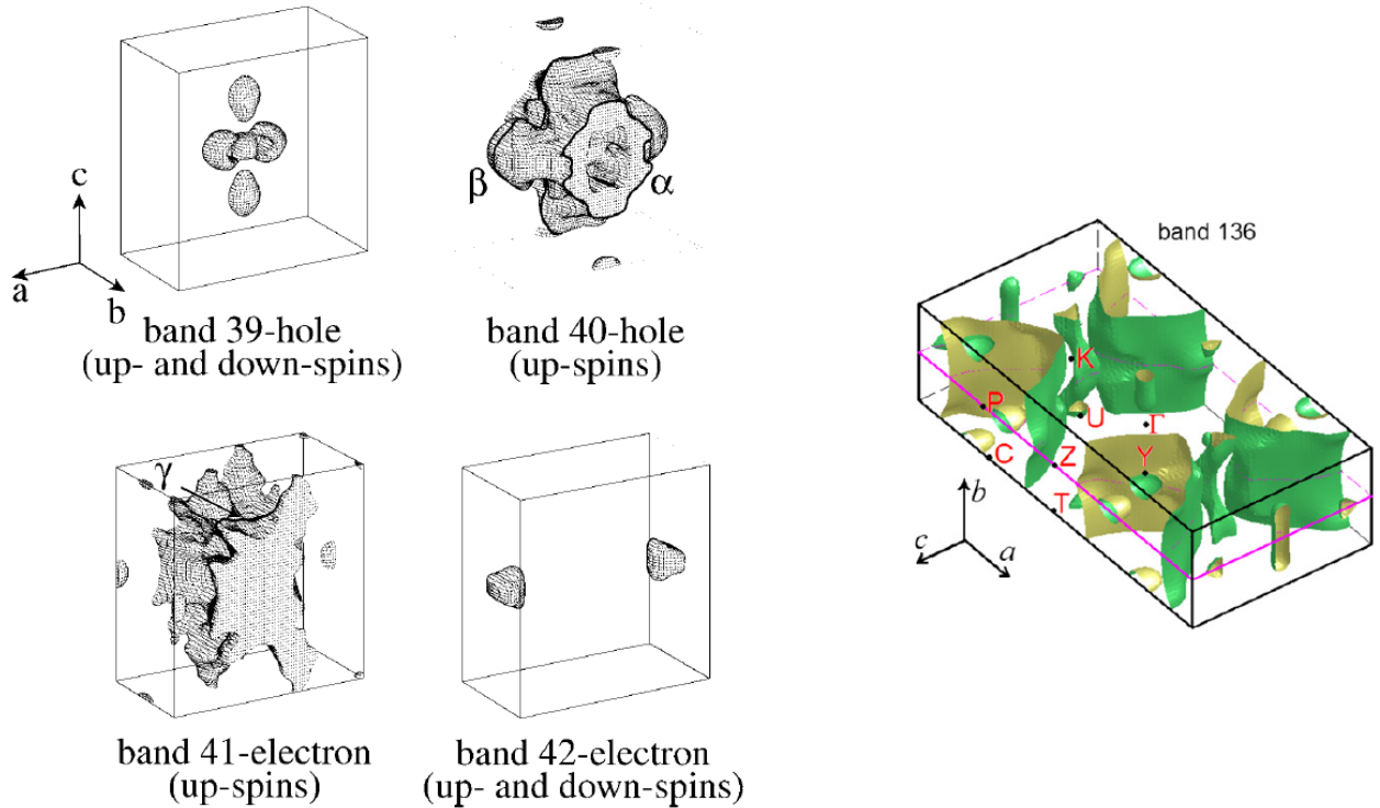
Figure 4.4: Degenerated Fermi surfaces of the FM2 phase of UGe_2 obtain by LAPW method [Settai et al., 2002] (on the left). FM2 Fermi surface of UGe_2 calculated by LSDA approach [Samsel-Czekala et al., 2011] (on the right).
