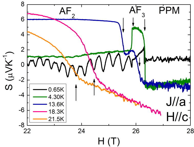
Figure 5.23: Evolution of the metamagnetic transitions, AF_2 - AF_3 and AF_3 -PPM, at high magnetic fields for the transverse configuration obtained from S(H) measurements.
