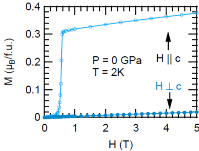
Figure 3.5: UCoAl magnetization measurements as a function a magnetic field applied along the c -axis (open circles) and on the basal plane (filled circles) at T = 2K .
