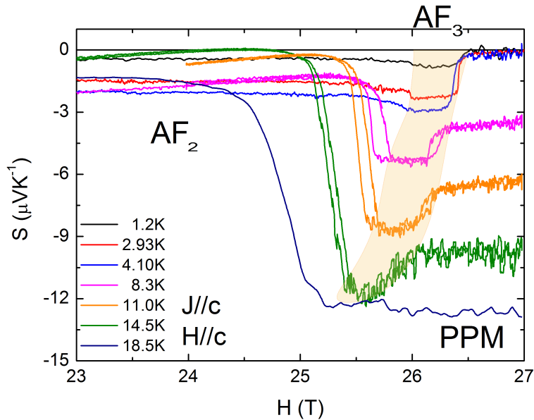
Figure 5.24: S(H) measurements at high fields for longitudinal configuration. The metamagnetic transitions, AF_2 - AF_3 and AF_3 -PPM, at high field are shown. The orange area shows the evolution of the AF_3 phase.
