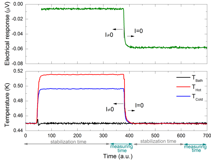
Figure 2.6: Temperatures and Seebeck voltage as a function of time for the vacuum stable conditions acquisition.
