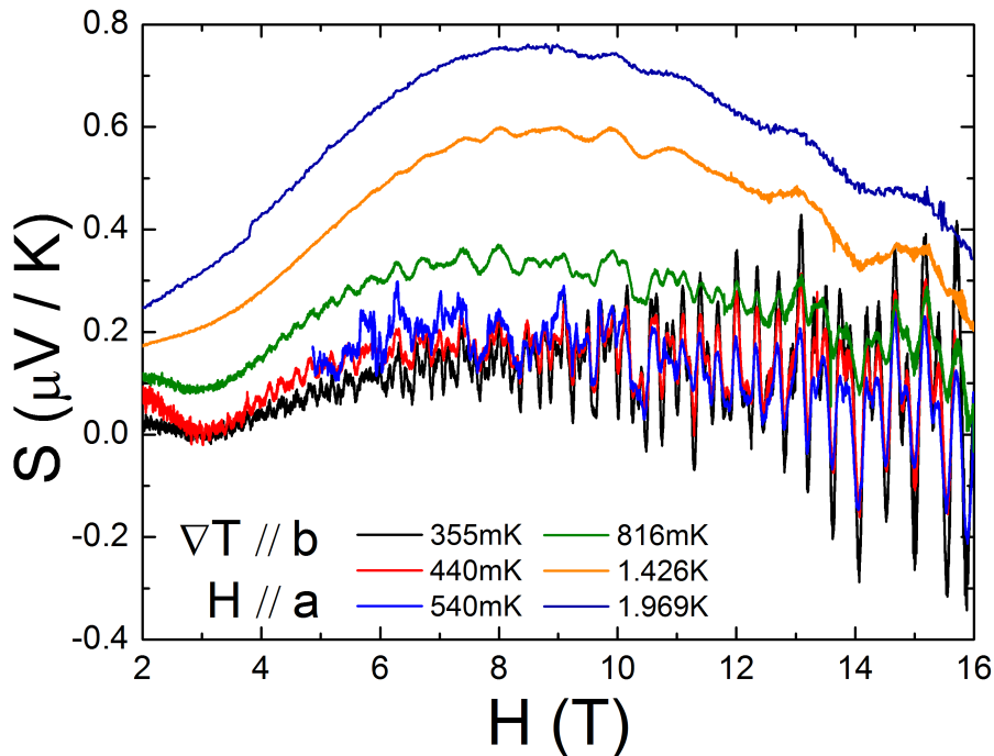
Figure 4.10: UGe_2 isothermal thermopower measurements with applied thermal gradient along the b -axis and magnetic field along the a -axis performed at different temperatures. Thermopower quantum oscillations are observed in the low temperature regime [0 – 2]K.
