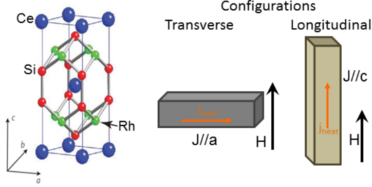
Figure 5.6: CeRh_2Si_2 crystallographic structure is represented on the left figure. Transverse and longitudinal measuring configurations are shown on the middle and on the right figures, respectively.
