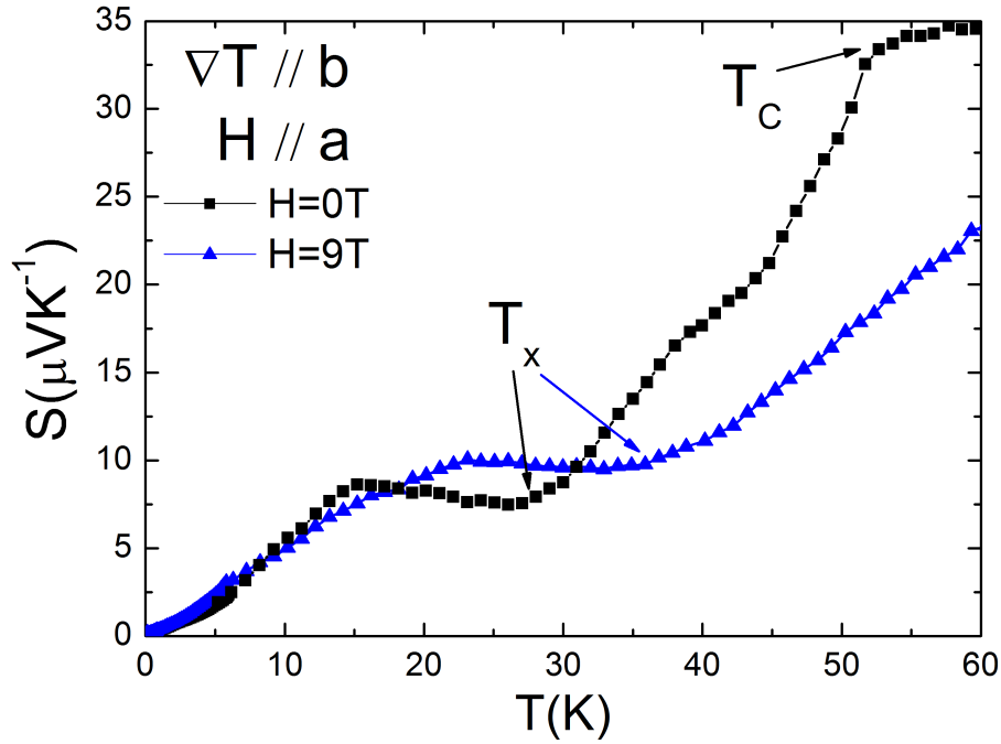
Figure 4.6: Thermopower measurements as a function of temperature S(T) at different magnetic fields: S(T) at H = 0T (black color) and S(T) at H = 9T (blue curve).
