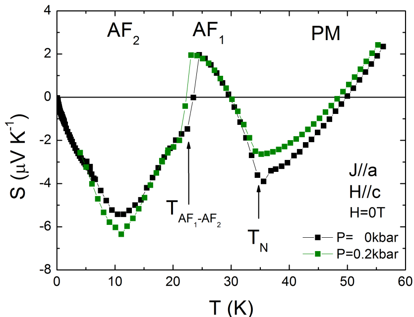
Figure 5.28: Thermopower as a function of temperature for transverse configuration at P = 0 (black curve) and P = 0.2\text{kbar} (green curve) obtained by ‘‘One heater-Two thermometers’’ and ‘‘RTG’’ techniques, respectively.
