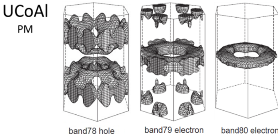
Figure 3.6: Paramagnetic Fermi surface of UCoAl obtained by FLAPW+LSDA band structure calculations (H. Harima, unpublished). This Fermi surface has one hole and two electron bands. The non inversion symmetry causes the large differences between the two electron-like bands.
