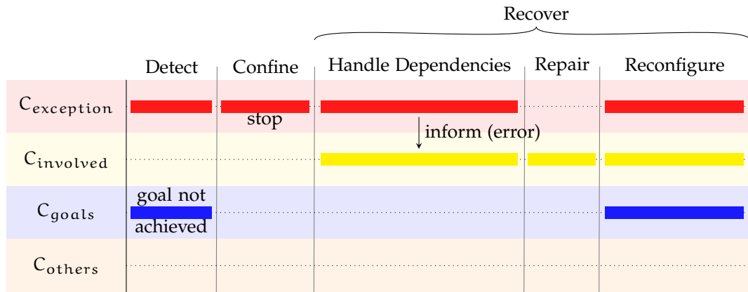
Figure 25: Involvement of components by phase of fault tolerance, with C_{\text{exception}} : the component where the uncaught error was detected, C_{\text{involved}} : components that were depending on the first one, C_{\text{goals}} : components whose detection occurred through the goal mechanism and C_{\text{others}} : other components that are not concerned, but may be eventually required to participate after the reconfiguration of the others, e.g. to compensate for another component that is no longer available.
