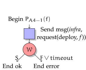
Figure 69: Plan for G_{A4} : "have functionality deployed"
