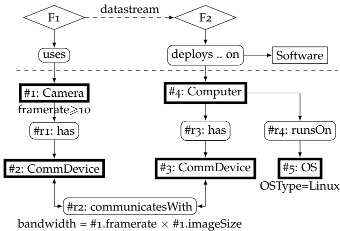
Figure 59: Example of a basic application graph
