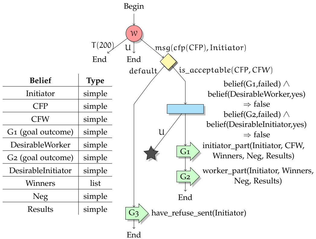
Figure 87: Main goal plan for the MC_i agents ( P_{MC_i0-1} ) - it adopts two complementary goals: one for dealing with the worker agents to whom it acts as an initiator ( G_1 ) and one for managing the initial CFP, in which case it acts as a worker ( G_2 ). The two goals G_1 and G_2 have strong links so the failure of one causes the other to stop and this is ensured by the two rules added before their adoption. “Is_acceptable(CFP, CFW)” is a predicate that returns true and instantiates CFW if local conditions are met for the MC_i to try and reply positively to the CFP (e.g. demand parameters are within acceptable limits, resources to spare etc.).
