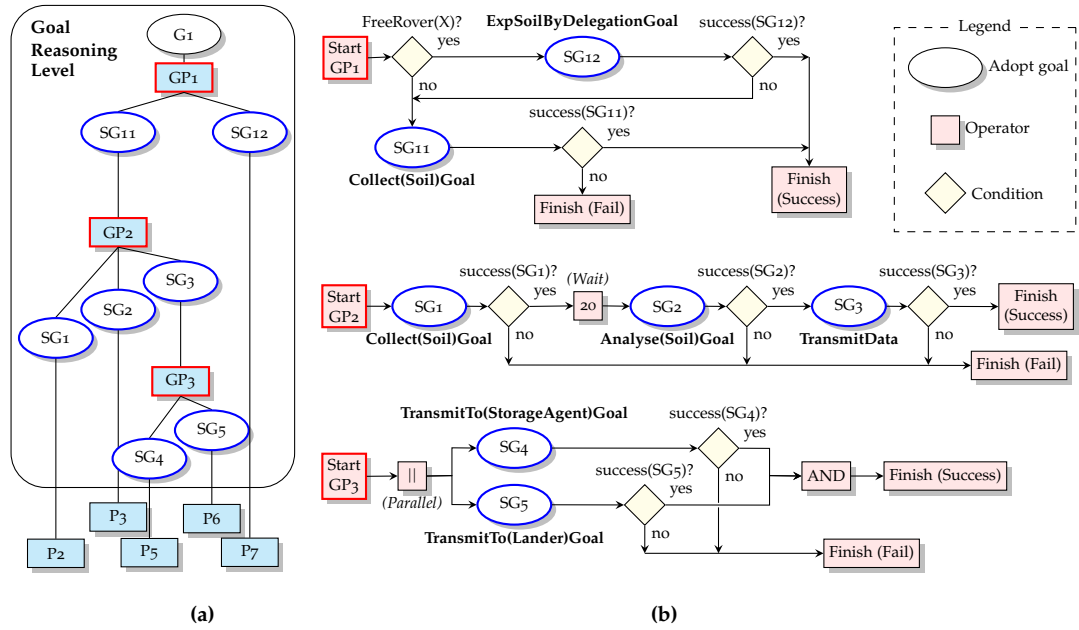
Figure 53: A multiple level goal plan for the Mars rover scenario from Fig. 49, with (a) the resulting goal-plan hierarchy (as used in Sec. 5.2 and similar to a GPT) representation and (b) the corresponding goal plans. Note the separation in (a) between the action plans, i.e. P2, P3, P5, P6 and P7, and the goal reasoning level comprising the goals and the three goal plans, i.e. GP1, GP2 and GP3.
