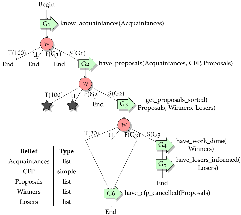
Figure 82: Plan P 10-1 - main goal plan
