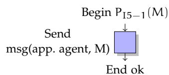
Figure 79: Plan for G_{15} : “have app. agent informed of outcome”
