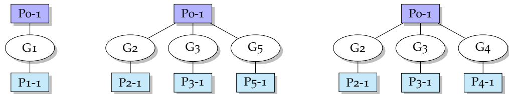
Figure 44: Goal-plan hierarchies for the worker agent in case it refuses the bid (left), it completes the task successfully (centre) or it fails to complete the task (right)
