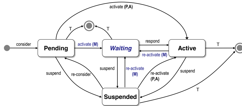
Figure 9: Goal automaton example from [111], with specific transitions depending on goal type: A - Achievement goal, P - Perform goal and M - Maintenance Goal, and T corresponding to a goal ending: drop, abort, succeed or fail.
