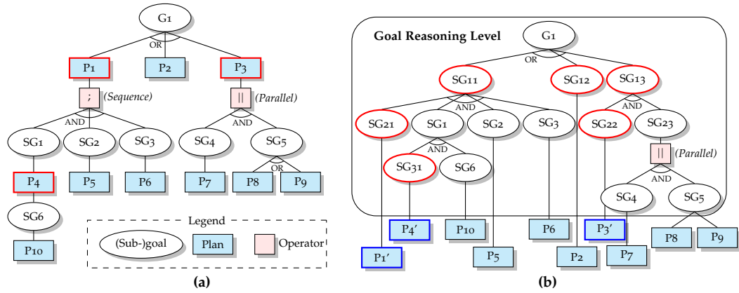
Figure 48: An example of Goal-Plan Tree (same as in Fig. 10) (a) and a Goal-Plan Separation of the same example (b)
