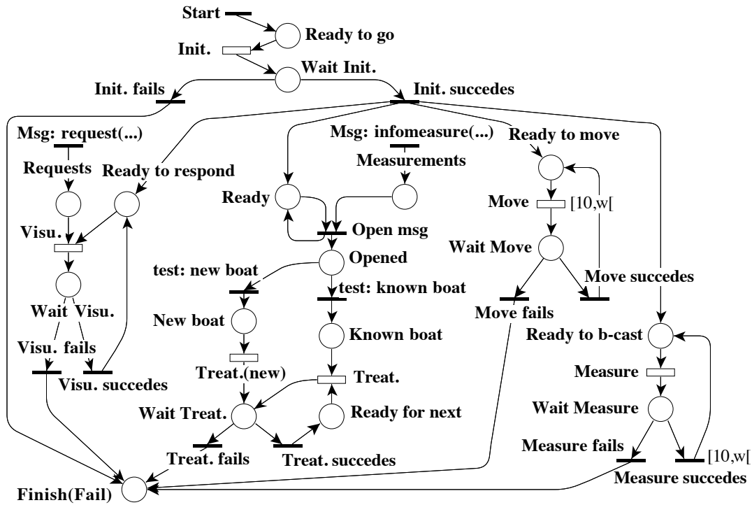
Figure 55: Petri net representation of the goal plan for the aircraft agent with goal adoptions represented as hollow transitions. The Treat. (for “treatment”) goal is adopted in two different contexts in order to insure that messages from each boat are treated sequentially, but in parallel with the other boats. Multiple instances of the goal with different beliefs are thus created.
