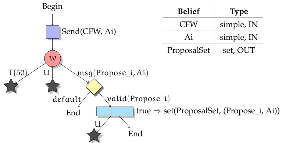
Figure 91: Plans P_{MCi1-2-1} "have proposal set" and P_{MCi1-2-1-1} "have cfw intent from one acquaintance"
