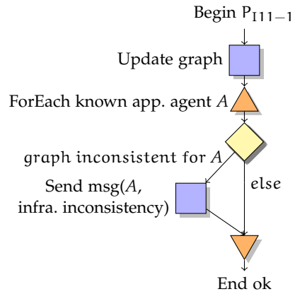
Figure 73: Plan for G_{111} : “have graph updated”
