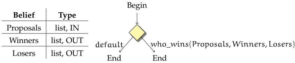
Figure 92: Plan P_{MCi1-3-1} - “get proposals sorted” simply uses an external method to sort according so some criteria and produce the two lists: Winners and Losers. The goal will fail if no Winners list is produced.
