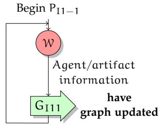
Figure 72: Plan for G_{11} : “keep infrastructure graph up to date”
