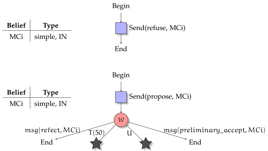
Figure 98: Plans P_{Wj1-1} “have refuse sent” and P_{Wj2-1} “have proposal sent”, whose goal is achieved if the reply is “preliminary accept”
