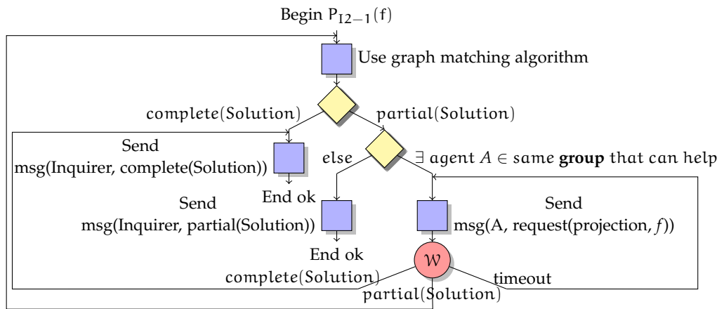
Figure 74: Plan for G_{12} : “have application projection solution”. “Inquirer” can be an Application Agent or another Infrastructure Agent .
