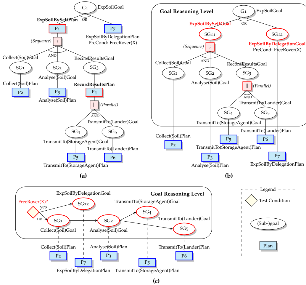
Figure 49: (a) the Goal-Plan Tree of a Mars rover from [108], (b) a translation of the Mars rover scenario in the form of a GPS-compliant AND-OR goal decomposition and (c) a modified representation of the scenario with a clear goal-plan separation
