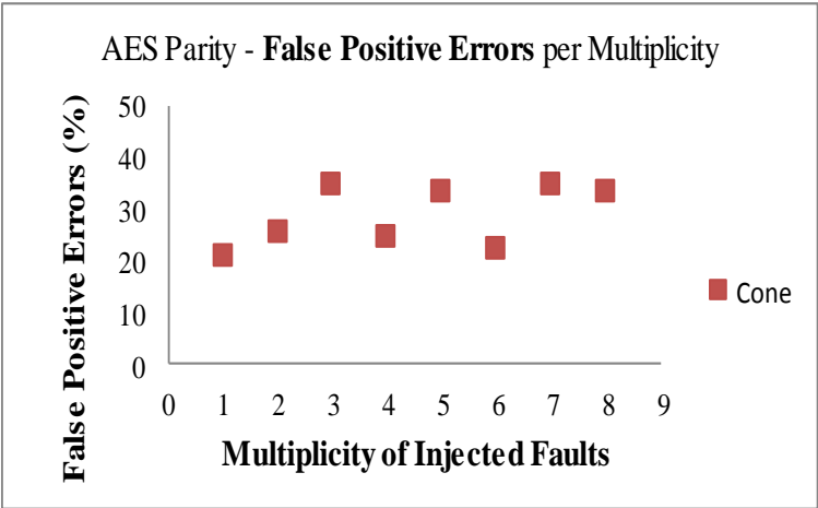
Figure 3.16: AES Parity, false positive error percentages per multiplicity
