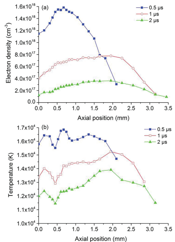
FIG. 4. Axial profiles of (a) electron density and (b) temperature determined for different delays of 0.5, 1.0, and 2.0 \mu\text{s} . We estimate the relative standard deviations of the electron density and the temperature to be 15% and 10%, respectively.
