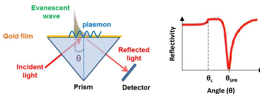
Figure 1.2.8: Schematic diagram of the principles of SPR. Image adapted from ref [215].
