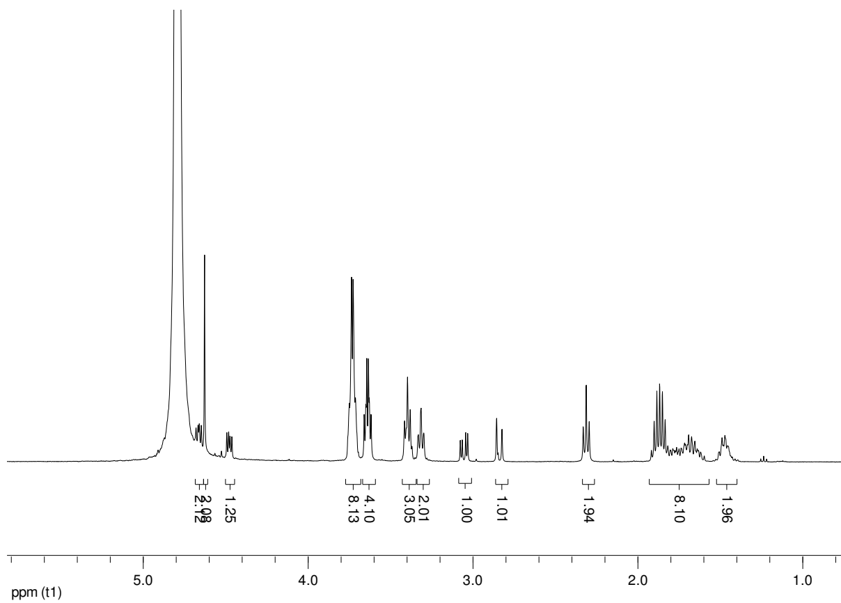
Figure Syn3. ^1\text{H} NMR spectrum (400 MHz, \text{D}_2\text{O} ) of compound 5.
