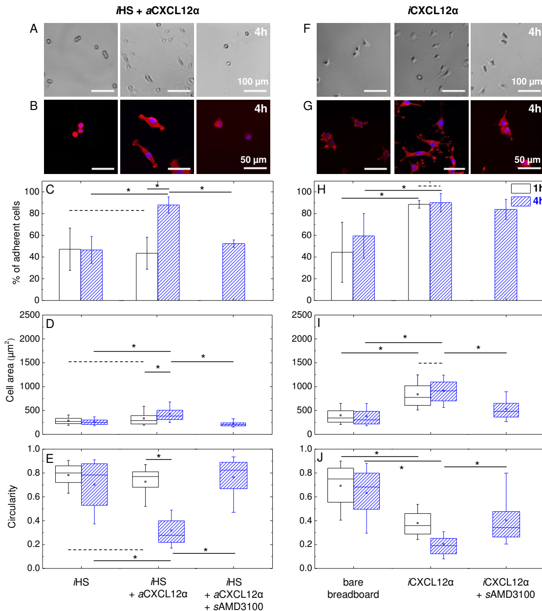
Figure 2. Effect of matrix-bound CXCL12 \alpha presentation on C2C12 myoblast adhesion, spreading and circularity. A to E: adsorbed CXCL12 \alpha ; F to J: immobilized CXCL12 \alpha . Bright-field images of live cells (A and F) and representative fluorescence staining of fixed cells (cell nuclei labeled in blue and actin in red; B and G) for C2C12 myoblasts exposed to surfaces presenting different surface functionalizations for 4 h. (C and H) Quantitative analysis of the percentage of adherent cells that remain after gentle rinsing following 1 h (black) and 4 h (blue, hatched) of exposure to different surface functionalizations. The area (D and I) and circularity (E and J) of the adhered cells are displayed as box plots; the small square and the horizontal line inside the box indicate the mean and the median, respectively, the box delimits the 25% to 75% percentile of data, and the error bar represents the lower 10% limit and the upper 90% limit. An ANNOVA test was performed to obtain p-values (lines with an asterisk indicate p < 0.05 ; dotted lines indicate no significant difference).
