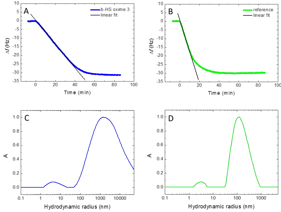
Figure S5. Quantification of active analyte concentrations from QCM-D binding assays. (A-B) QCM-D responses ( \Delta f ) for the adsorption of 3 (freshly defrozed and incubated at 1 \mu\text{g/mL} total HS concentration; A) and a biotinylated oligonucleotide (incubated at c_{\text{ref}} = 1.56 \mu\text{g/mL} ; B) to a SAV monolayer. The oligonucleotide served as reference molecule to determine the concentration of intact b-HS, c_{\text{b-HS}} , in the HS solution, as described in the following. Binding of an analyte (b-HS in our case) to a ligand (SAV) on the QCM-D sensor surface is a two-step event, consisting of mass transfer to the sensor surface followed by the actual binding to the ligand. Since the biotin-SAV bond forms rapidly, the first step is rate limiting in our assay, except at high coverage where the scarcity of available binding sites limits binding. For mass-transfer limited binding, the binding rate depends exclusively on the flow conditions (i.e. flow-cell geometry and flow rate, maintained constant in our assay) and the analyte's active concentration (i.e. the concentration of HS being effectively biotin-conjugated, c_{\text{b-HS}} ) and diffusion coefficient, D_{\text{b-HS}} . 7 Considering the flow conditions in our experimental setup (i.e. laminar flow in a slit), the binding rate is given by
