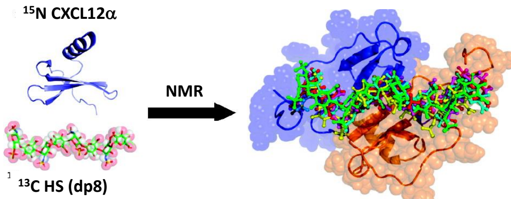
Figure I.1.13: Structure of CXCL12 \alpha dimer (ribbon structure) induced by ^{13}\text{C} labelled octasaccharide. Image taken from ref [120].
