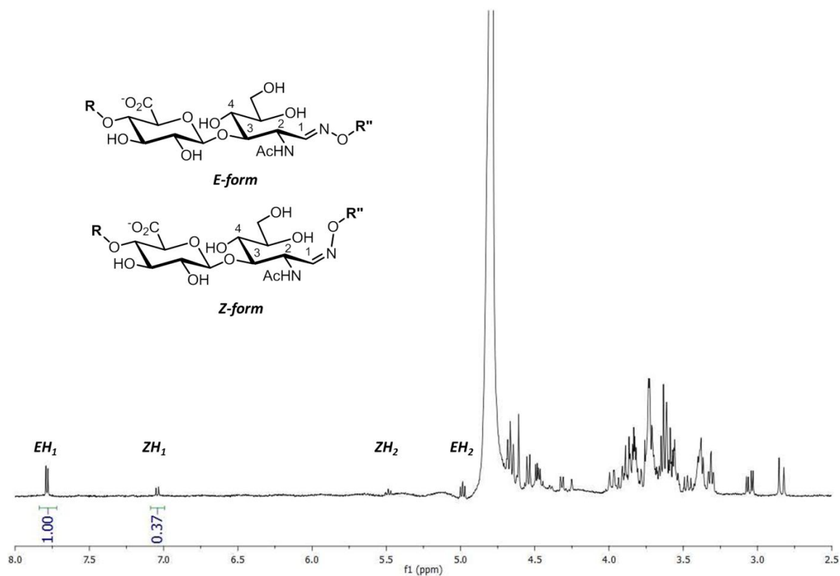
Figure S2. NMR analysis of b-HA_dp4 10 . The 1 NMR analysis shows the formation of E and Z conformations of 10 , indicating that the attachment of biotin occurs at the reducing end of HA which leads to both the open and closed forms. Integrating the signals corresponding to the two conformations, the oxime link was found to be 73% and 27% in E and Z conformation, respectively. R is a GlcA β(1→3) GlcNAc β(1→4) disaccharide, and R'' is defined in Scheme 1.
