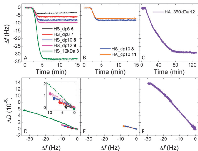
Fig. 3 QCM-D binding assays for HS (A) and HA (B, C) of various sizes (as indicated). All GAGs were conjugated with biotin via oxime ligation. Data for 8 are also shown in (B) to facilitate comparison with 11 . Incubation conditions were as described in Fig. 1, except for 12 , which was incubated from 5 to 110 min. (D–F) \Delta D vs. \Delta f curves corresponding to (A–C), respectively; the inset in (D) shows a part of the data at a higher magnification. The magnitude of the slope of the \Delta D vs. \Delta f curves increases as a function of GAG size, indicating that larger GAGs generate a softer film. 21
